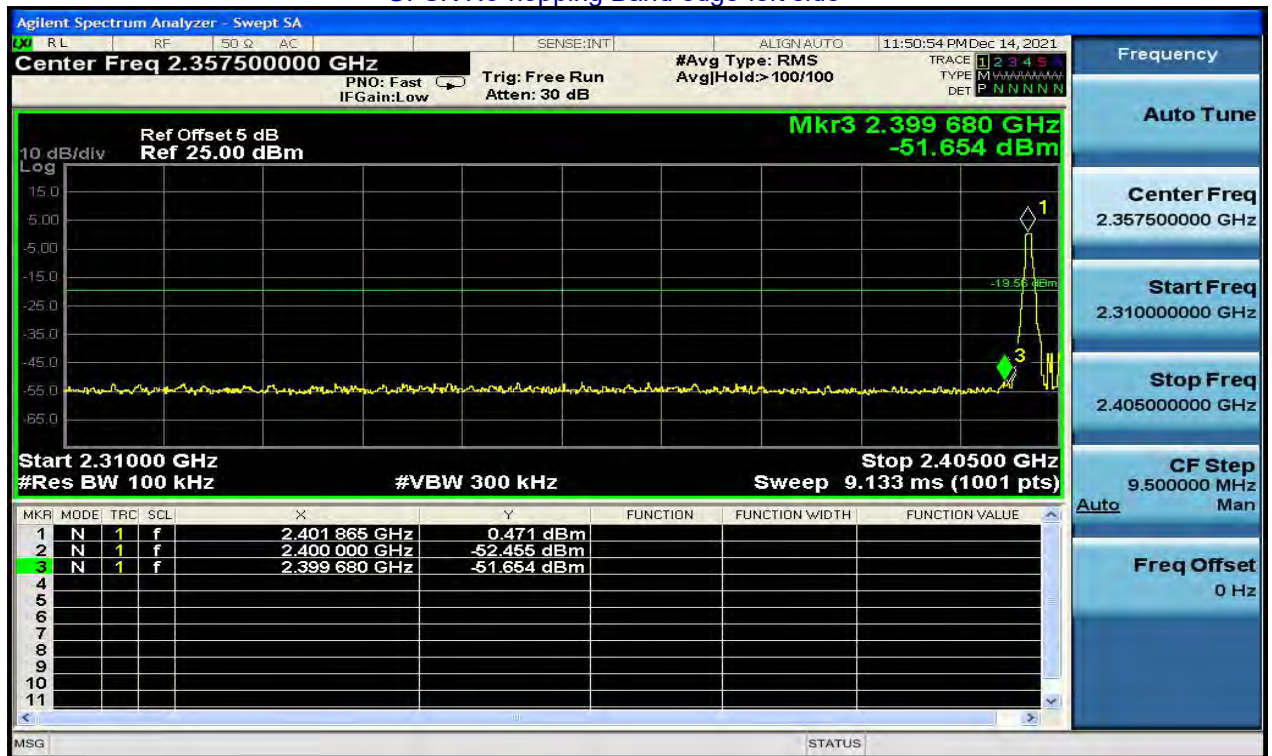
GFSK No-hopping Band edge-left side
