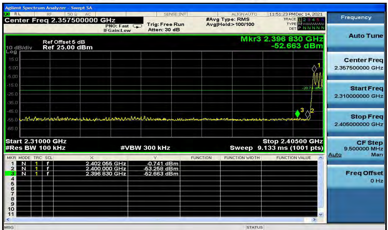
GFSK Hopping Band edge-left side
