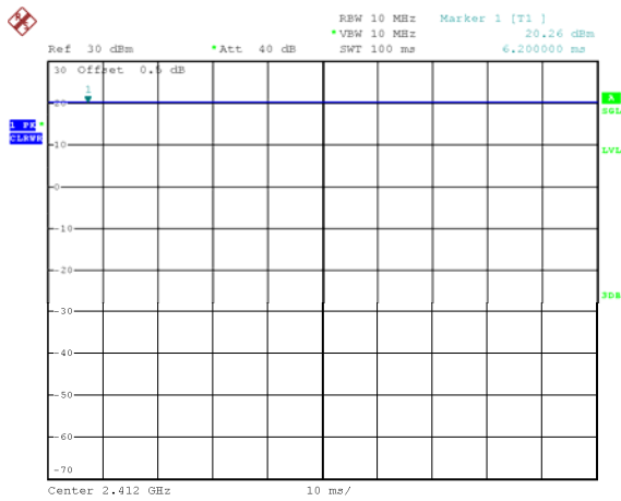
Wi-Fi 802.11g
