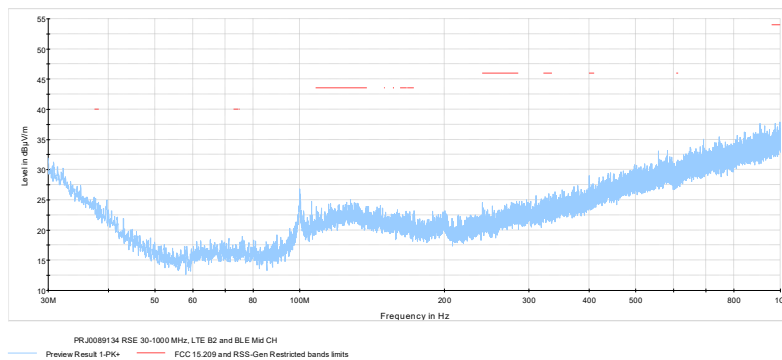
Figure 7.1-4: Radiated spurious emissions 30 – 1000 MHz, LTE Band 2 and BLE mid channel
