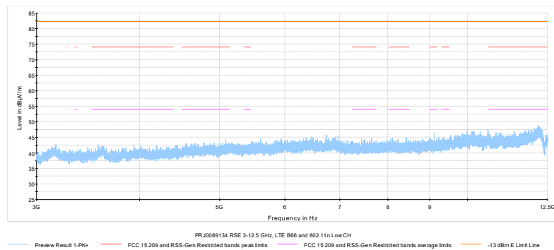
Figure 7.1-12: Spot checking, Radiated spurious emissions 3 – 12.5 GHz, LTE Band 66 and WiFi low channel
