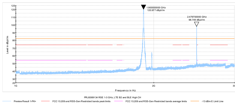
Figure 7.1-8: Radiated spurious emissions 1 – 3 GHz, LTE Band 2 and BLE high channel
