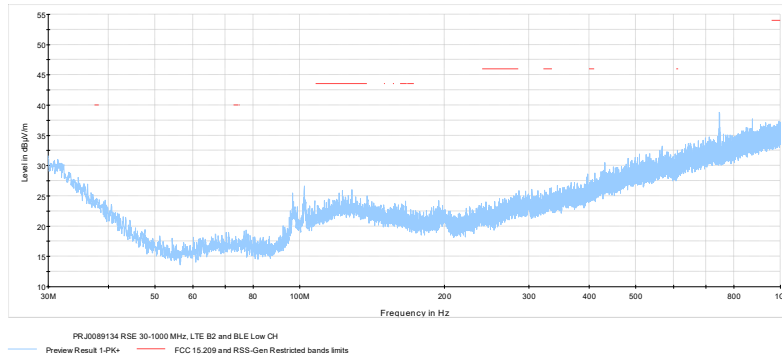
Figure 7.1-1: Radiated spurious emissions 30 – 1000 MHz, LTE Band 2 and BLE low channel
