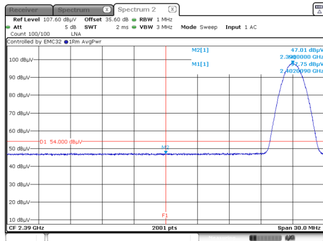
Figure 7.1-20: Restricted band edge spurious emissions at 2390 MHz, BLE, Average
