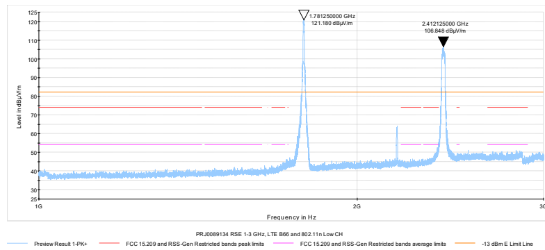
Figure 7.1-11: Spot checking, Radiated spurious emissions 1 – 3 GHz, LTE Band 66 and WiFi low channel
