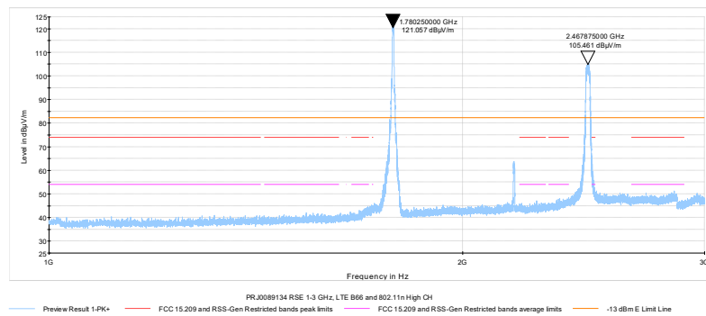
Figure 7.1-17: Spot checking, Radiated spurious emissions 1 – 3 GHz, LTE Band 66 and WiFi high channel
