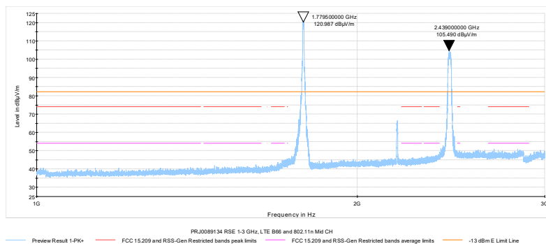
Figure 7.1-14: Spot checking, Radiated spurious emissions 1 – 3 GHz, LTE Band 66 and WiFi mid channel
