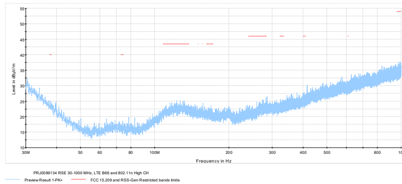
Figure 7.1-16: Spot checking, Radiated spurious emissions 30 – 1000 MHz, LTE Band 66 and WiFi high channel
