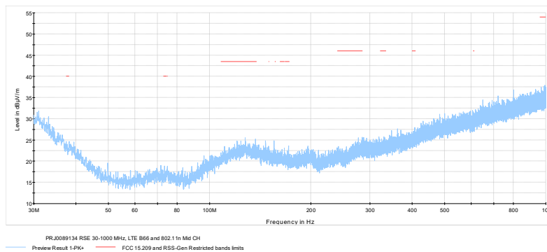
Figure 7.1-13: Spot checking, Radiated spurious emissions 30 – 1000 MHz, LTE Band 66 and WiFi mid channel
