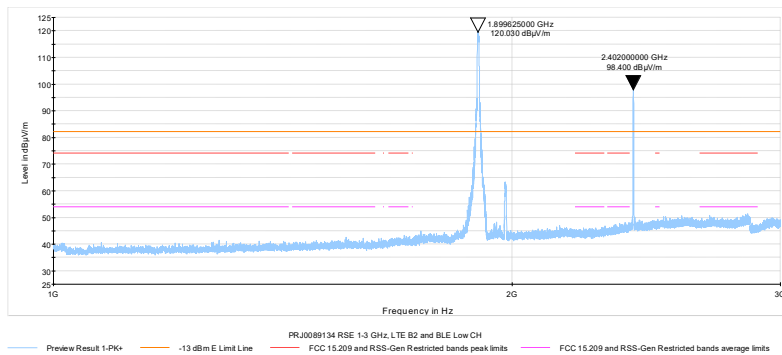
Figure 7.1-2: Radiated spurious emissions 1 – 3 GHz, LTE Band 2 and BLE low channel
