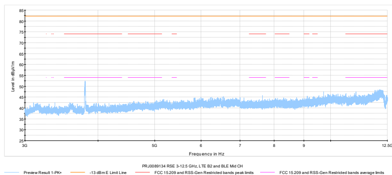
Figure 7.1-6: Radiated spurious emissions 3 – 12.5 GHz, LTE Band 2 and BLE mid channel
