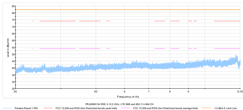
Figure 7.1-15: Spot checking, Radiated spurious emissions 3 – 12.5 GHz, LTE Band 66 and WiFi mid channel
