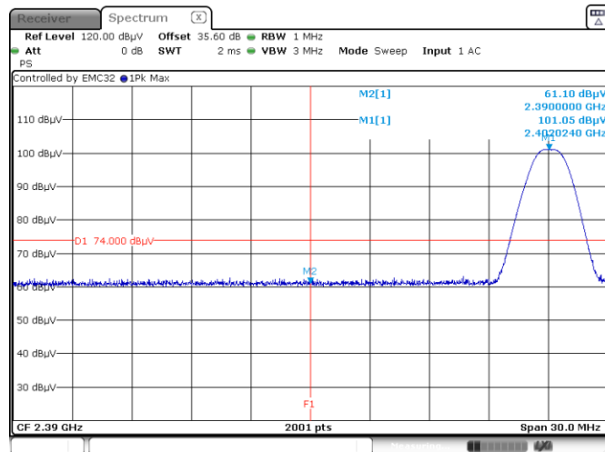
Figure 7.1-19: Restricted band edge spurious emissions at 2390 MHz, BLE, Peak
