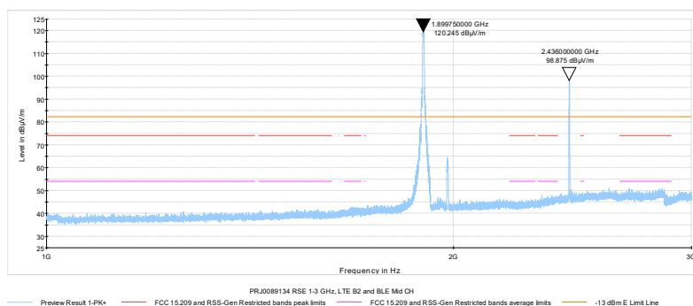
Figure 7.1-5: Radiated spurious emissions 1 – 3 GHz, LTE Band 2 and BLE mid channel
