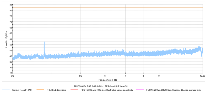
Figure 7.1-3: Radiated spurious emissions 3 – 12.5 GHz, LTE Band 2 and BLE low channel
