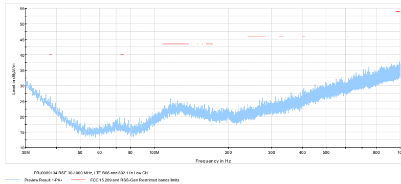
Figure 7.1-10: Spot checking, Radiated spurious emissions 30 – 1000 MHz, LTE Band 66 and WiFi low channel
