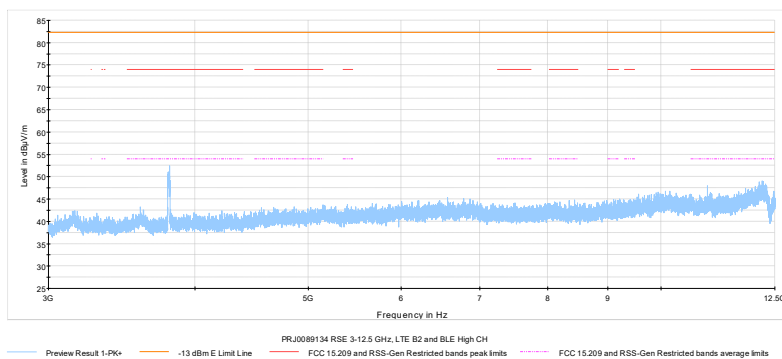
Figure 7.1-9: Radiated spurious emissions 3 – 12.5 GHz, LTE Band 2 and BLE high channel
