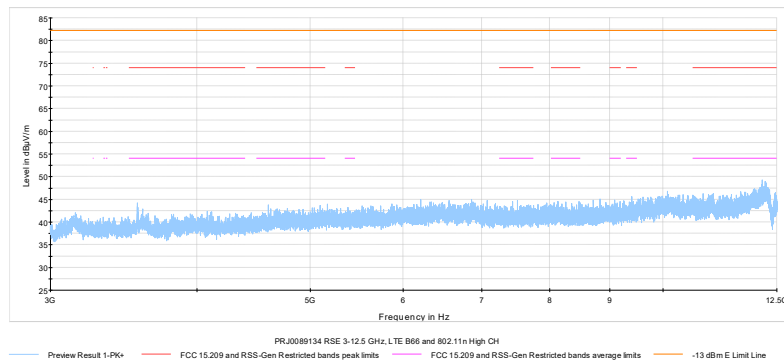
Figure 7.1-18: Spot checking, Radiated spurious emissions 3 – 12.5 GHz, LTE Band 66 and WiFi high channel
