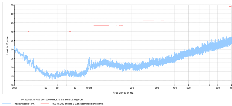
Figure 7.1-7: Radiated spurious emissions 30 – 1000 MHz, LTE Band 2 and BLE high channel
