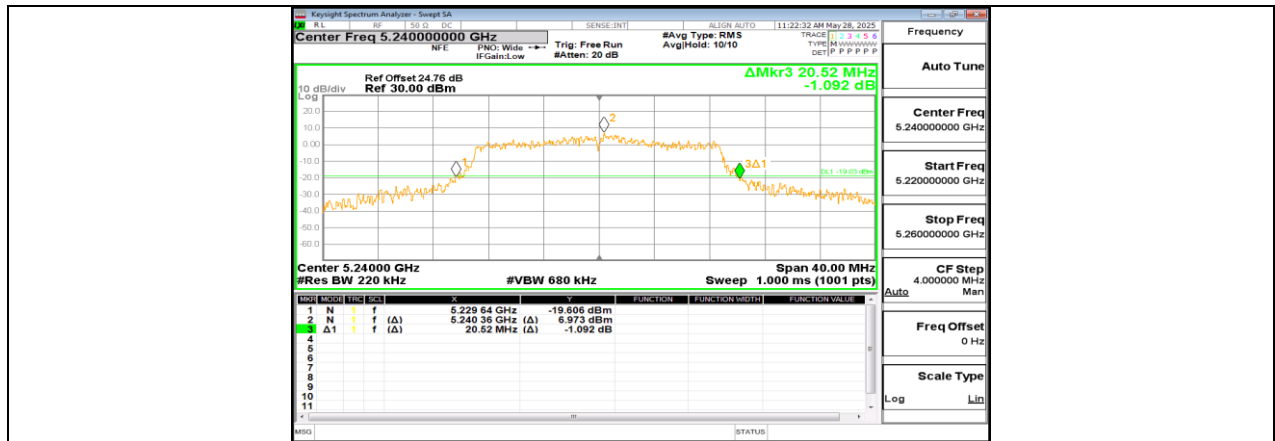
11N20SISO_Ant1_5240
