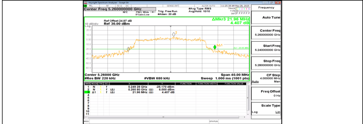
11N20SISO_Ant1_5260
