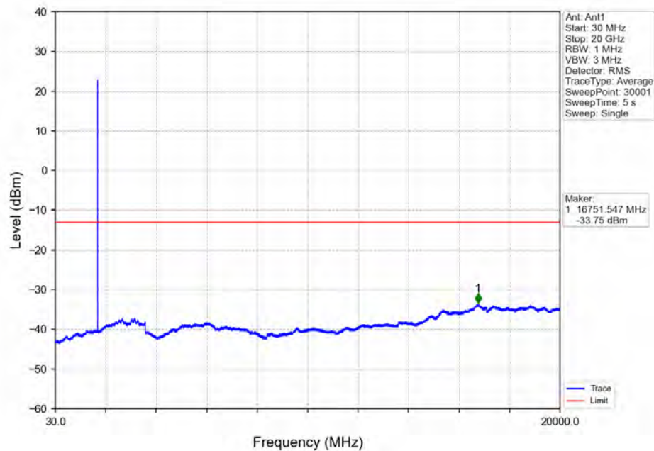
Band4_1.4MHz_QPSK_LCH_1710.7MHz_RB_6_0_NTNV
