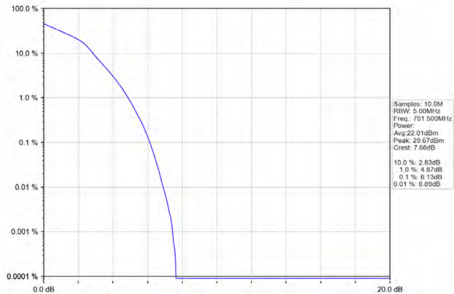
Band12_5MHz_16QAM_LCH_701.5MHz_RB_25_0_NTNV
