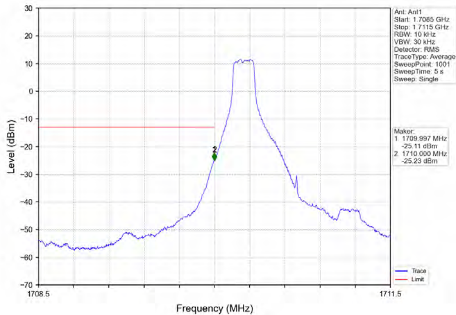
Band4_1.4MHz_QPSK_LCH_1710.7MHz_RB_1_0_NTNV
