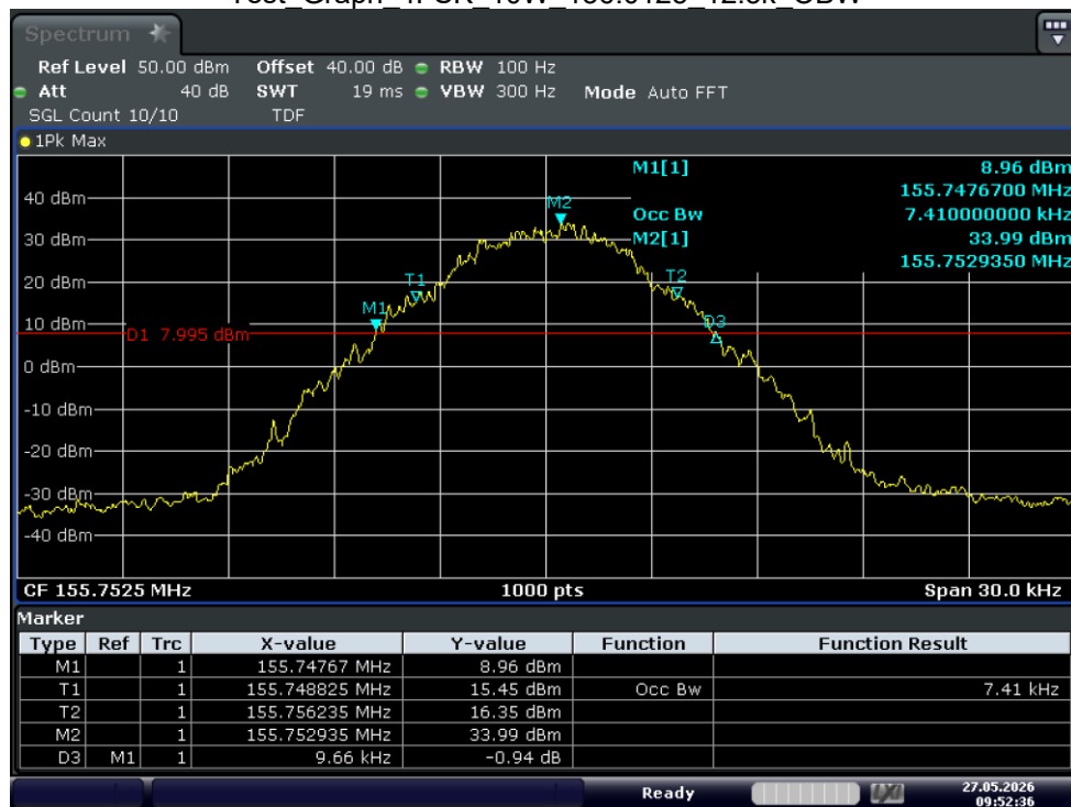
Test_Graph_4FSK_10W_155.7525_12.5k_OBW
