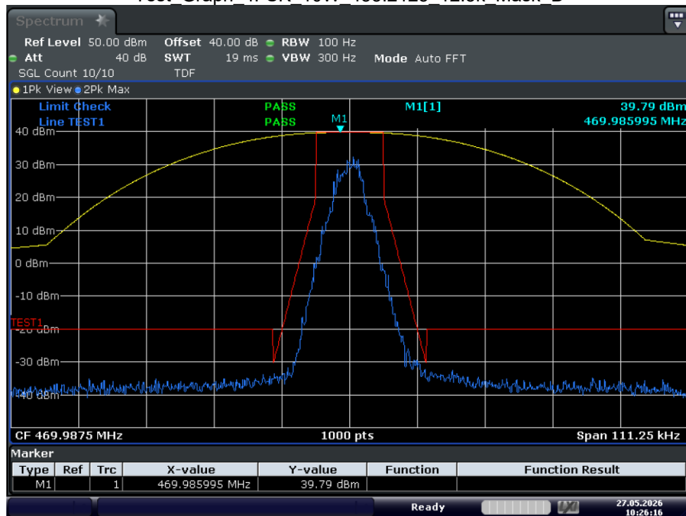
Test_Graph_4FSK_10W_469.9875_12.5k_Mask_D
