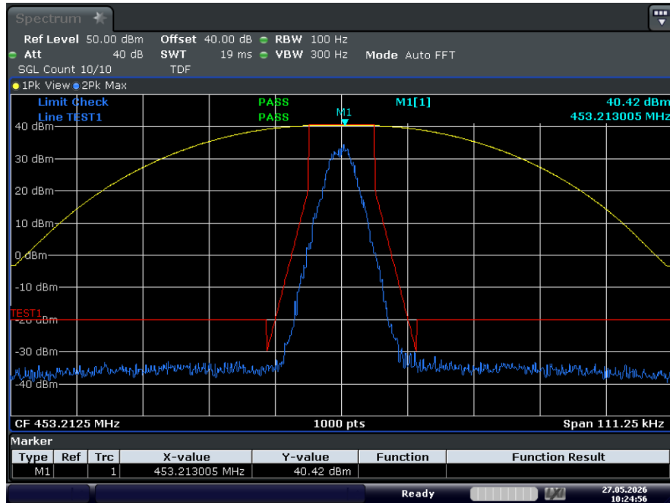
Test Graph 4FSK 10W 453.2125 12.5k Mask D
