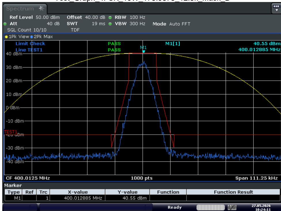
Test_Graph_4FSK_10W_400.0125_12.5k_Mask_D
