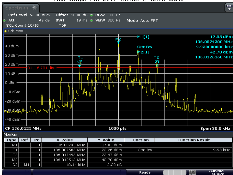
Test_Graph_FM_25W_136.0125_12.5k_OBW
