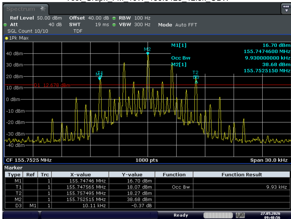
Test_Graph_FM_10W_155.7525_12.5k_OBW
