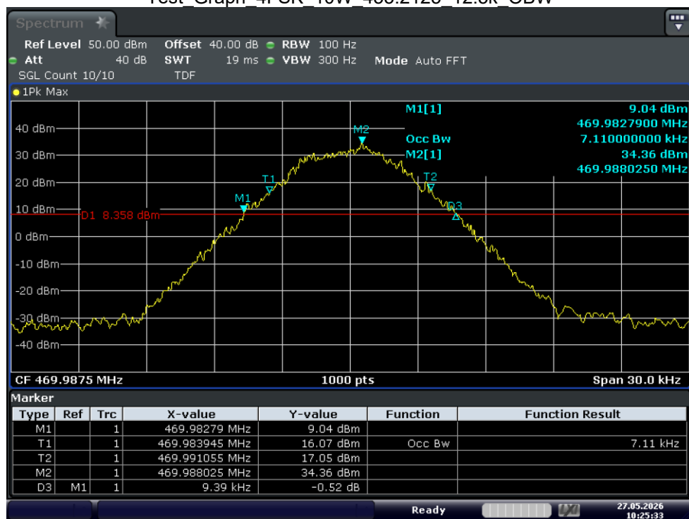
Test_Graph_4FSK_10W_469.9875_12.5k_OBW
