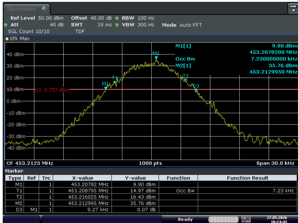
Test Graph 4FSK 10W 453.2125 12.5k OBW
