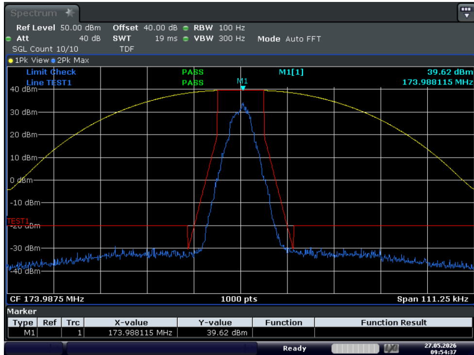
Test Graph 4FSK 10W 173.9875 12.5k Mask D
