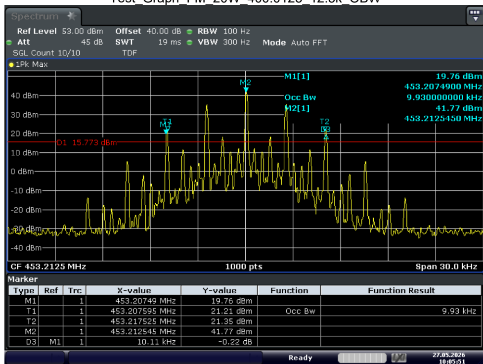
Test_Graph_FM_20W_453.2125_12.5k_OBW
