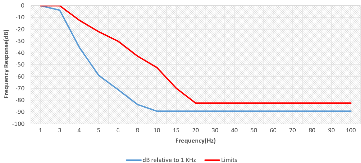
Audio Low Pass Filter Frequency Response
