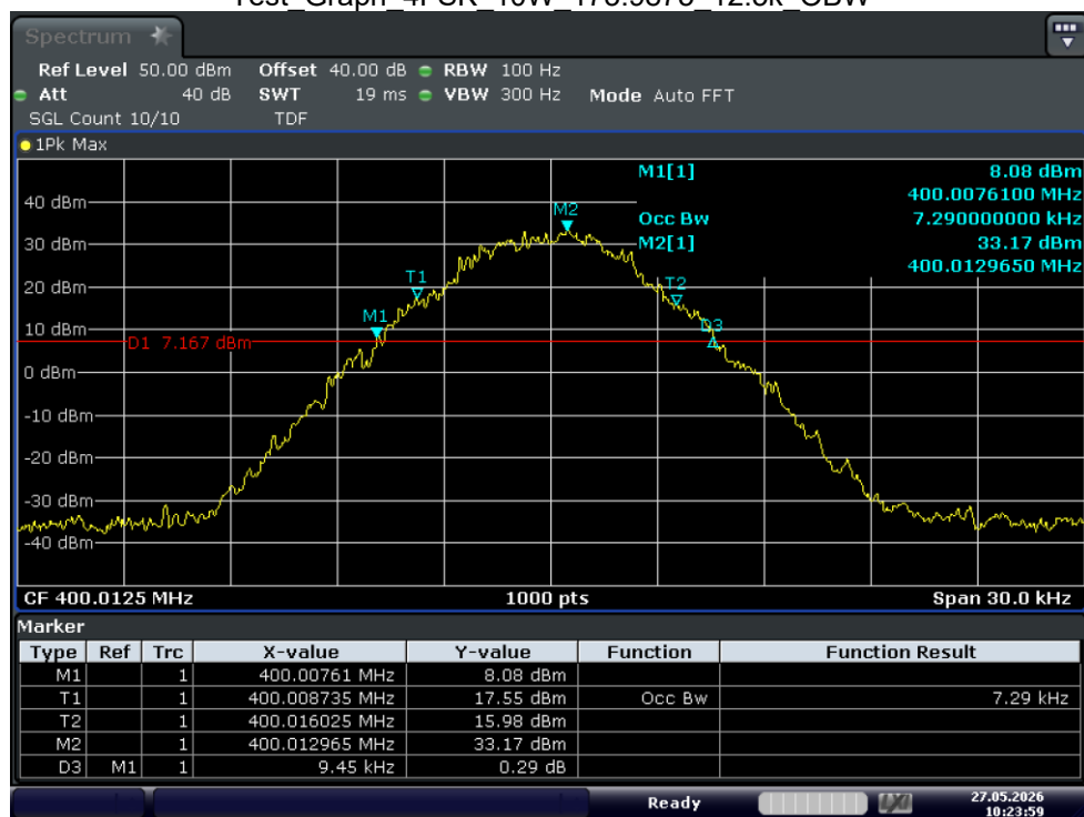
Test_Graph_4FSK_10W_400.0125_12.5k_OBW
