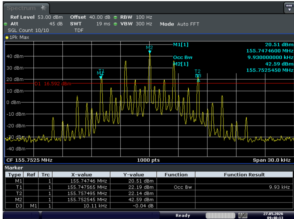
Test Graph FM 25W 155.7525 12.5k OBW
