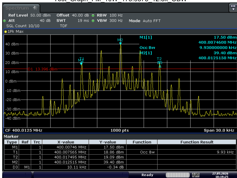
Test_Graph_FM_10W_400.0125_12.5k_OBW
