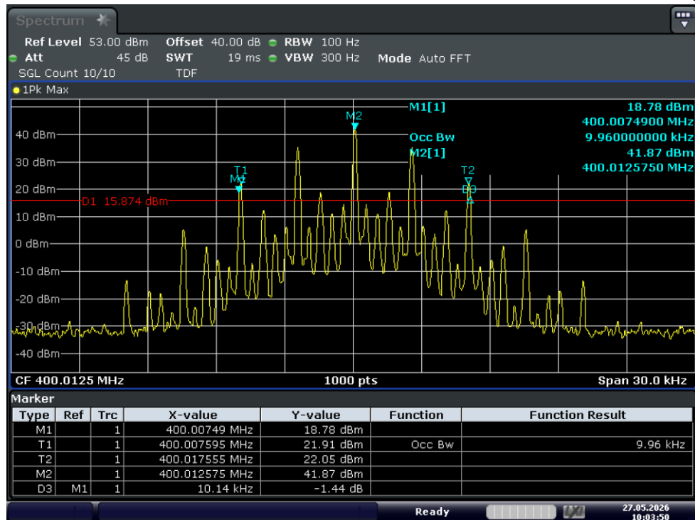
Test Graph FM 20W 400.0125 12.5k OBW
