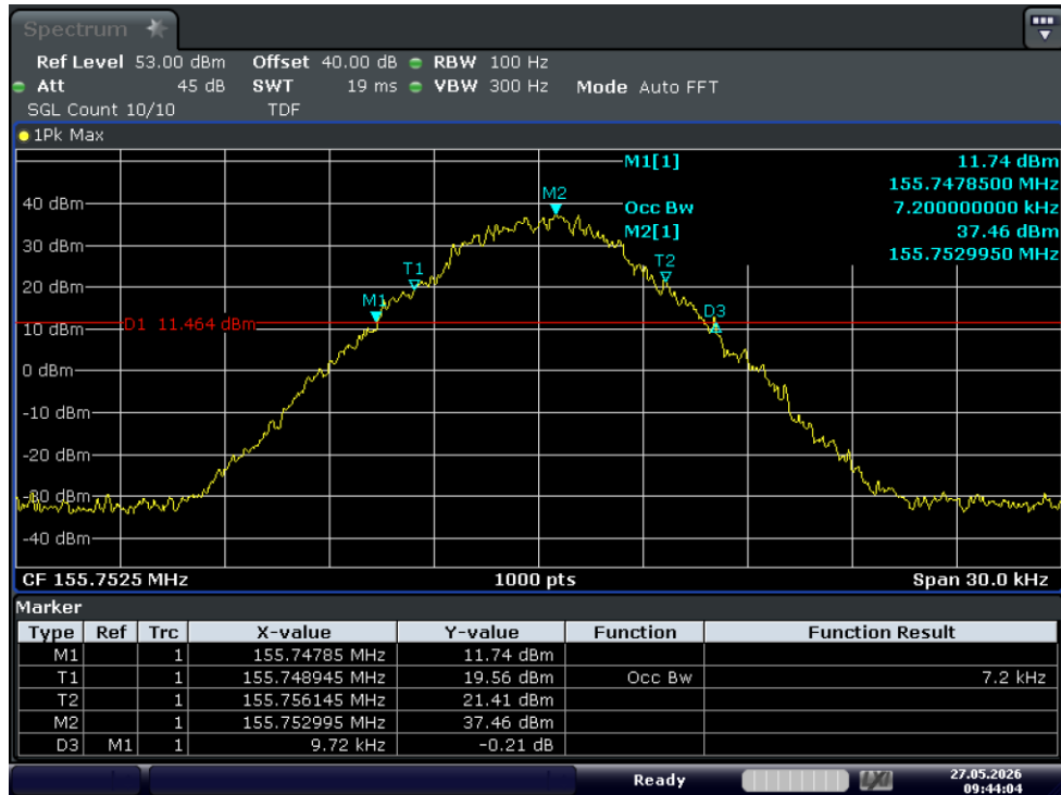
Test Graph 4FSK 25W 155.7525 12.5k OBW
