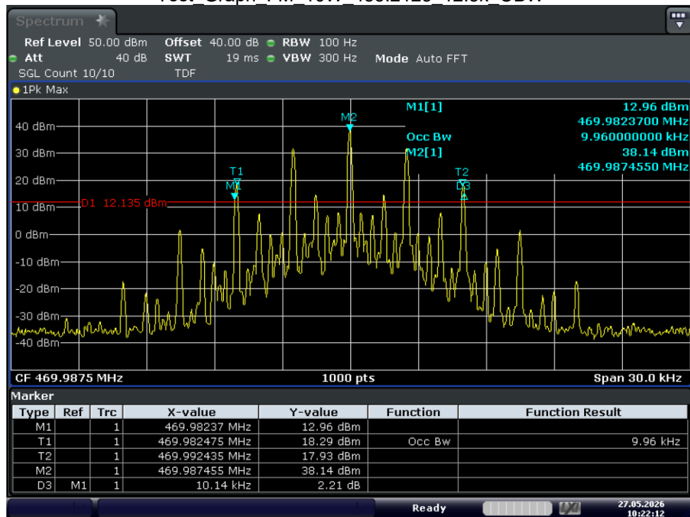
Test_Graph_FM_10W_469.9875_12.5k_OBW
