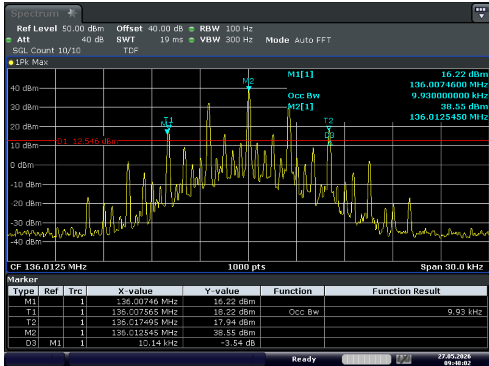
Test Graph FM 10W 136.0125 12.5k OBW
