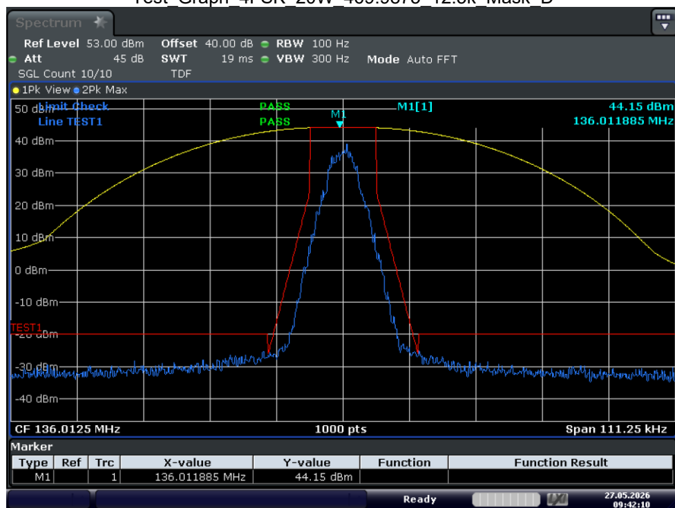
Test_Graph_4FSK_25W_136.0125_12.5k_Mask_D
