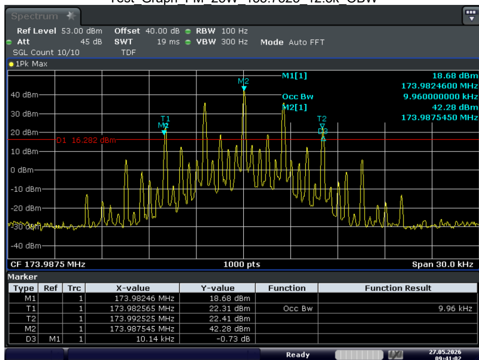
Test_Graph_FM_25W_173.9875_12.5k_OBW
