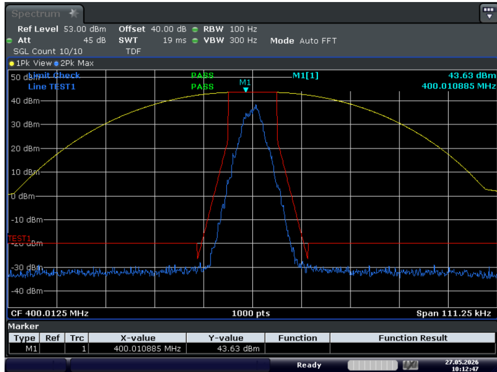
Test Graph 4FSK 20W 400.0125 12.5k Mask D
