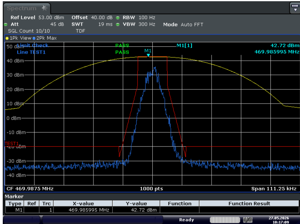
Test Graph 4FSK 20W 469.9875 12.5k Mask D
