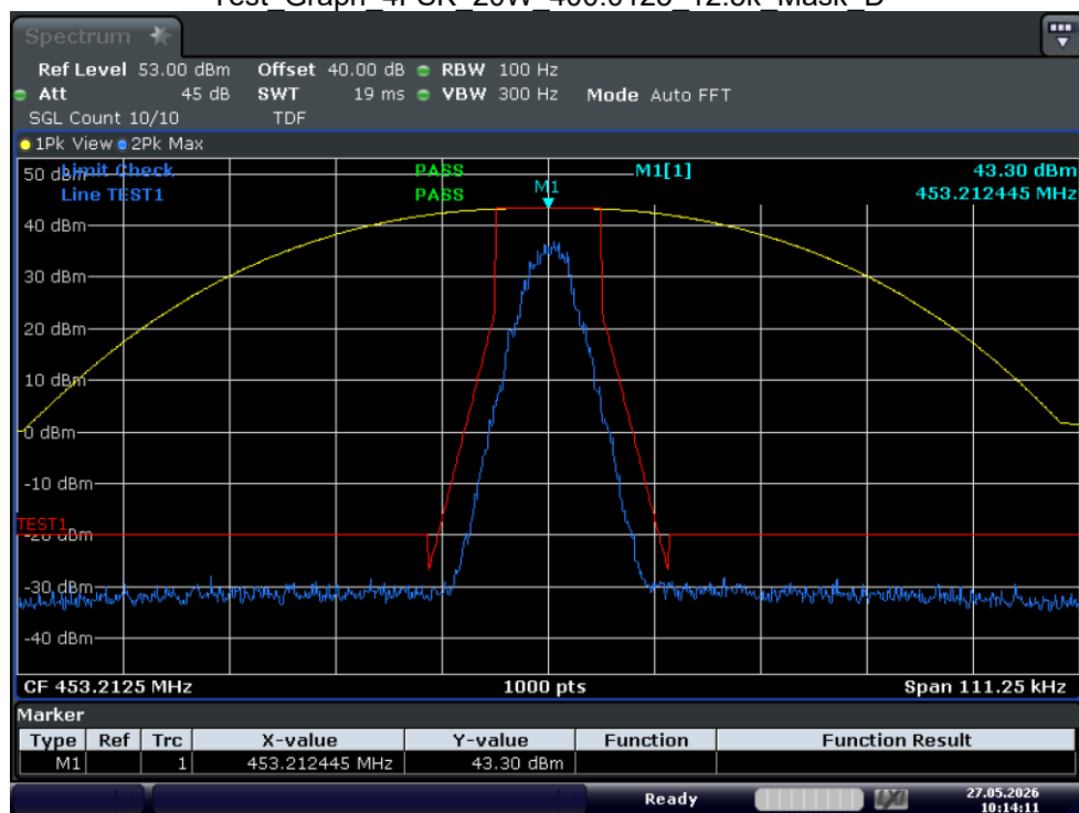
Test_Graph_4FSK_20W_453.2125_12.5k_Mask_D
