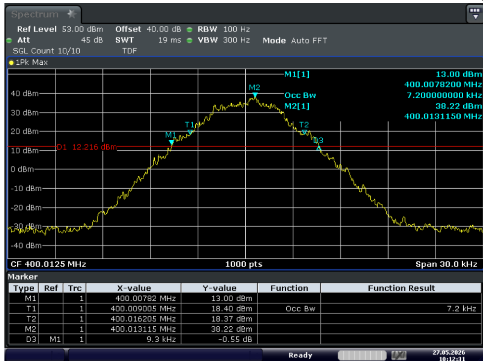
Test Graph 4FSK 20W 400.0125 12.5k OBW
