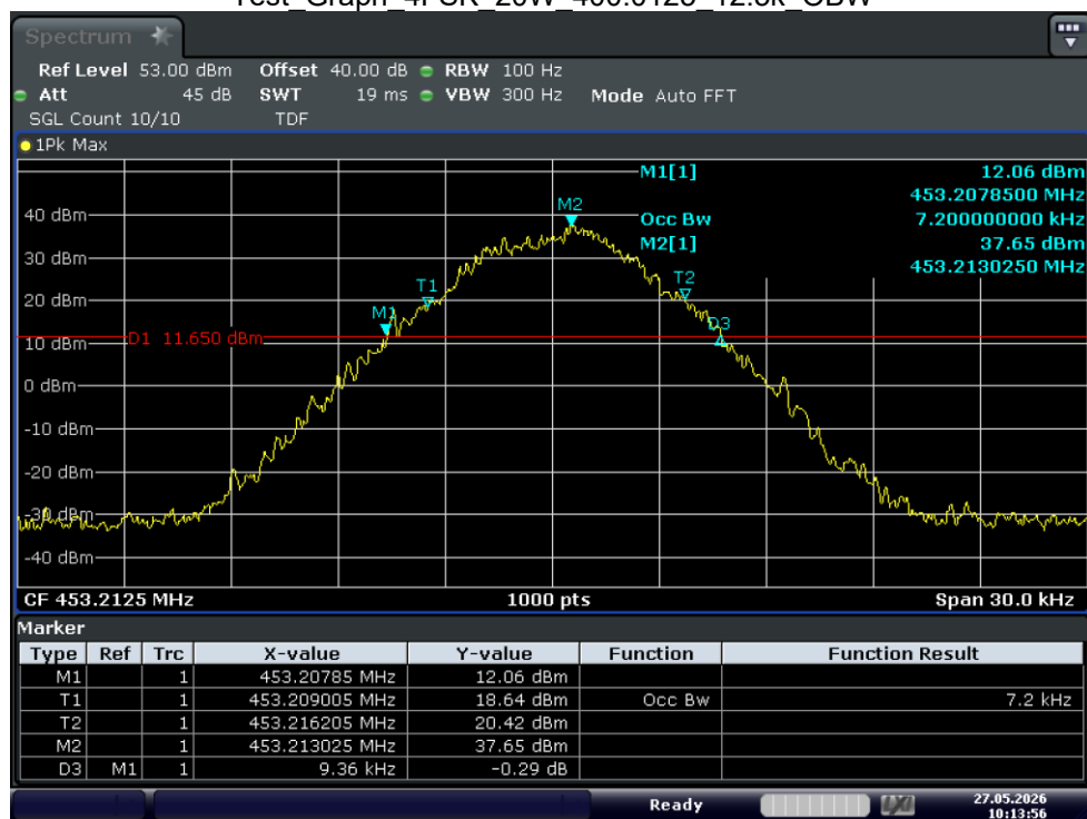
Test_Graph_4FSK_20W_453.2125_12.5k_OBW
