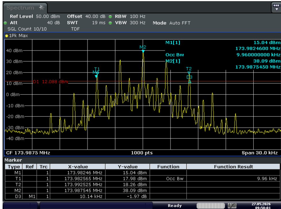
Test Graph FM 10W 173.9875 12.5k OBW
