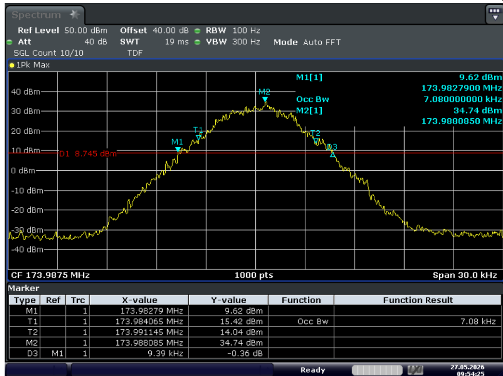
Test Graph 4FSK 10W 173.9875 12.5k OBW
