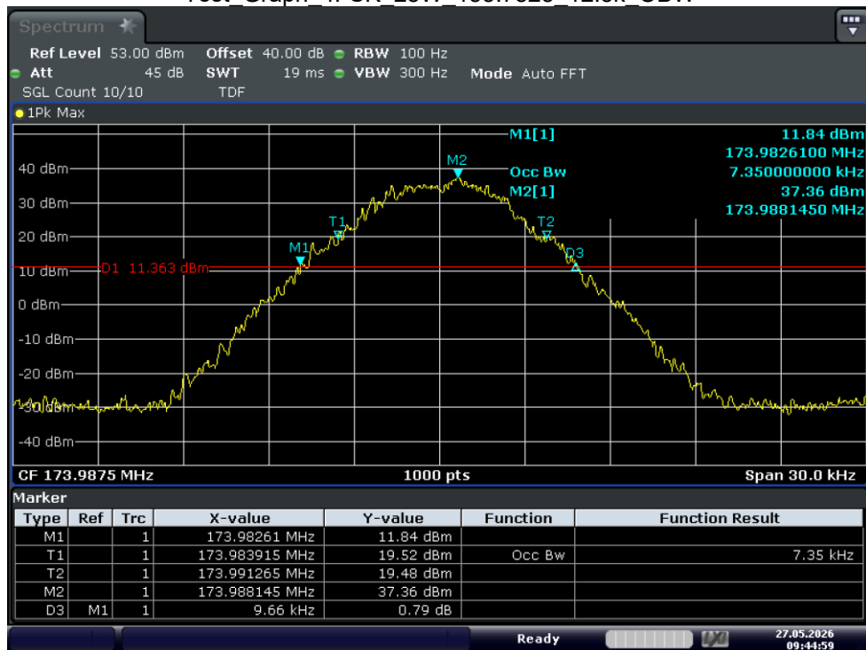
Test_Graph_4FSK_25W_173.9875_12.5k_OBW
