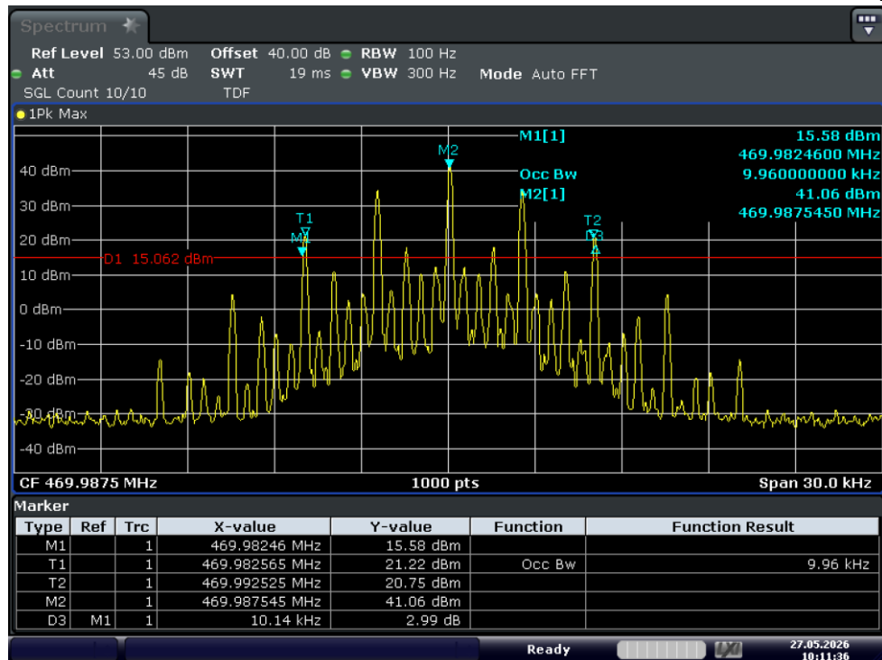
Test Graph FM 20W 469.9875 12.5k OBW
