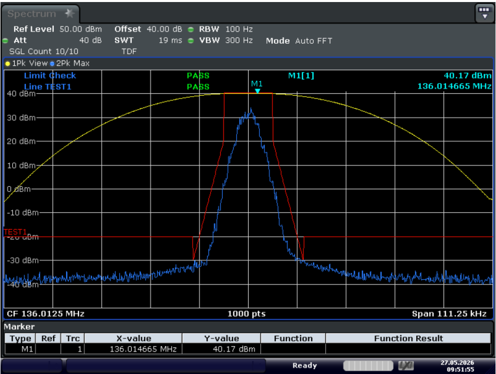
Test Graph 4FSK 10W 136.0125 12.5k Mask D
