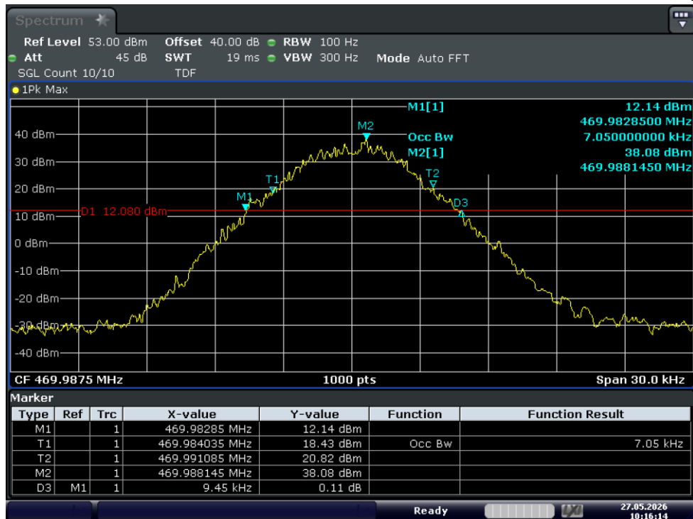
Test Graph 4FSK 20W 469.9875 12.5k OBW
