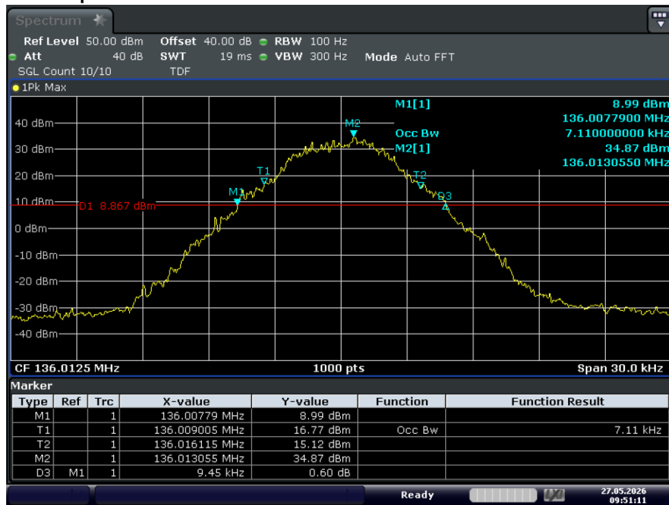
Test Graph 4FSK 10W 136.0125 12.5k OBW
