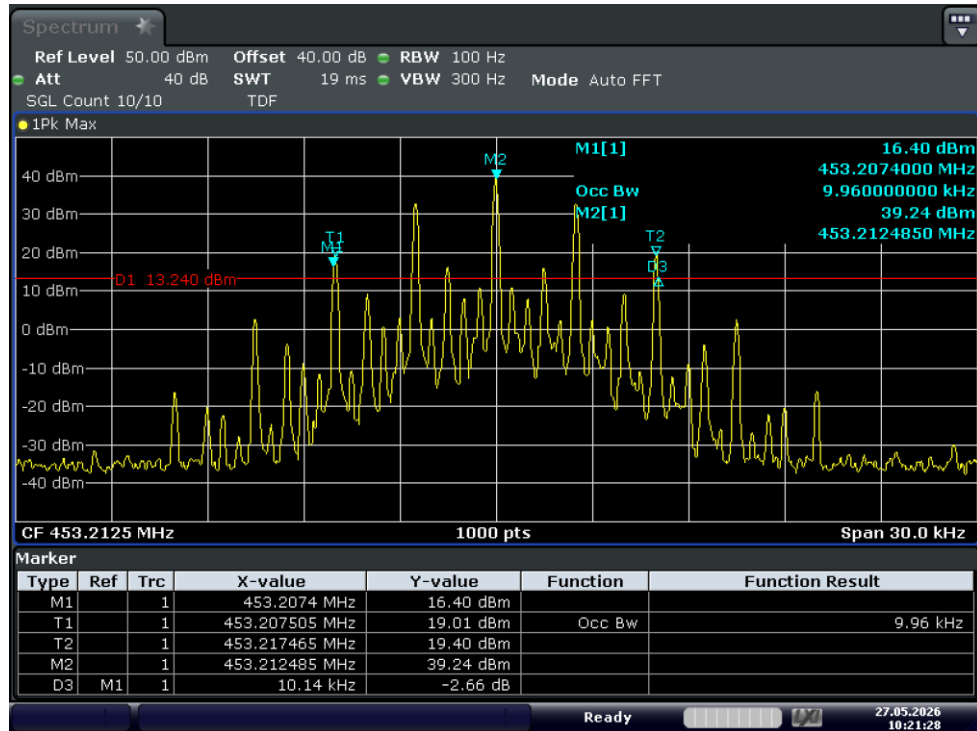
Test Graph FM 10W 453.2125 12.5k OBW
