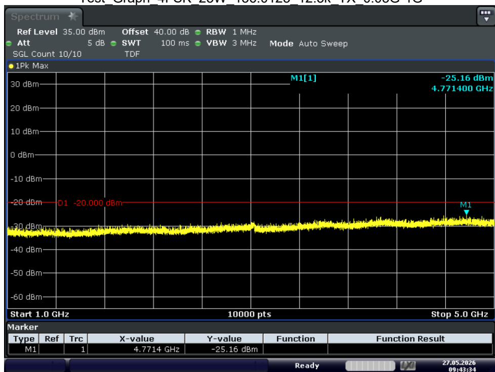
Test_Graph_4FSK_25W_136.0125_12.5k_TX_1G-5G
