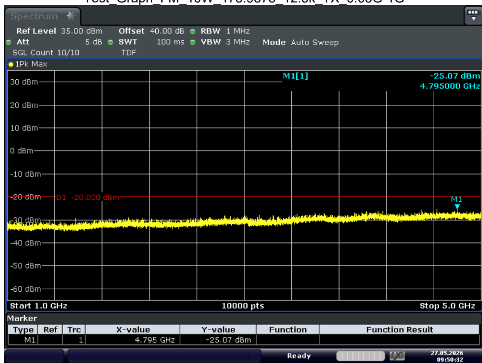
Test_Graph_FM_10W_173.9875_12.5k_TX_1G-5G
