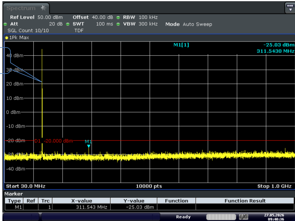
Test Graph FM 25W 155.7525 12.5k TX 0.03G-1G
