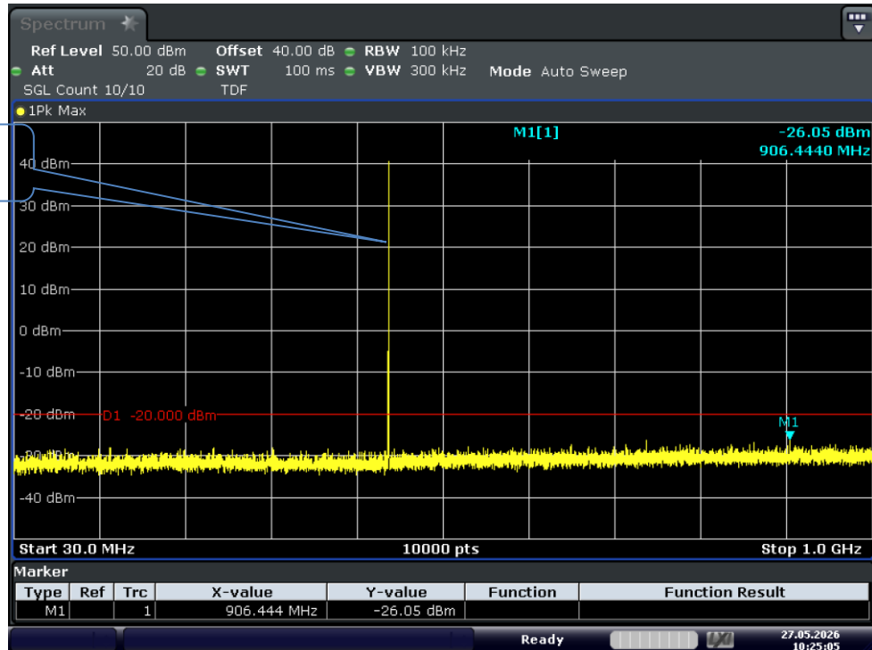
Test Graph 4FSK 10W 453.2125 12.5k TX 0.03G-1G
