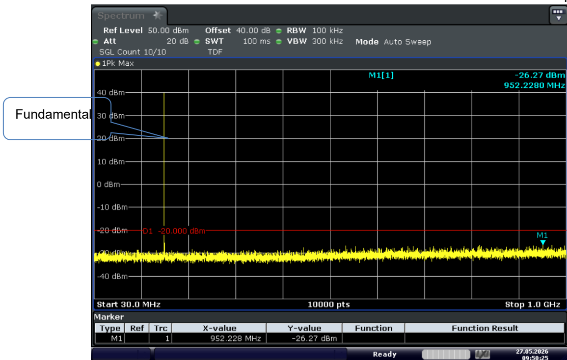
Test Graph FM 10W 173.9875 12.5k TX 0.03G-1G
