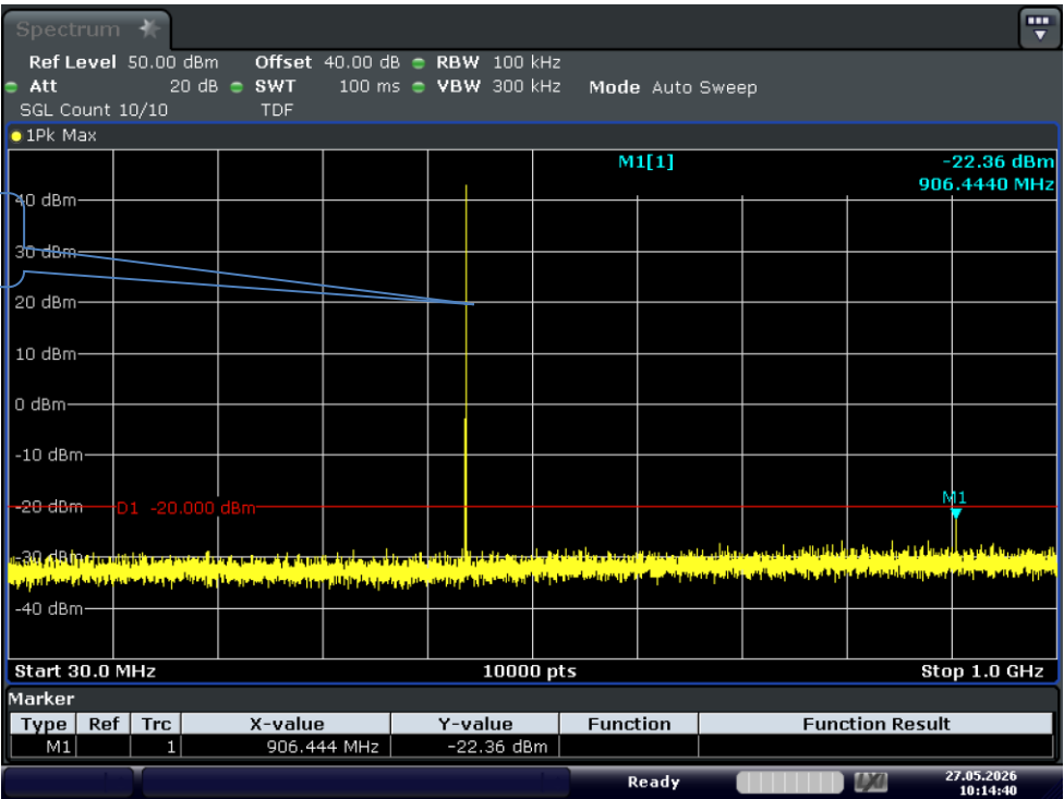
Test Graph 4FSK 20W 453.2125 12.5k TX 0.03G-1G
