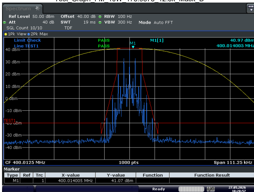
Test_Graph_FM_10W_400.0125_12.5k_Mask_D
