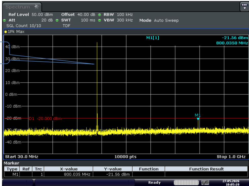
Test Graph FM 20W 400.0125 12.5k TX 0.03G-1G
