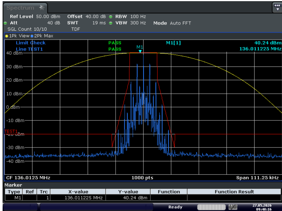
Test Graph FM 10W 136.0125 12.5k Mask D
