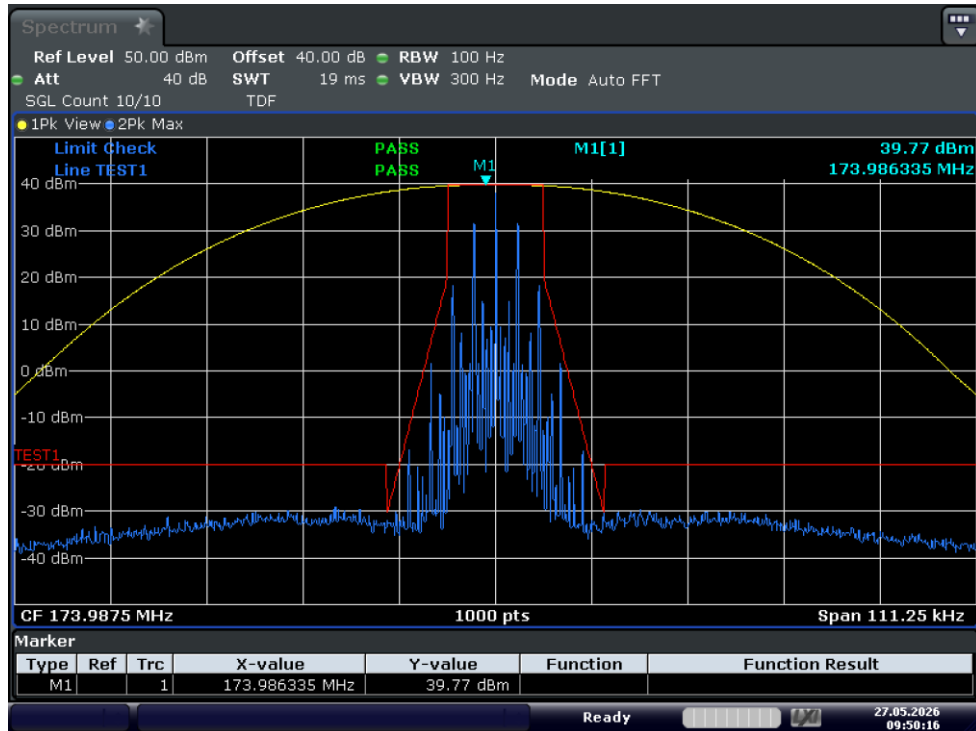
Test Graph FM 10W 173.9875 12.5k Mask D
