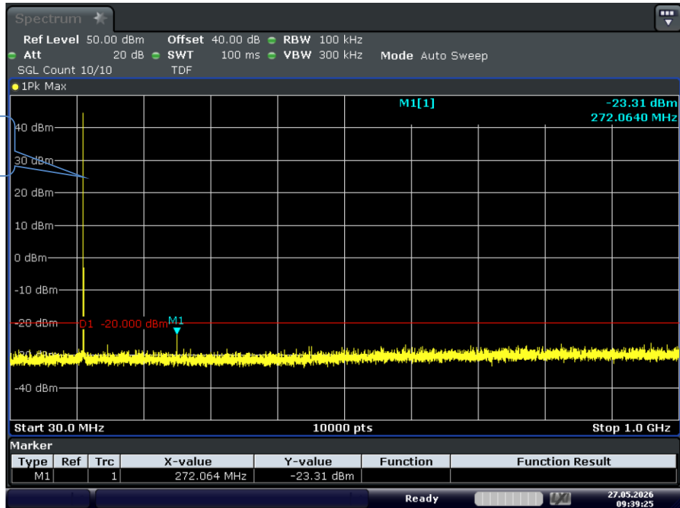
Test Graph FM 25W 136.0125 12.5k TX 0.03G-1G
