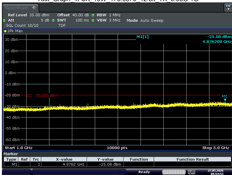
Test_Graph_4FSK_10W_173.9875_12.5k_TX_1G-5G
