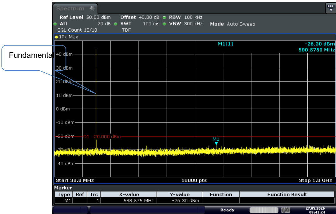
Test Graph FM 25W 173.9875 12.5k TX 0.03G-1G
