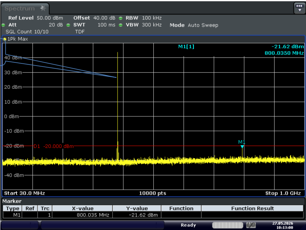
Test Graph 4FSK 20W 400.0125 12.5k TX 0.03G-1G
