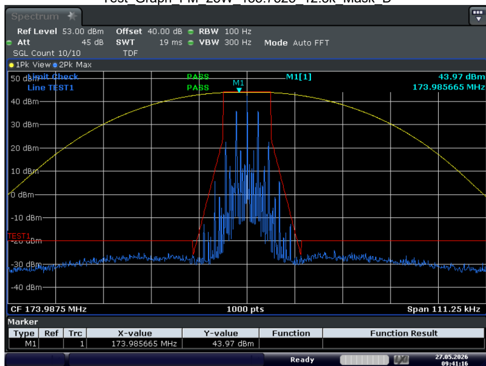
Test_Graph_FM_25W_173.9875_12.5k_Mask_D
