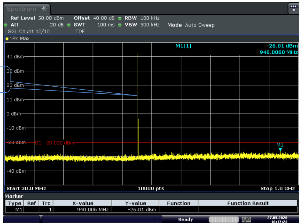
Test Graph 4FSK 20W 469.9875 12.5k TX 0.03G-1G
