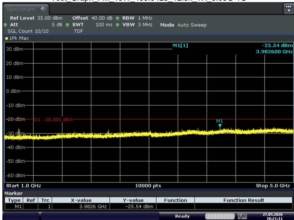
Test_Graph_FM_10W_400.0125_12.5k_TX_1G-5G
