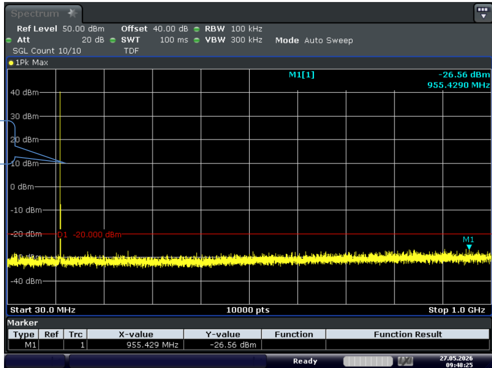
Test Graph FM 10W 136.0125 12.5k TX 0.03G-1G
