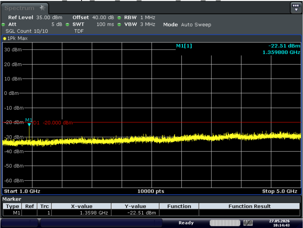
Test_Graph_4FSK_20W_453.2125_12.5k_TX_1G-5G
