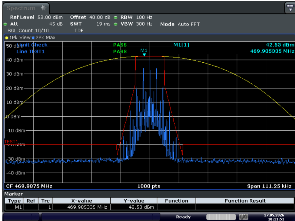
Test Graph FM 20W 469.9875 12.5k Mask D
