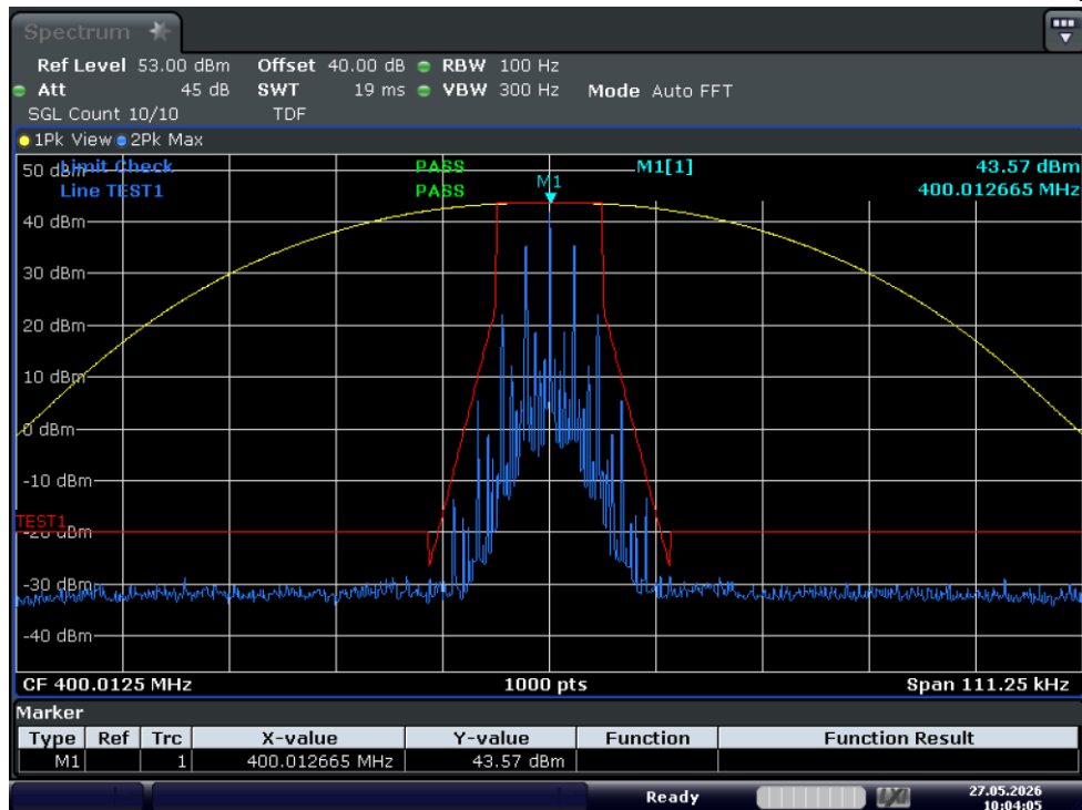
Test Graph FM 20W 400.0125 12.5k Mask D
