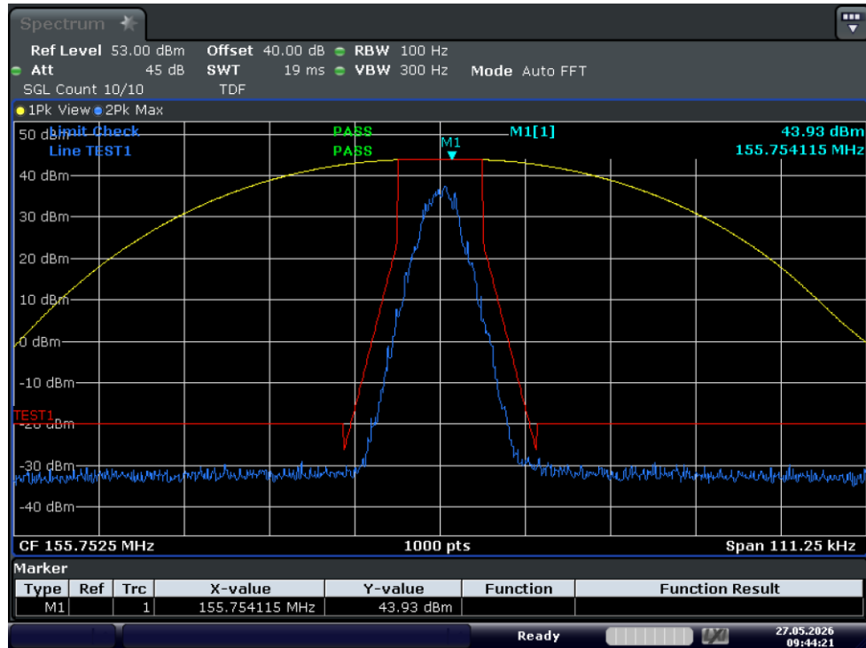
Test Graph 4FSK 25W 155.7525 12.5k Mask D
