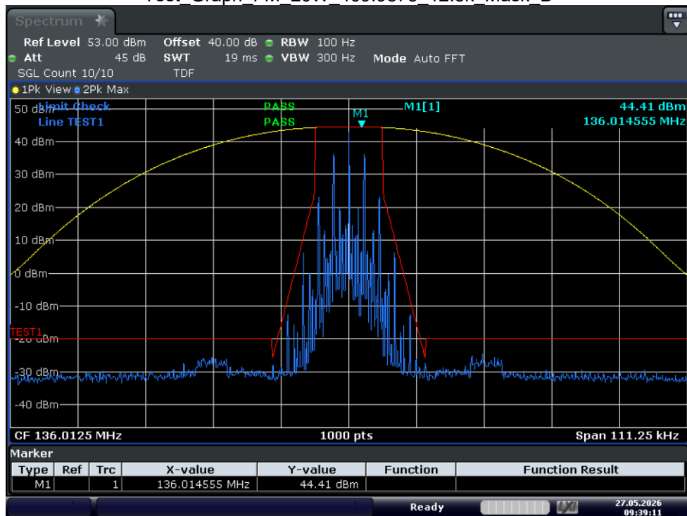
Test_Graph_FM_25W_136.0125_12.5k_Mask_D
