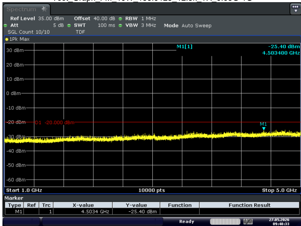
Test_Graph_FM_10W_136.0125_12.5k_TX_1G-5G
