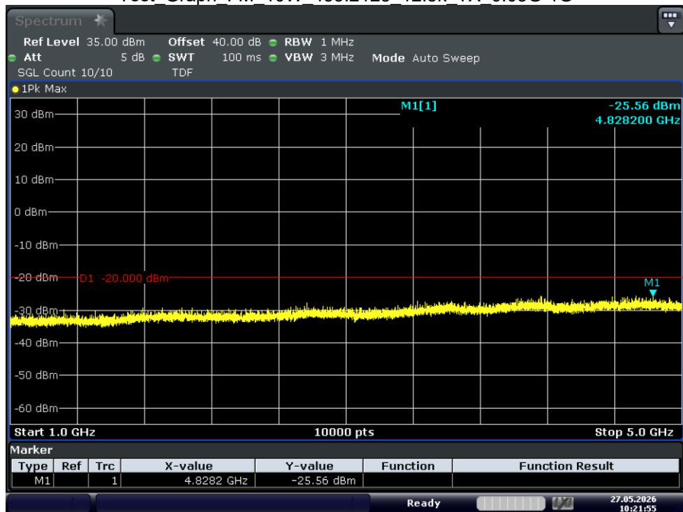
Test_Graph_FM_10W_453.2125_12.5k_TX_1G-5G
