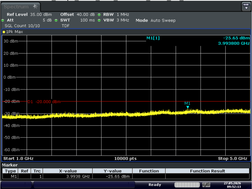
Test_Graph_4FSK_10W_136.0125_12.5k_TX_1G-5G
