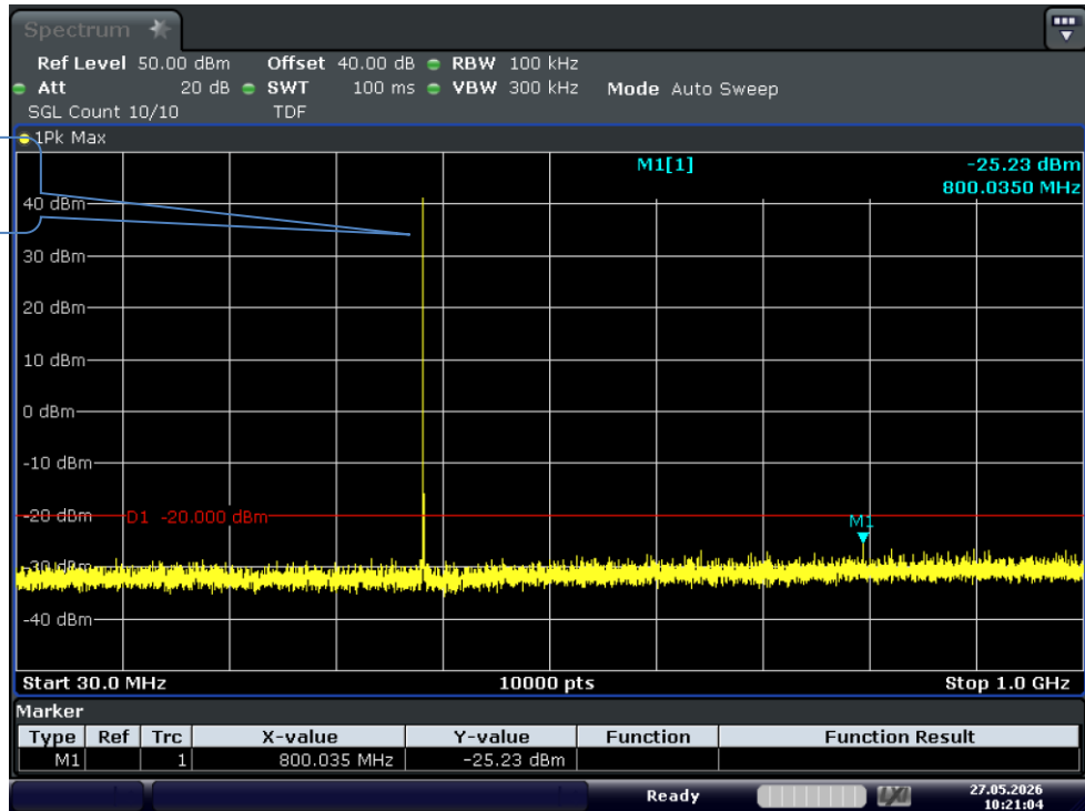
Test Graph FM 10W 400.0125 12.5k TX 0.03G-1G
