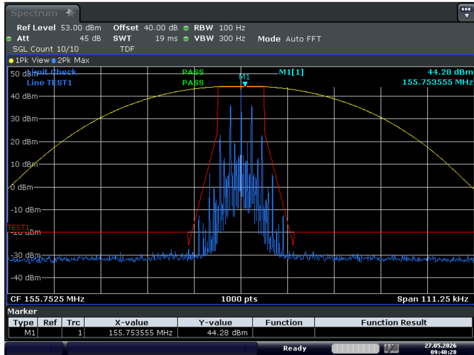
Test Graph FM 25W 155.7525 12.5k Mask D
