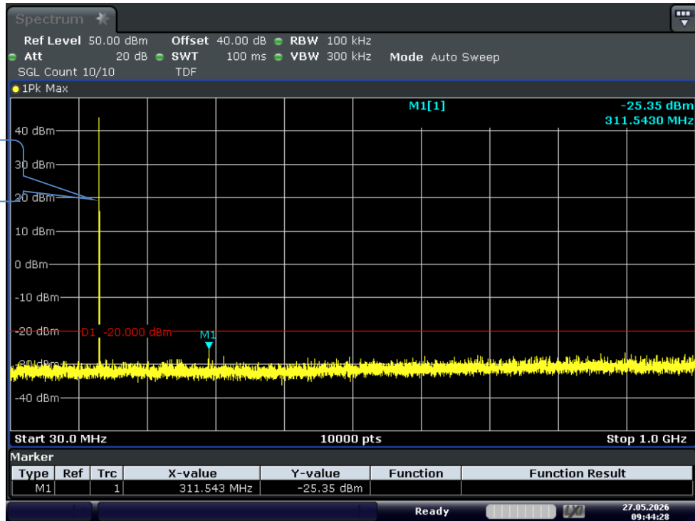
Test Graph 4FSK 25W 155.7525 12.5k TX 0.03G-1G
