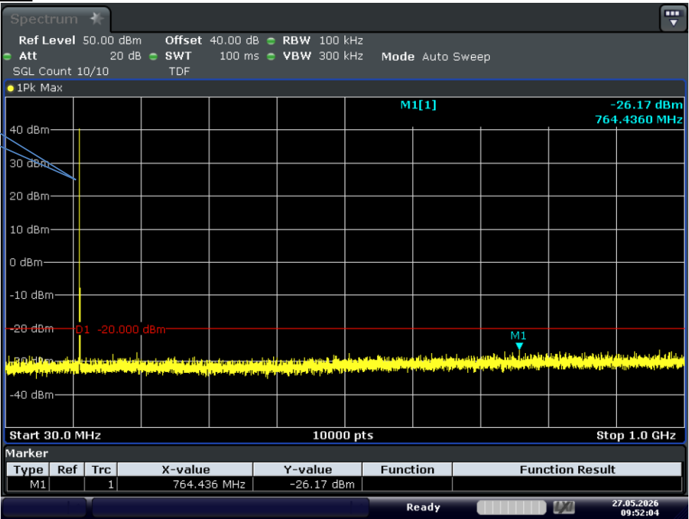
Test Graph 4FSK 10W 136.0125 12.5k TX 0.03G-1G
