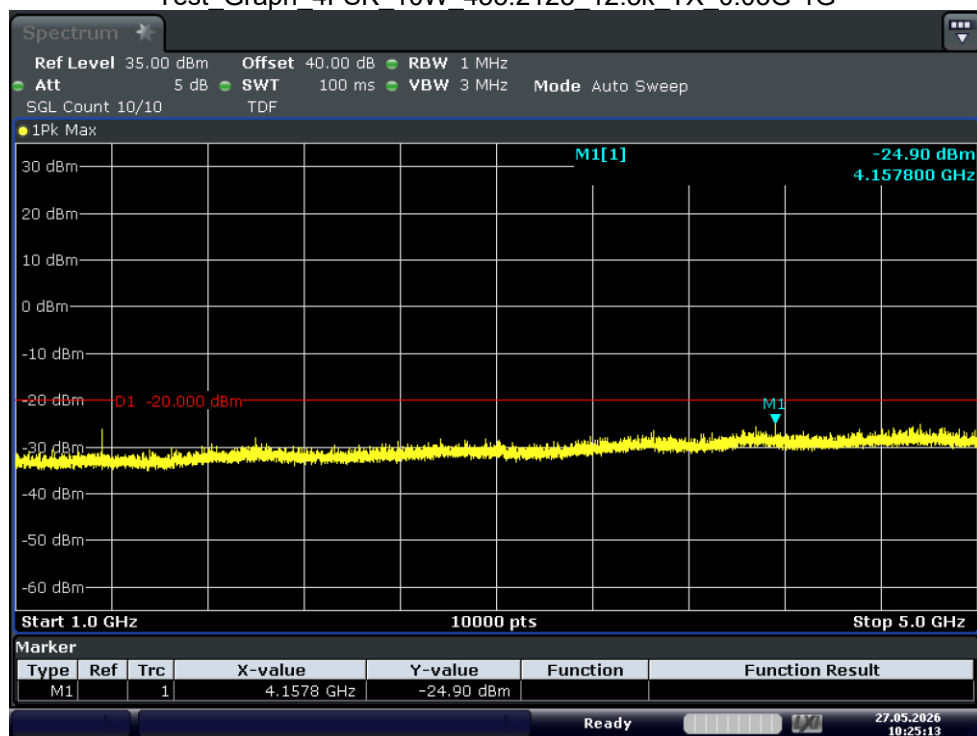
Test_Graph_4FSK_10W_453.2125_12.5k_TX_1G-5G
