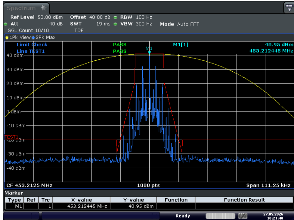
Test Graph FM 10W 453.2125 12.5k Mask D
