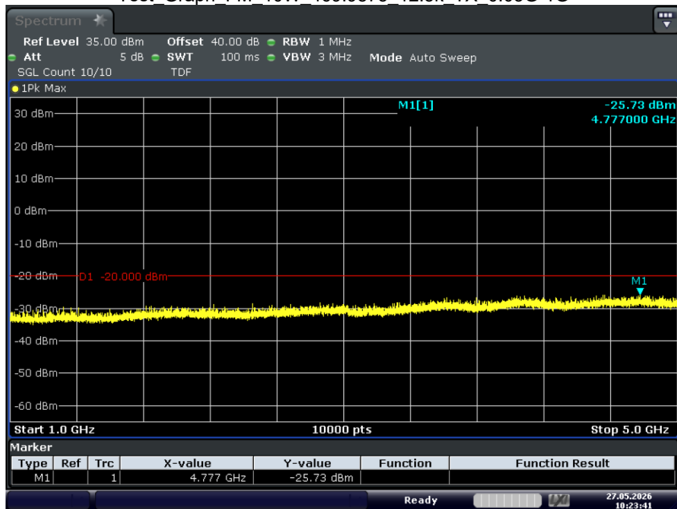
Test_Graph_FM_10W_469.9875_12.5k_TX_1G-5G
