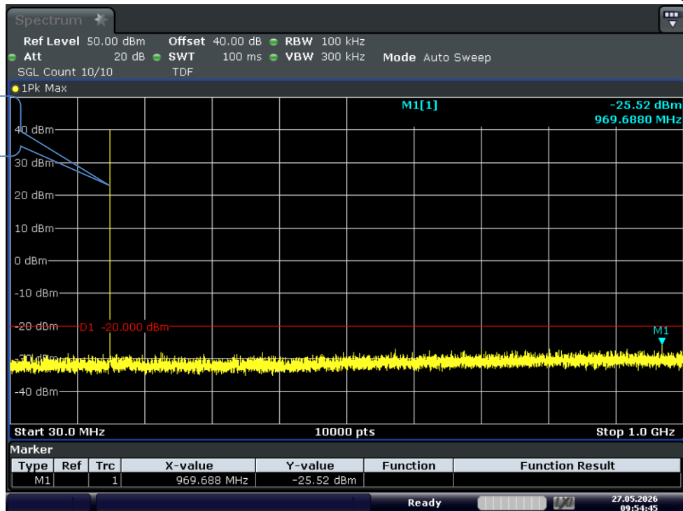
Test Graph 4FSK 10W 173.9875 12.5k TX 0.03G-1G
