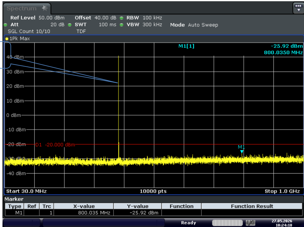
Test Graph 4FSK 10W 400.0125 12.5k TX 0.03G-1G
