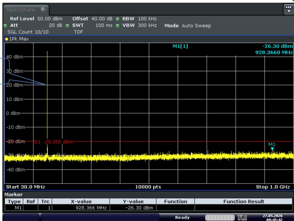
Test Graph 4FSK 25W 173.9875 12.5k TX 0.03G-1G
