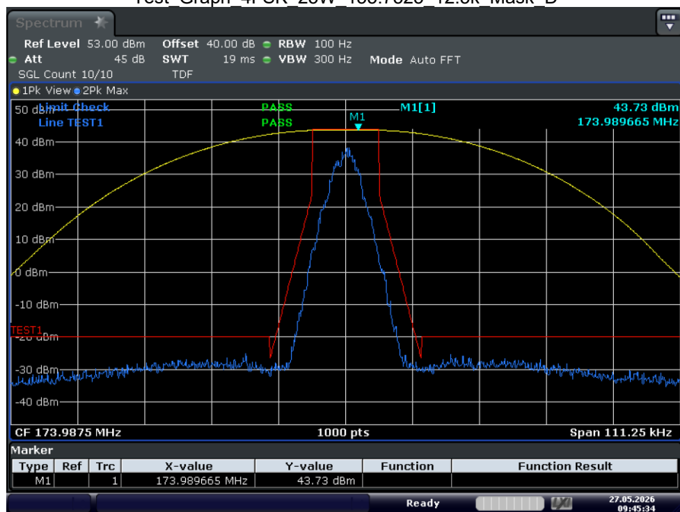
Test_Graph_4FSK_25W_173.9875_12.5k_Mask_D
