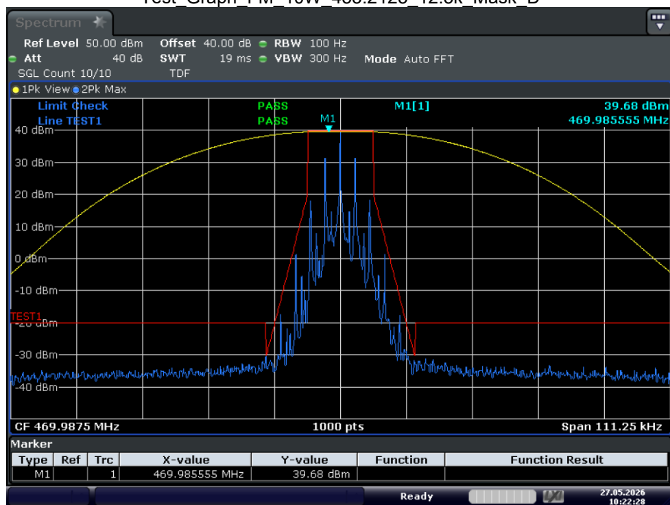
Test_Graph_FM_10W_469.9875_12.5k_Mask_D
