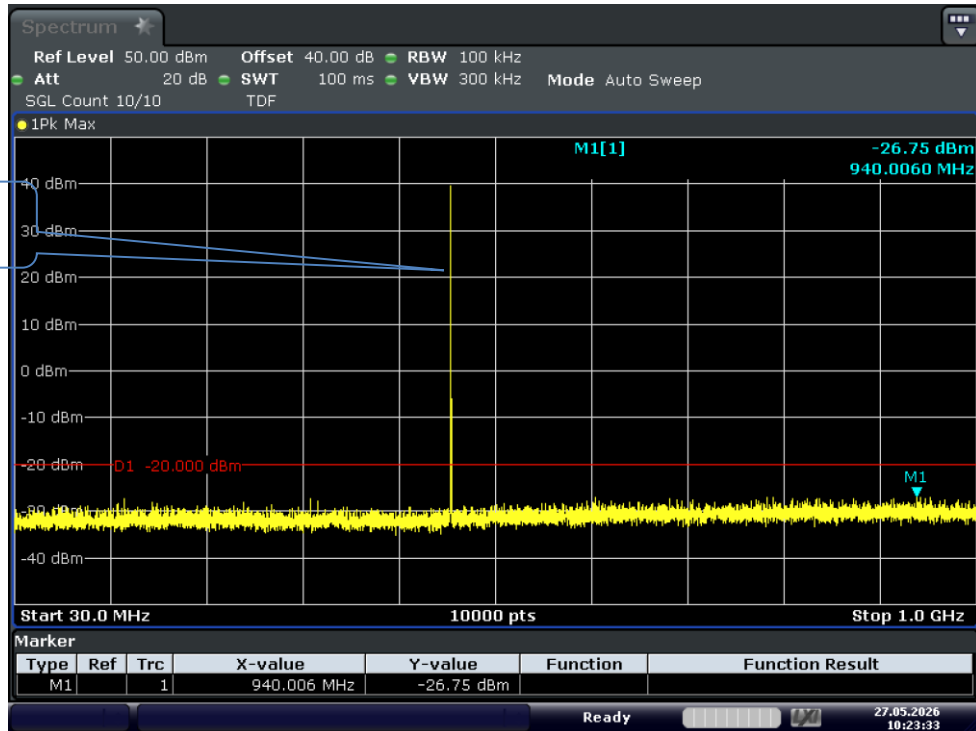
Test Graph FM 10W 469.9875 12.5k TX 0.03G-1G
