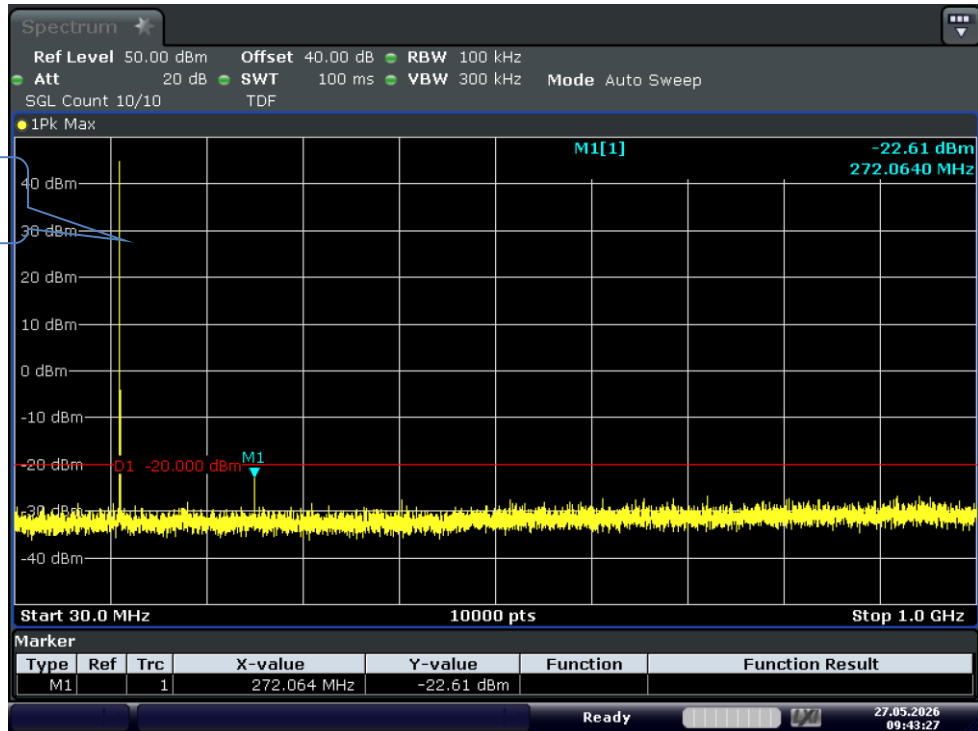
Test Graph 4FSK 25W 136.0125 12.5k TX 0.03G-1G
