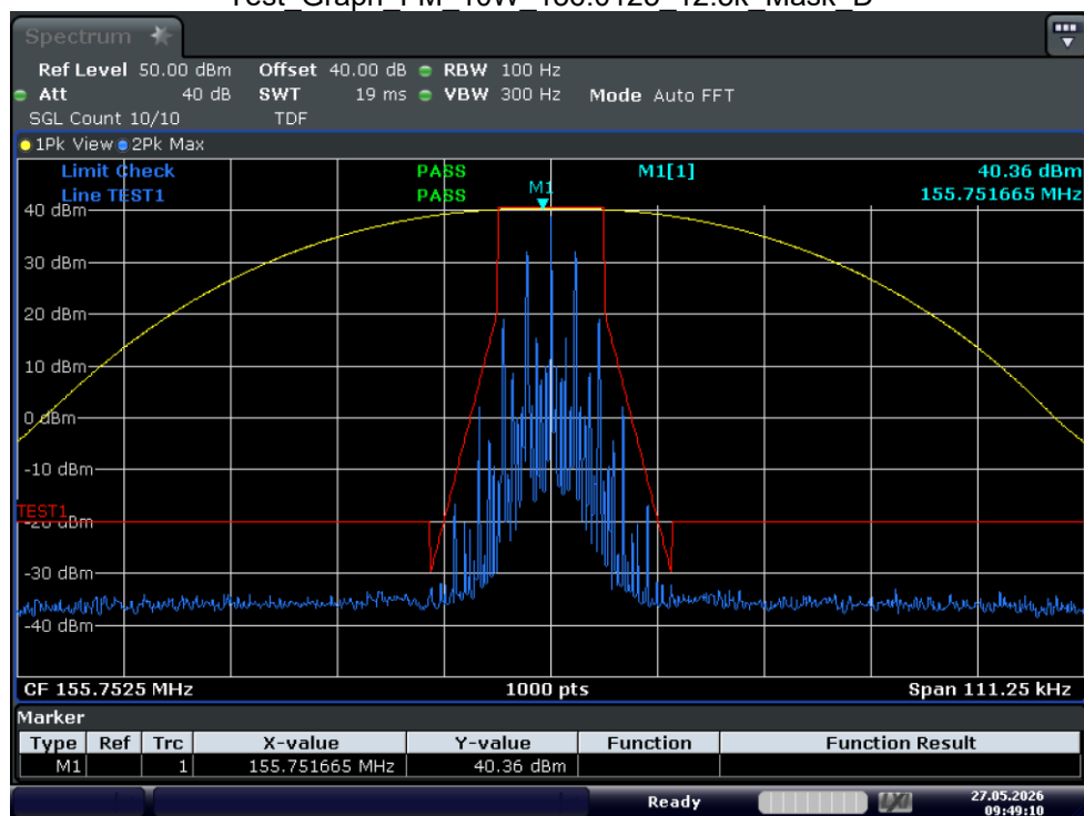
Test_Graph_FM_10W_155.7525_12.5k_Mask_D
