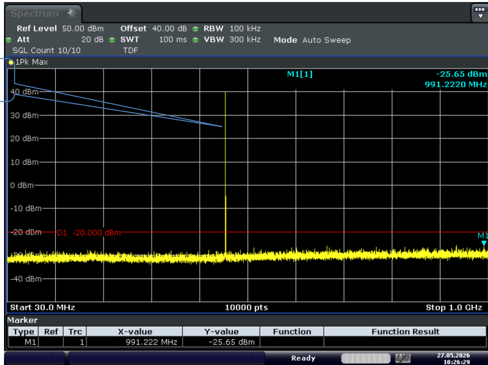
Test Graph 4FSK 10W 469.9875 12.5k TX 0.03G-1G
