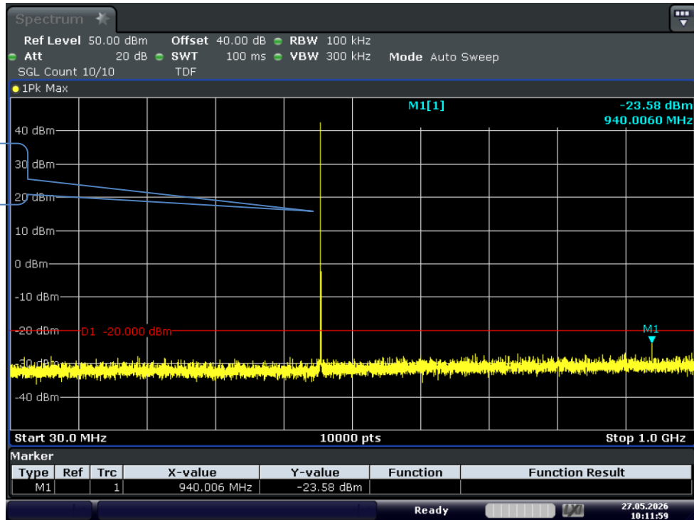
Test Graph FM 20W 469.9875 12.5k TX 0.03G-1G
