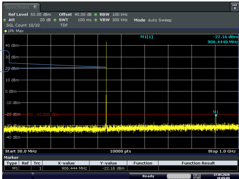
Test Graph FM 20W 453.2125 12.5k TX 0.03G-1G
