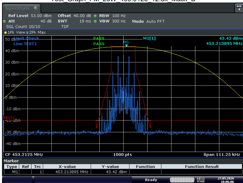
Test_Graph_FM_20W_453.2125_12.5k_Mask_D
