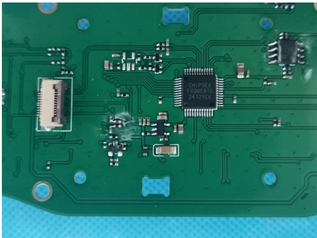
Internal View of EUT (Figure 16)
