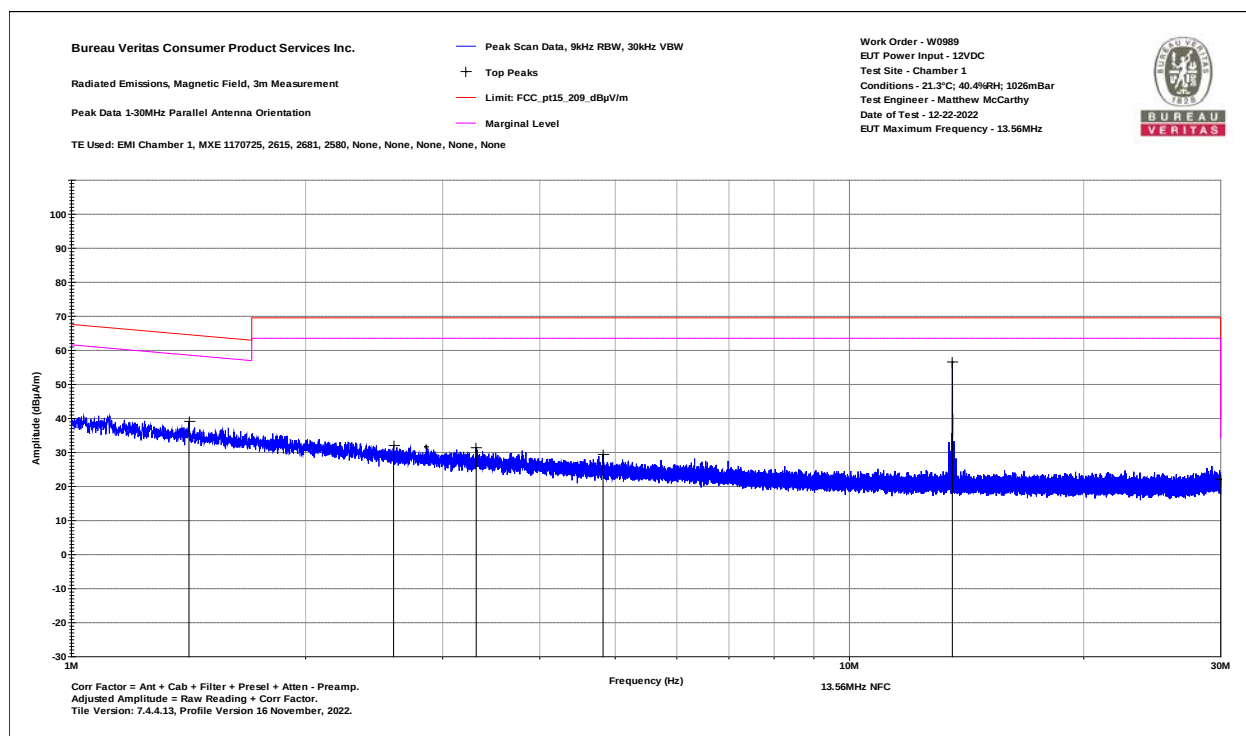
1MHz – 30MHz Parallel Plot
