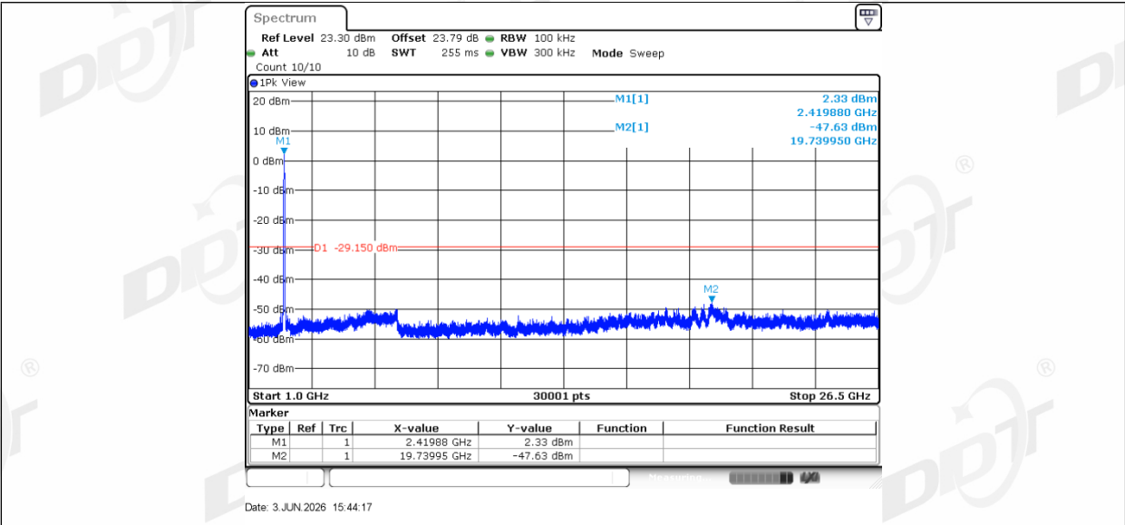
11N40SISO_Ant1_2437_0~Reference
