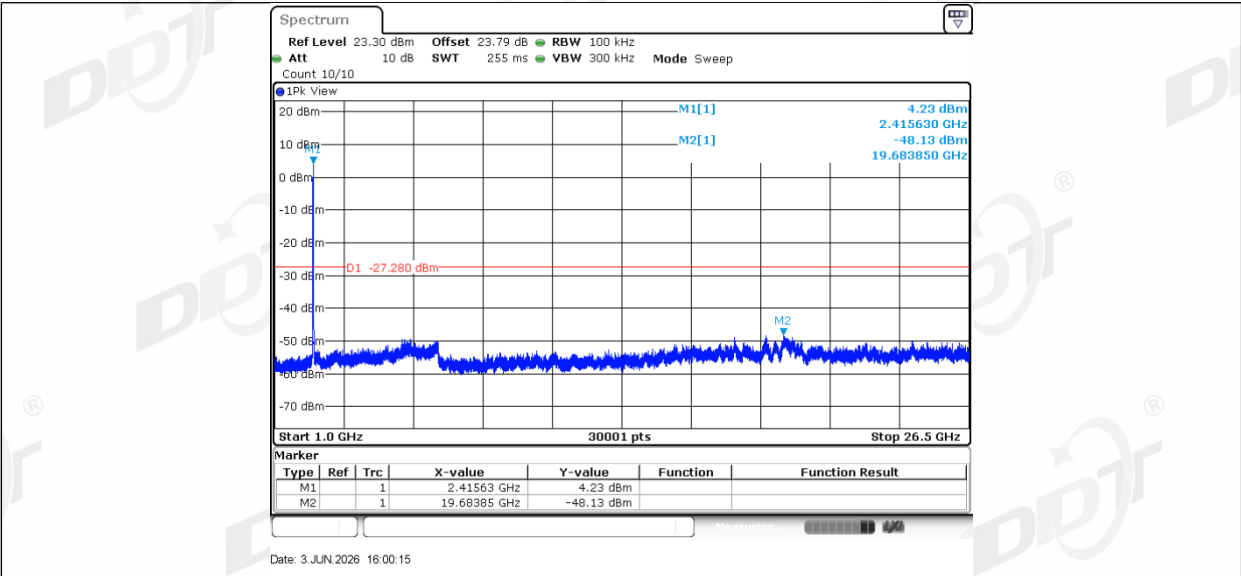
11AX20SISO Ant1 2437 0~Reference
