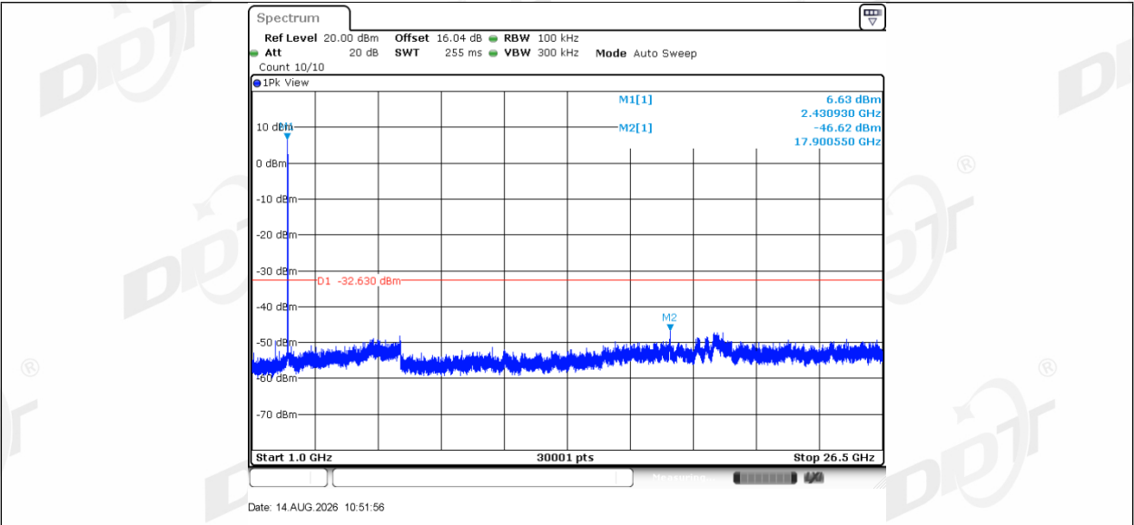
11AX20SISO Ant1 2437 52Tone RU39 0~Reference
