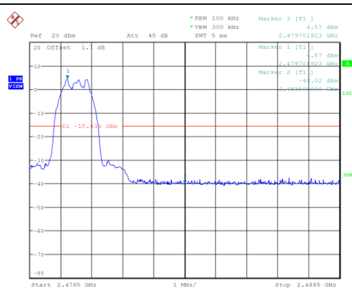
Frequency Band Edge:8DPSK,Ch78, Hopping OFF
