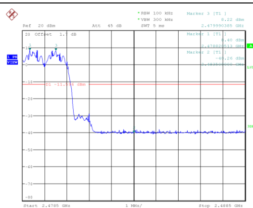
Frequency Band Edge: 8DPSK, Ch78, Hopping ON
