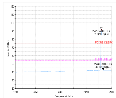
Bandedge: Ch39
