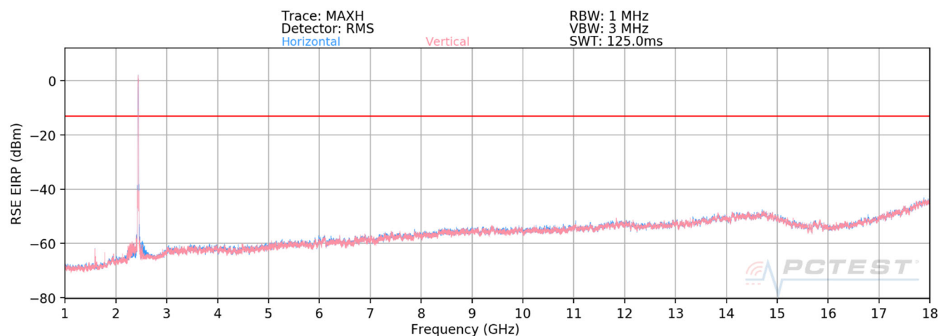
Plot 7-1. Radiated Spurious Plot above 1GHz (B14 10MHz Mid Channel + AP(2.4GHz) 802.11b Ch 6)
