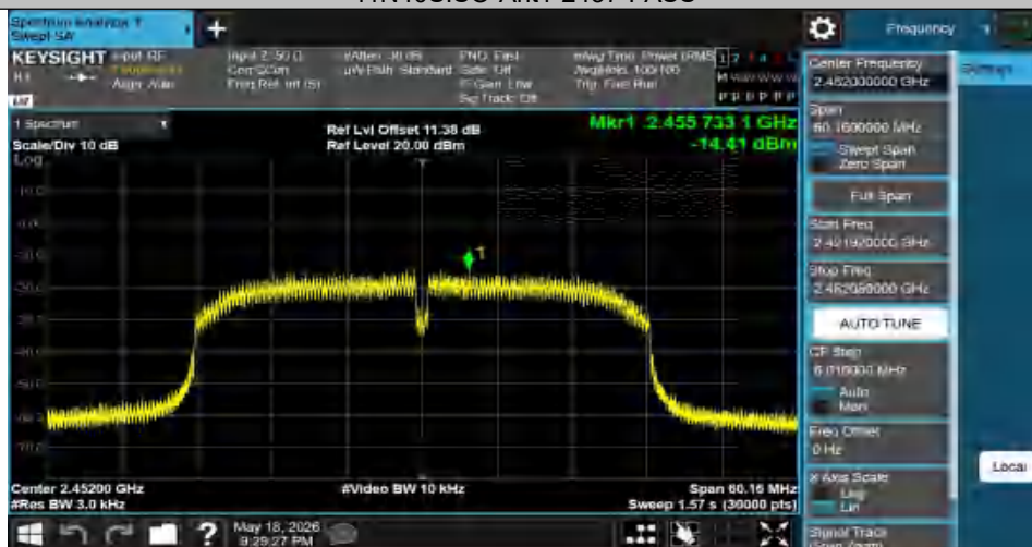
11N40SISO-Ant1-2452-PASS
