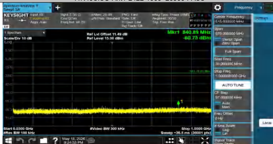
11N40SISO-Ant1-2437-30~1000-PASS
