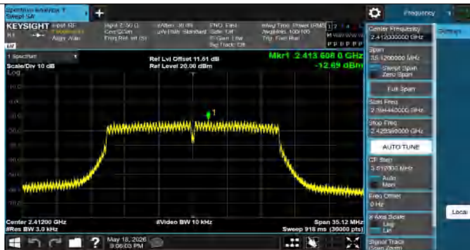
11N20SISO-Ant1-2412-PASS
