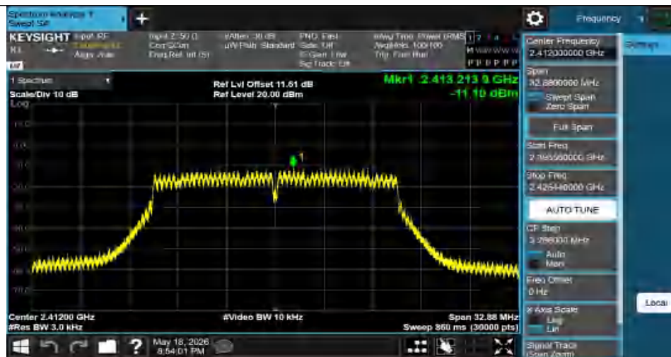
11G-Ant1-2412-PASS
