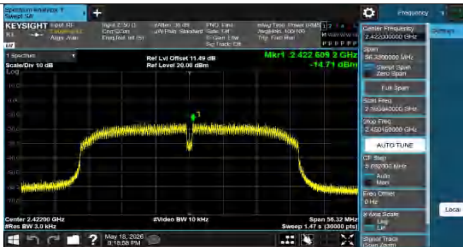
11N40SISO-Ant1-2422-PASS
