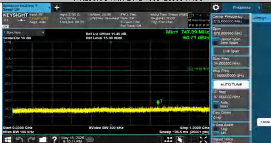
11N20SISO-Ant1-2437-30~1000-PASS
