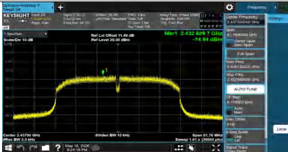
11N40SISO-Ant1-2437-PASS
