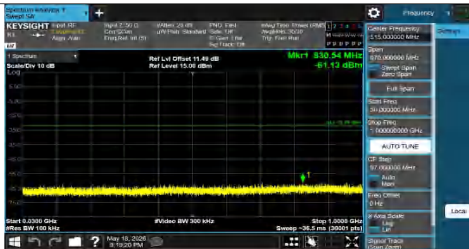
11N40SISO-Ant1-2422-30~1000-PASS
