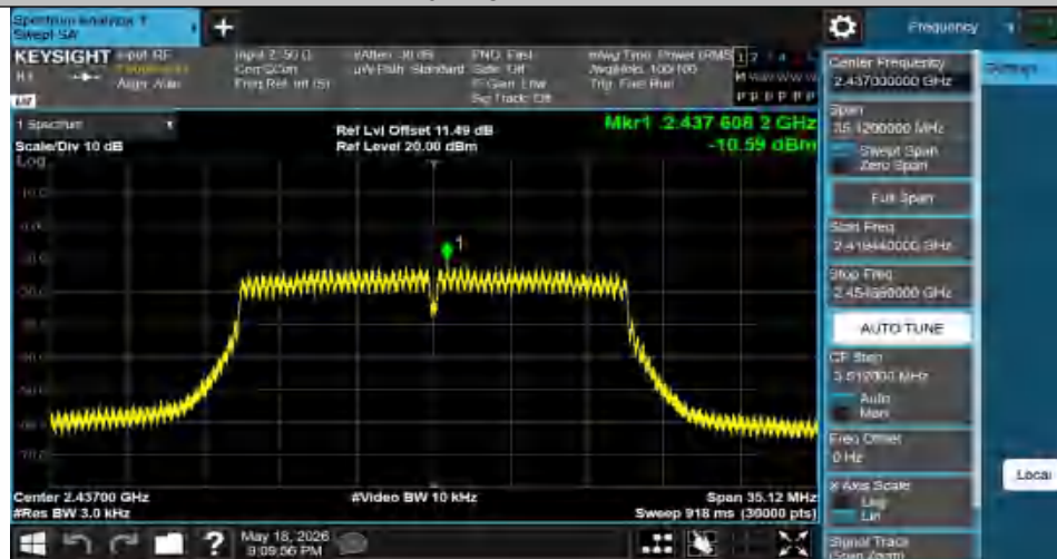
11N20SISO-Ant1-2437-PASS
