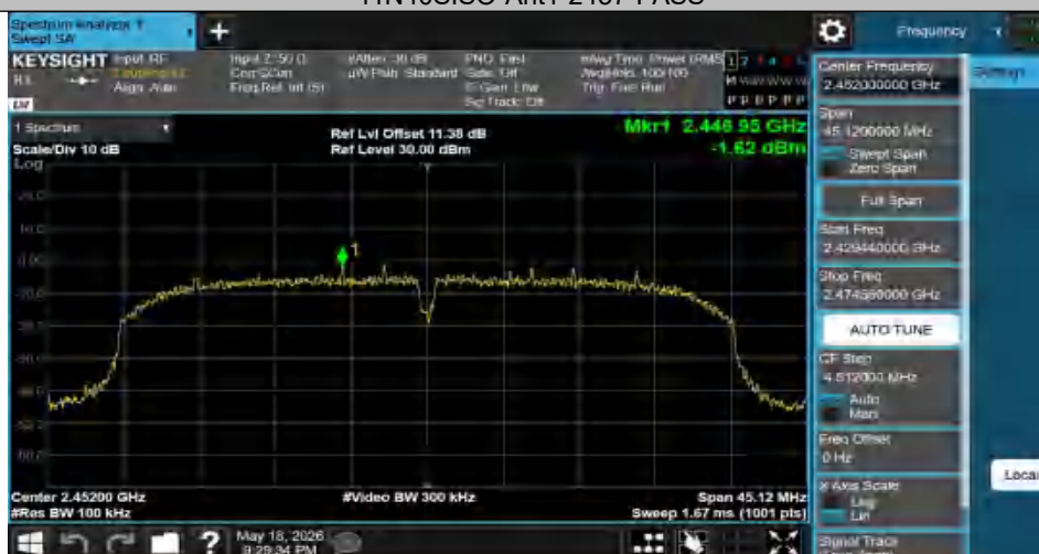
11N40SISO-Ant1-2452-PASS
