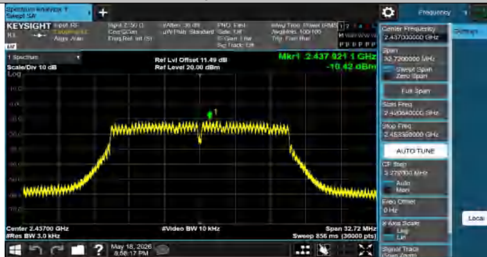
11G-Ant1-2437-PASS
