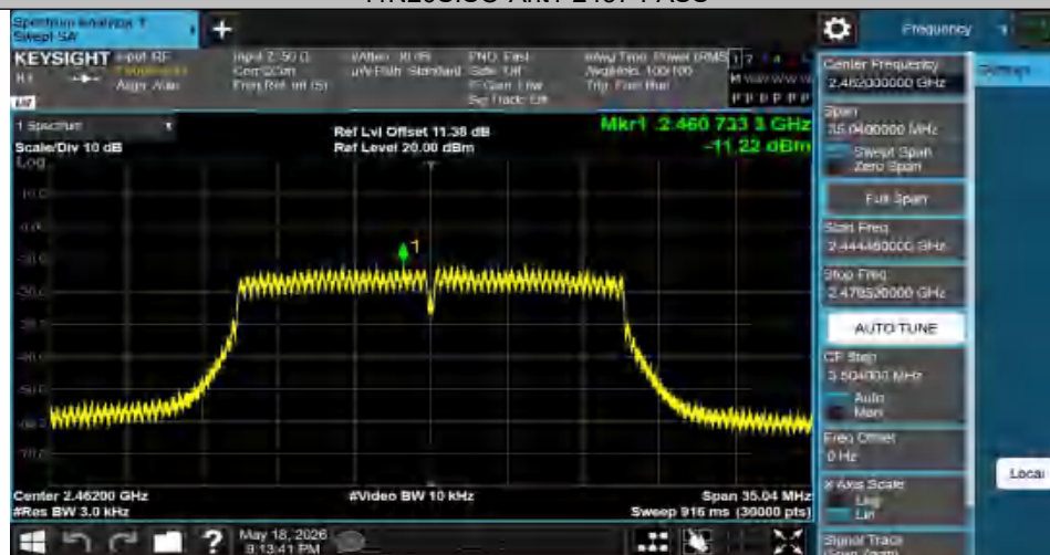
11N20SISO-Ant1-2462-PASS
