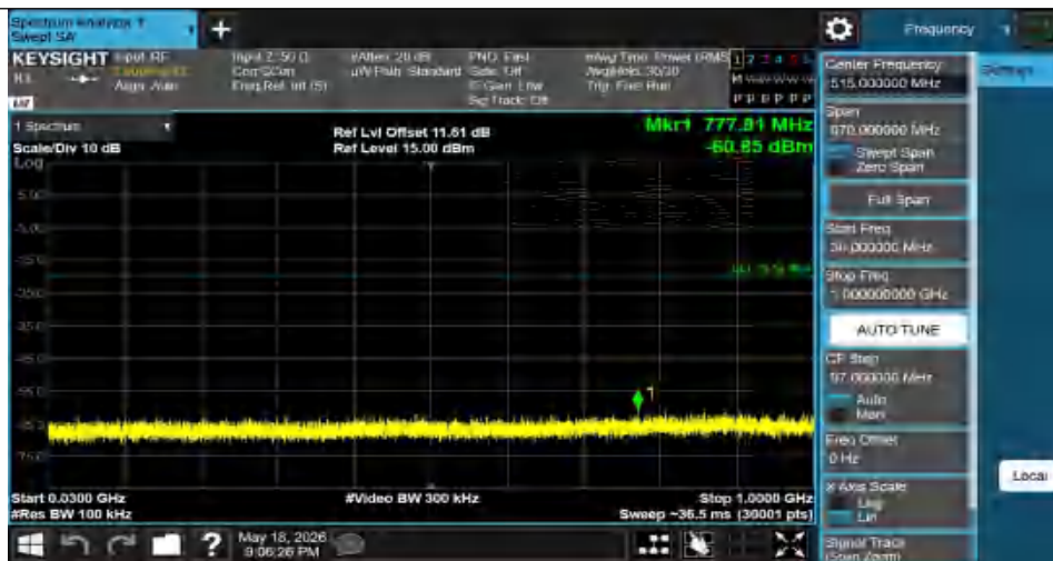
11N20SISO-Ant1-2412-30~1000-PASS
