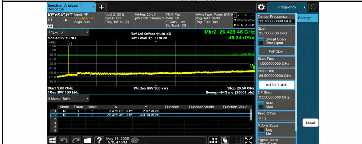
BLE_1M-Ant1-2480-1000~26500-PASS
