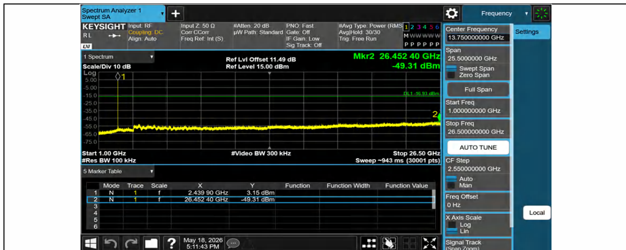
BLE_1M-Ant1-2440-1000~26500-PASS
