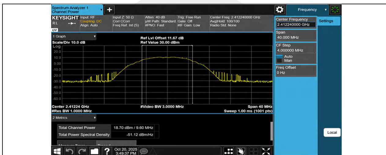
11B-Ant1-2412-PASS
