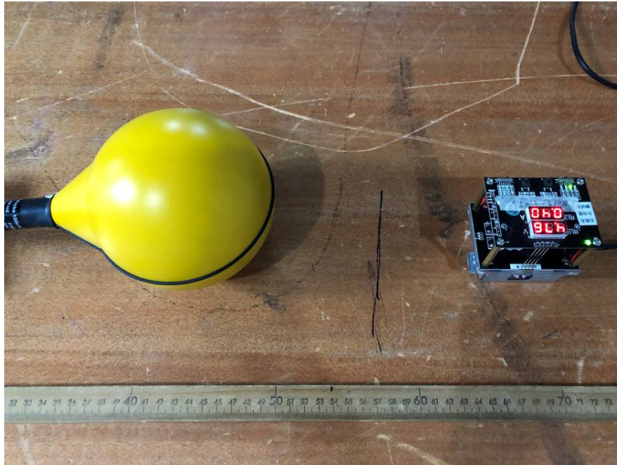
H-Filed Strength View Position A (Test distance: 15cm)
