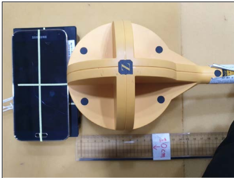
Photo of MPE Test Set up at 6 cm distance (H-field)
