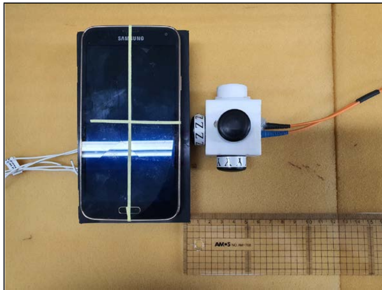
Photo of MPE Test Set up at 4 cm distance (E-field)
