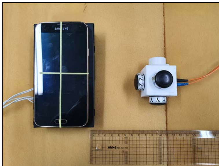
Photo of MPE Test Set up at 10 cm distance (E-field)
