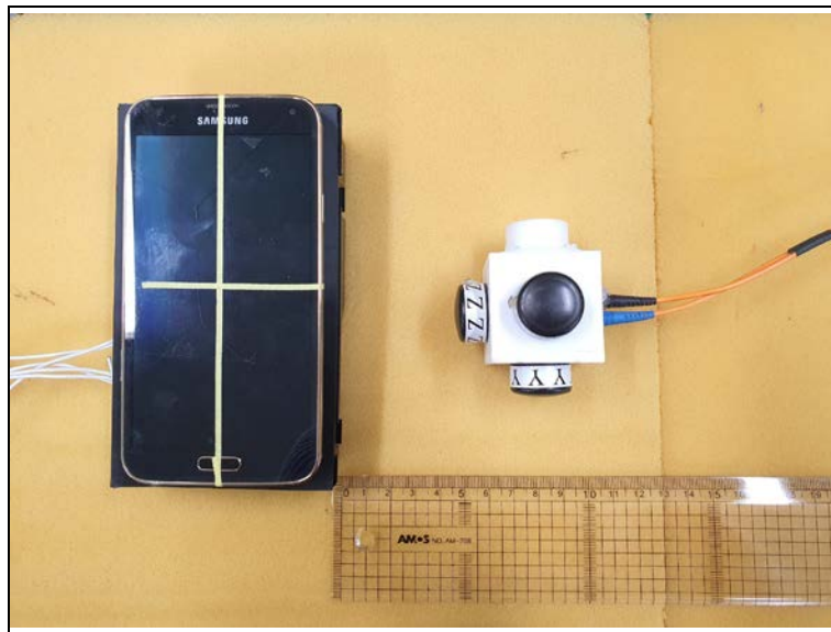
Photo of MPE Test Set up at 6 cm distance (E-field)
