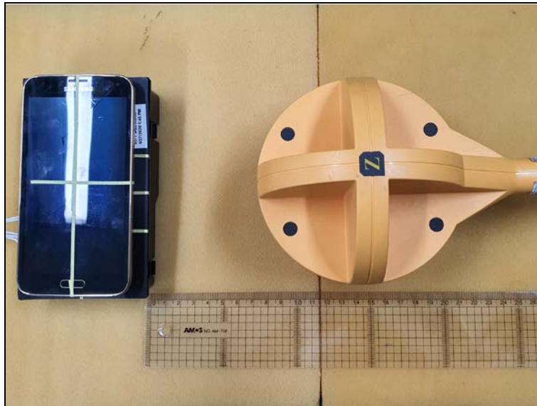
Photo of MPE Test Set up at 10 cm distance (H-field)
