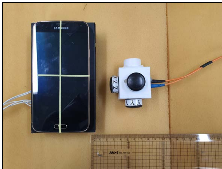
Photo of MPE Test Set up at 6 cm distance (E-field)
