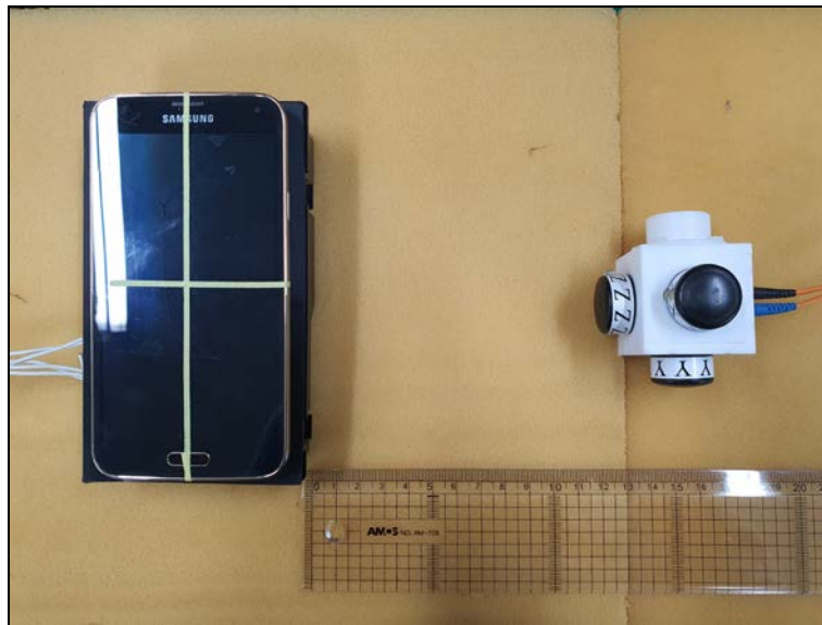
Photo of MPE Test Set up at 10 cm distance (E-field)
