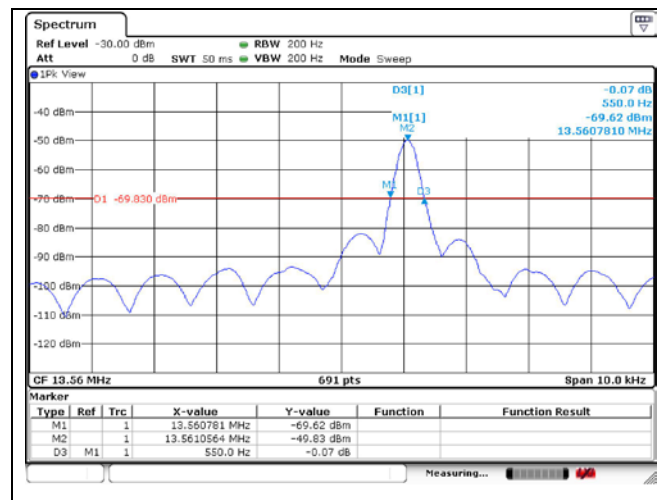
20 dB Bandwidth
