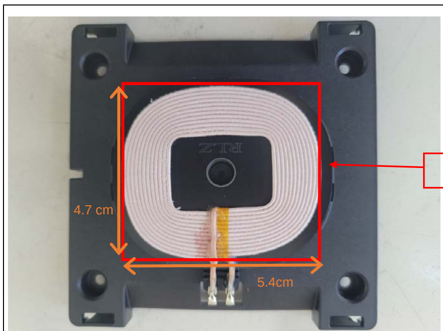
coil antenna
