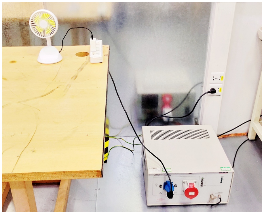
Conducted Emission Test Setup:
