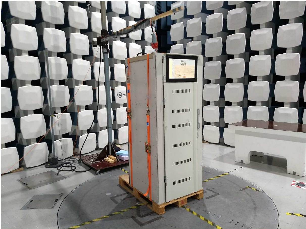
Radiated Emissions, 9 kHz – 1000 MHz
