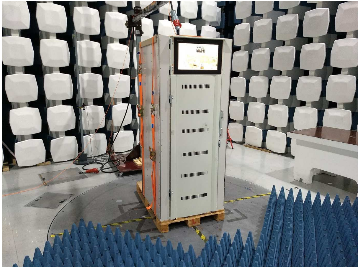
Radiated Emissions, 1000 – 12000 MHz
