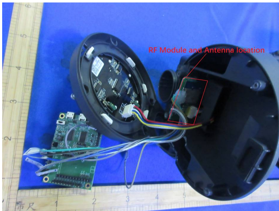
Internal View of RF Module and Antenna
