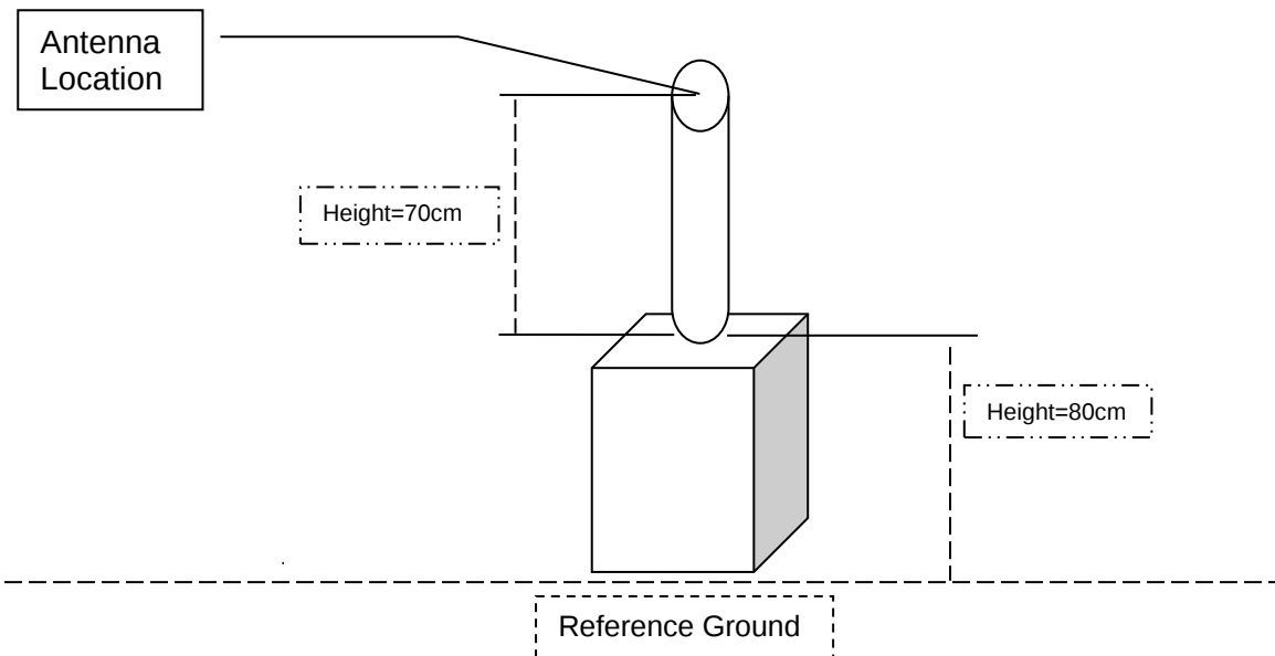
RADIATED RF MEASUREMENT SETUP (ABOVE 1 GHz- X axis)-Part 2
