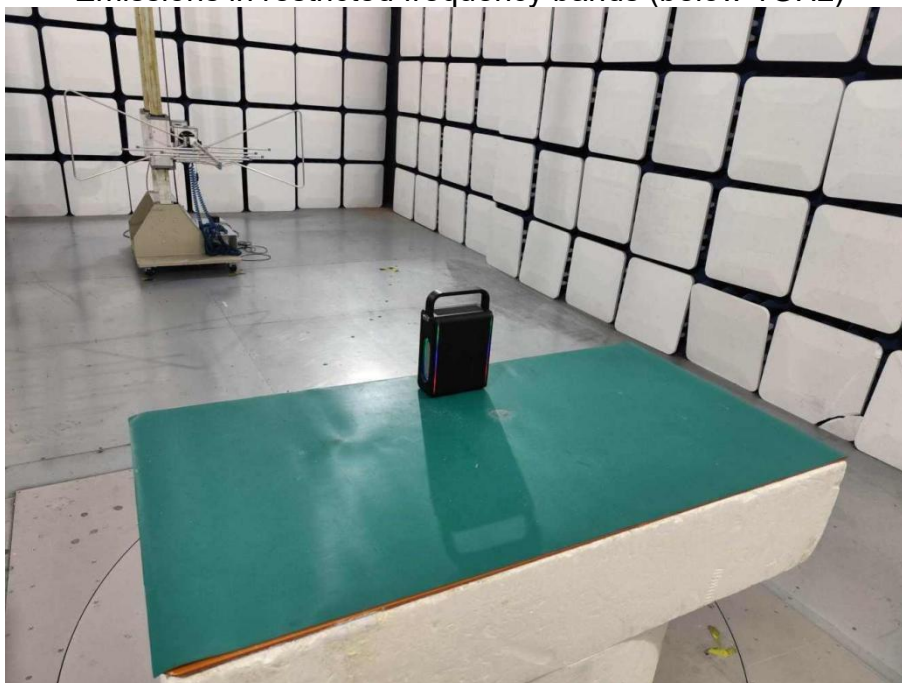
Band edge emissions (Radiated) Emissions in restricted frequency bands (below 1GHz)
