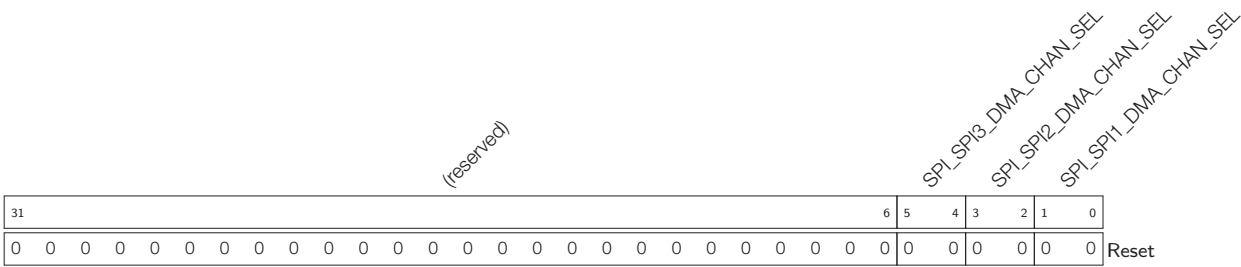
Register 5.202: SPI_DMA_CHAN_SEL_REG (0x5A8)
