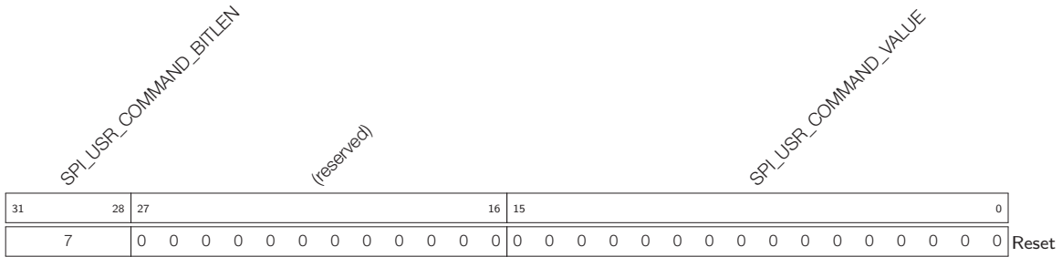
Register 7.10: SPI_USER2_REG (0x24)
