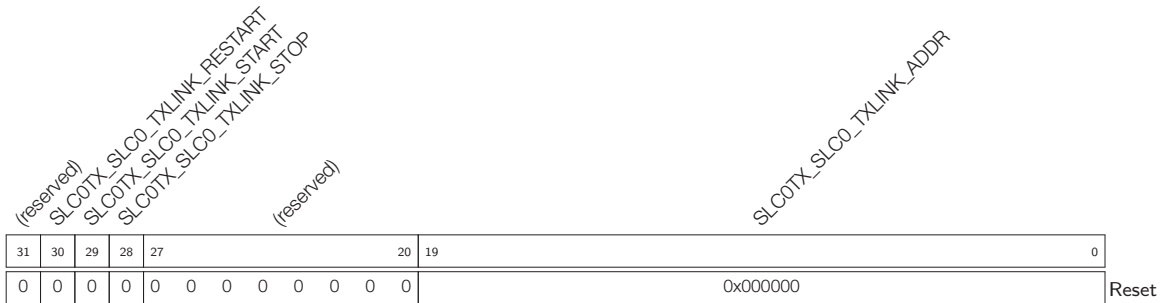
Register 8.7: SLC0TX_LINK_REG (0x40)
