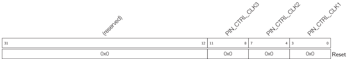
Register 4.33: IO_MUX_PIN_CTRL (0x3FF49000)
