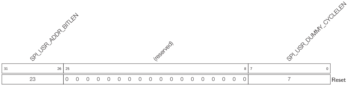
Register 7.9: SPI_USER1_REG (0x20)
