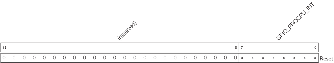
Register 4.28: GPIO_PCPU_INT1_REG (0x007c)
