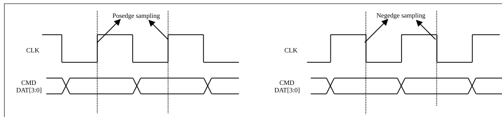
Figure 28: Sampling Timing Diagram
