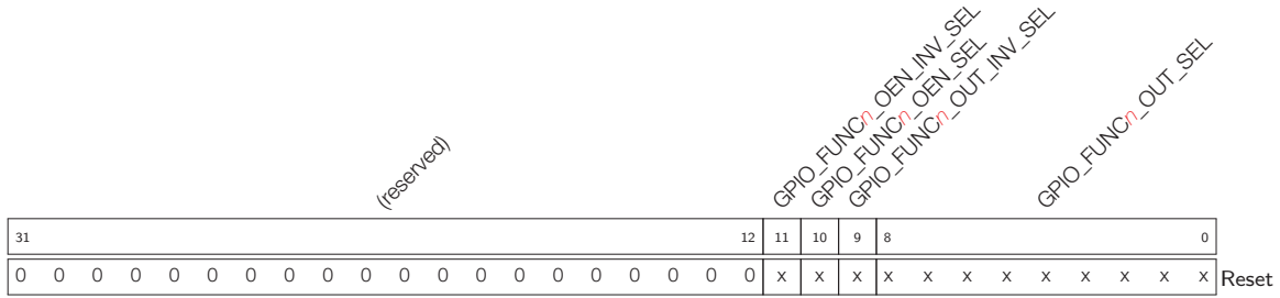
Register 4.32: GPIO_FUNC n _OUT_SEL_CFG_REG ( n : 0-19, 21-23, 25-27, 32-33) (0x530+0x4* n )
