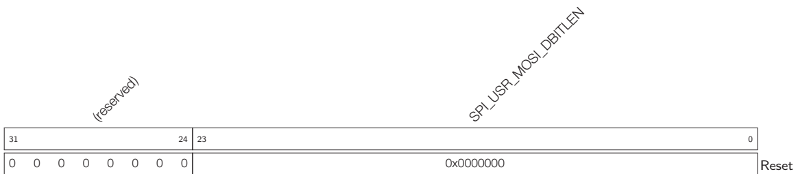
Register 7.11: SPI_MOSI_DLEN_REG (0x28)
