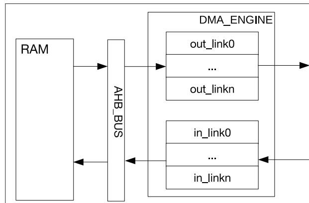
Figure 11: DMA Engine Architecture
