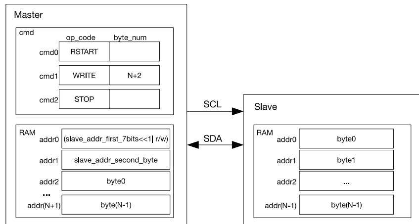
Figure 52: I2C Master Writes to Slave with 10-bit Address
