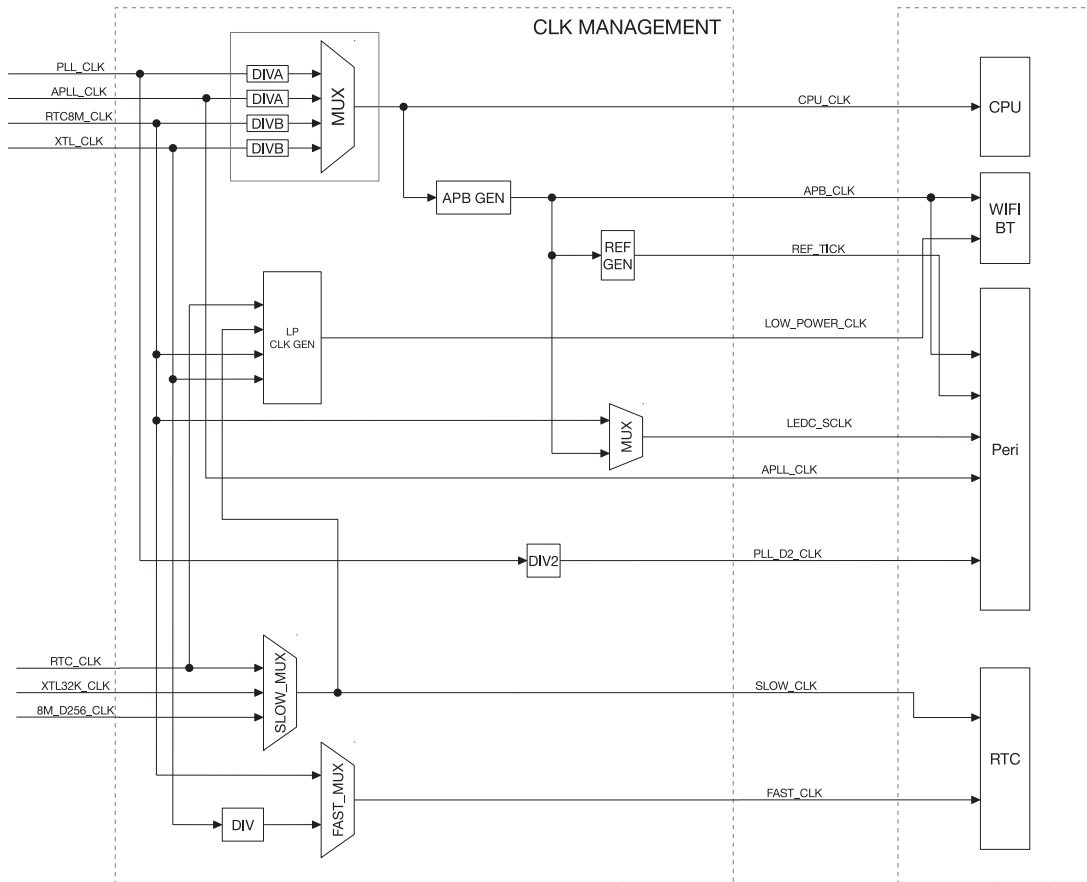
Figure 6: System Clock
