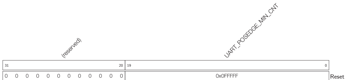
Register 13.25: UART_POSPULSE_REG (0x68)
