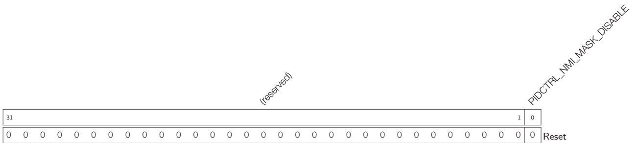
Register 27.16: PIDCTRL_NMI_MASK_DISABLE_REG (0x058)
