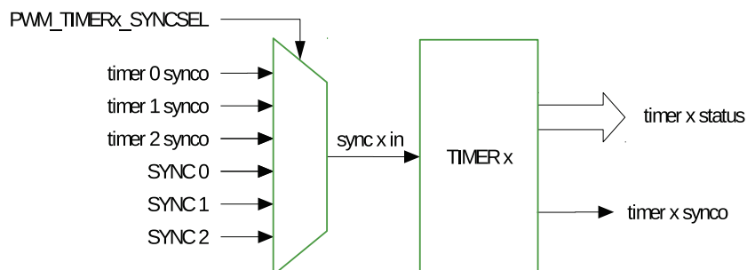
Figure 92: Timer Submodule
