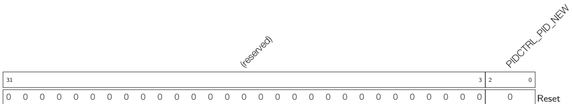
Register 27.13: PIDCTRL_PID_NEW_REG (0x048)
