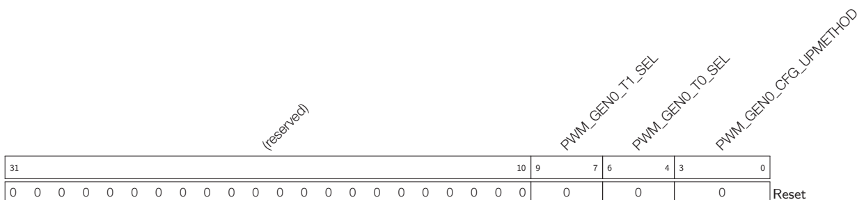
Register 16.19: PWM_GEN0_CFG0_REG (0x0048)
