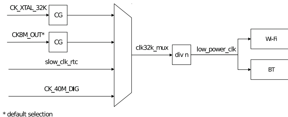
Figure 169: Digital Low-Power Clocks
