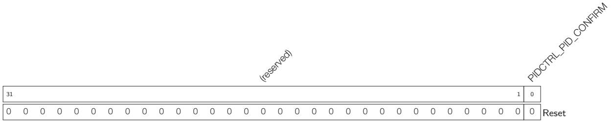
Register 27.14: PIDCTRL_PID_CONFIRM_REG (0x04C)
