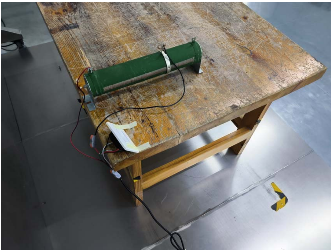
Conducted Emissions Side View- Model:SNA042CLR3-ZB-1X1200-P
