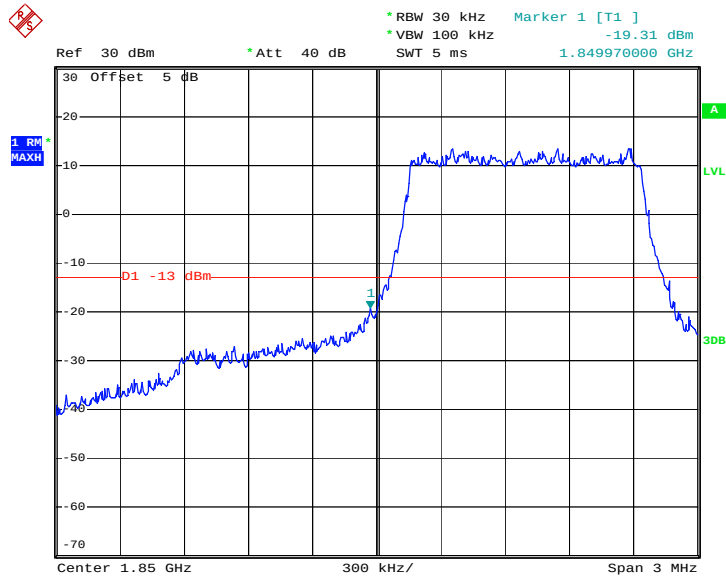
QPSK_1.4MHz_ 6 RB_ Left
