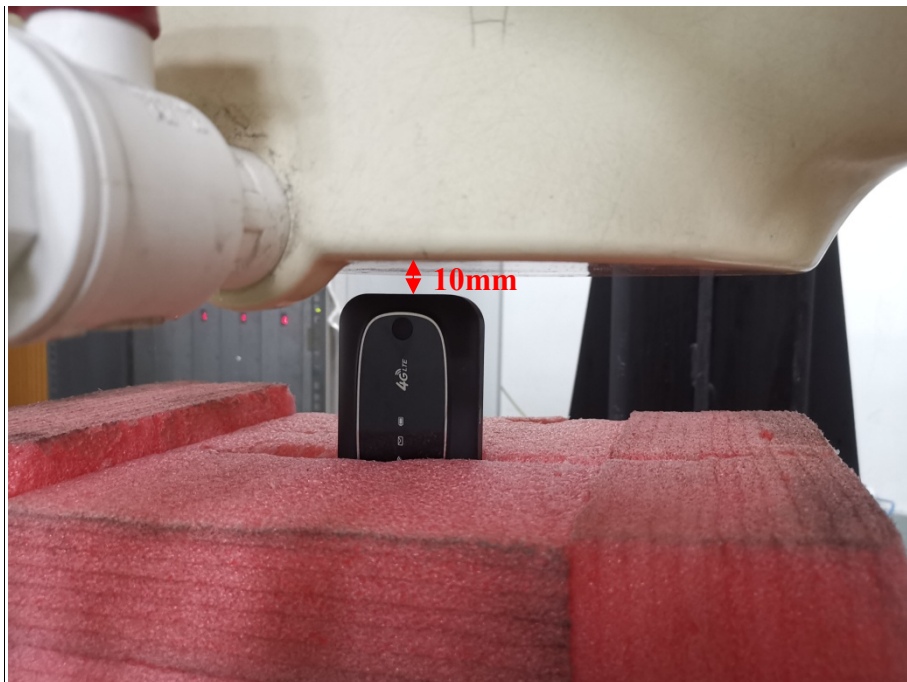
Body Bottom Setup Photo (10mm) ( Mode:M7)
