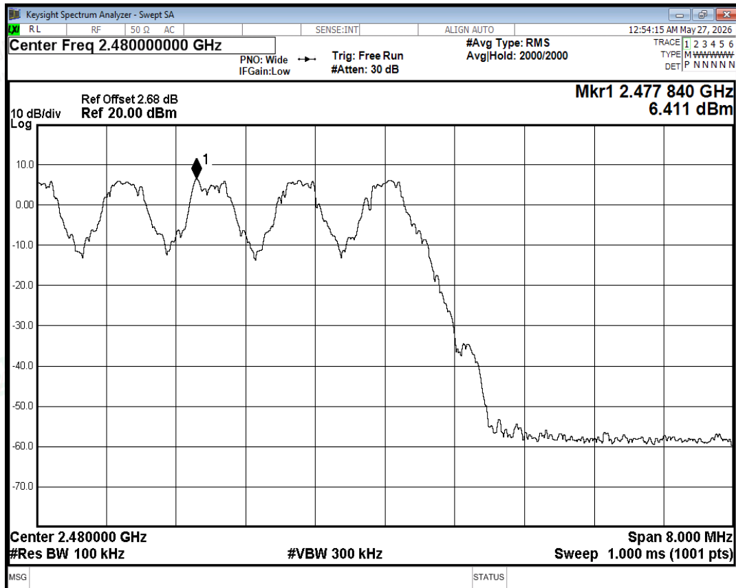
Band Edge(Hopping) NVNT 1-DH5 2480MHz Ant Hopping Ref
