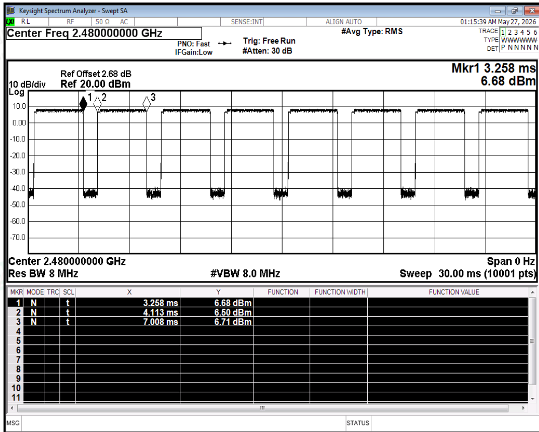
Duty Cycle NVNT 3-DH5 2480MHz Ant
