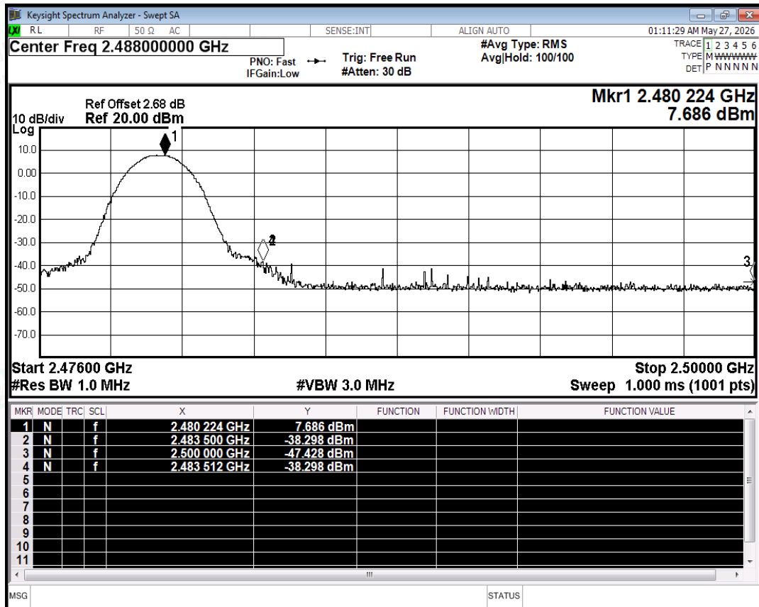
Restrict Band NVNT 2-DH5 2480MHz Ant No-Hopping Peak
