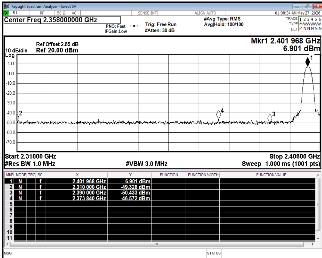
Restrict Band NVNT 2-DH5 2402MHz Ant No-Hopping Peak
