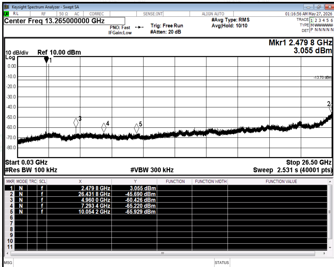
Tx. Spurious NVNT 3-DH5 2480MHz Ant Emission
