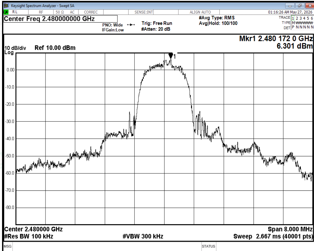
Tx. Spurious NVNT 3-DH5 2480MHz Ant Ref
