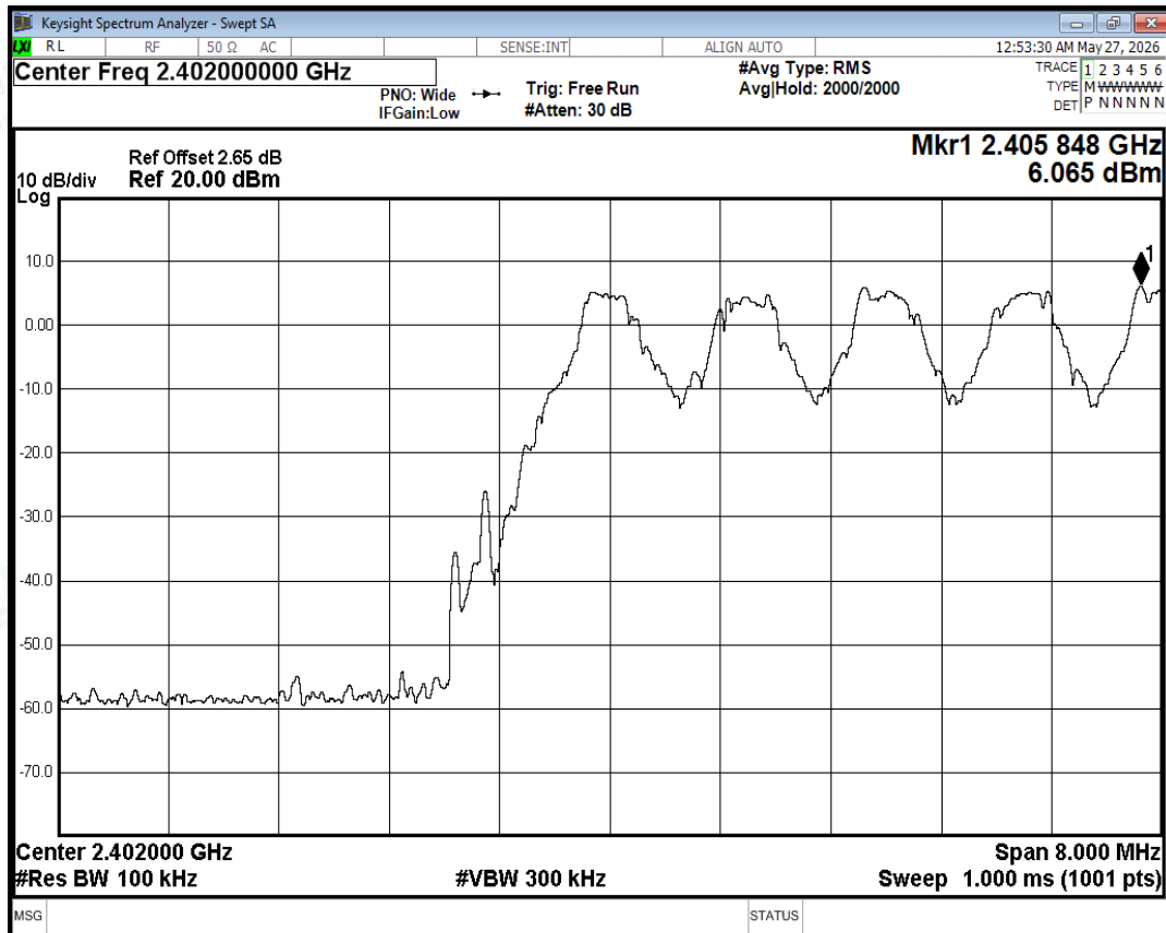
Band Edge(Hopping) NVNT 1-DH5 2402MHz Ant Hopping Ref
