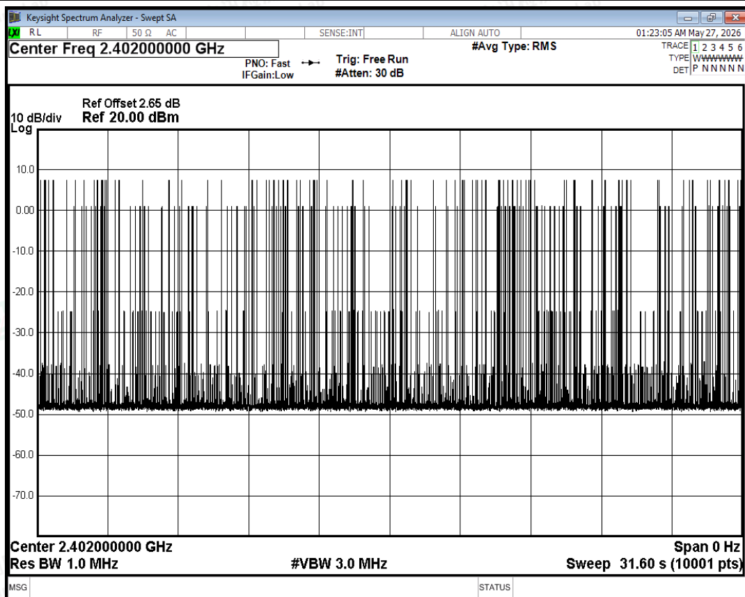
Dwell NVNT 3-DH5 2402MHz Ant Accumulated
