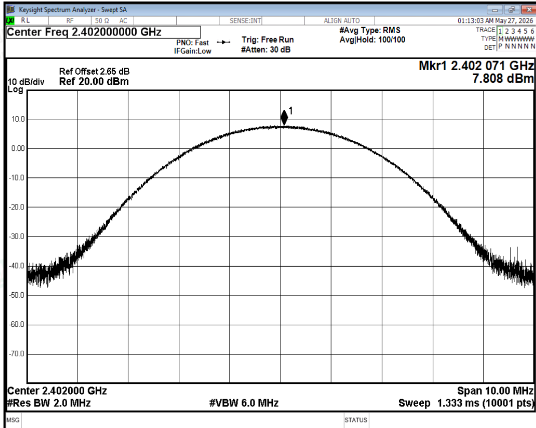
Peak Power NVNT 3-DH5 2402MHz Ant
