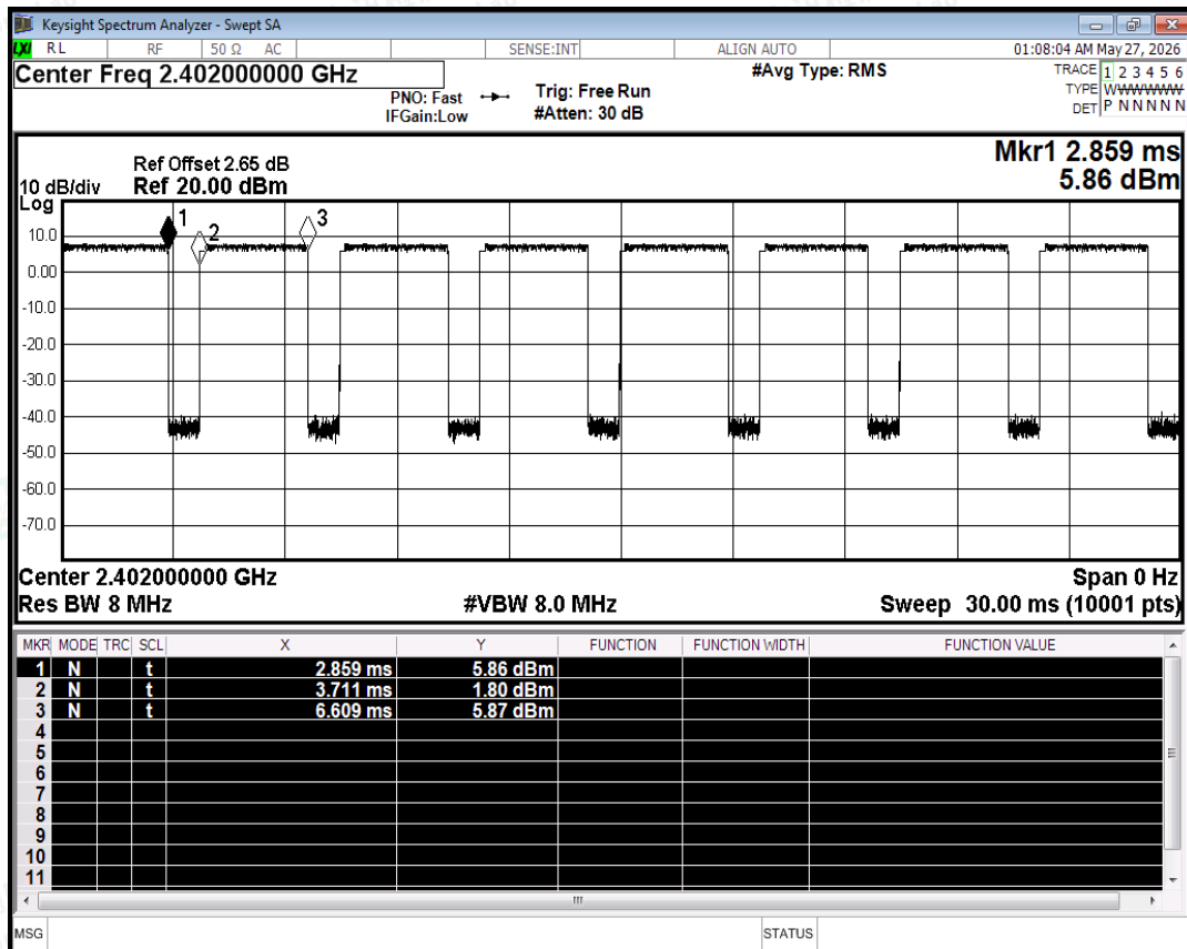
Duty Cycle NVNT 2-DH5 2402MHz Ant
