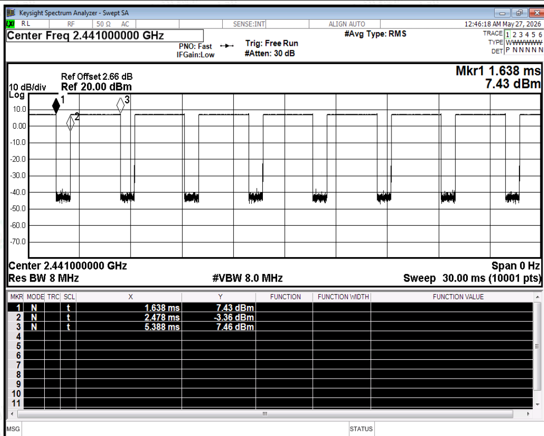
Duty Cycle NVNT 1-DH5 2441MHz Ant
