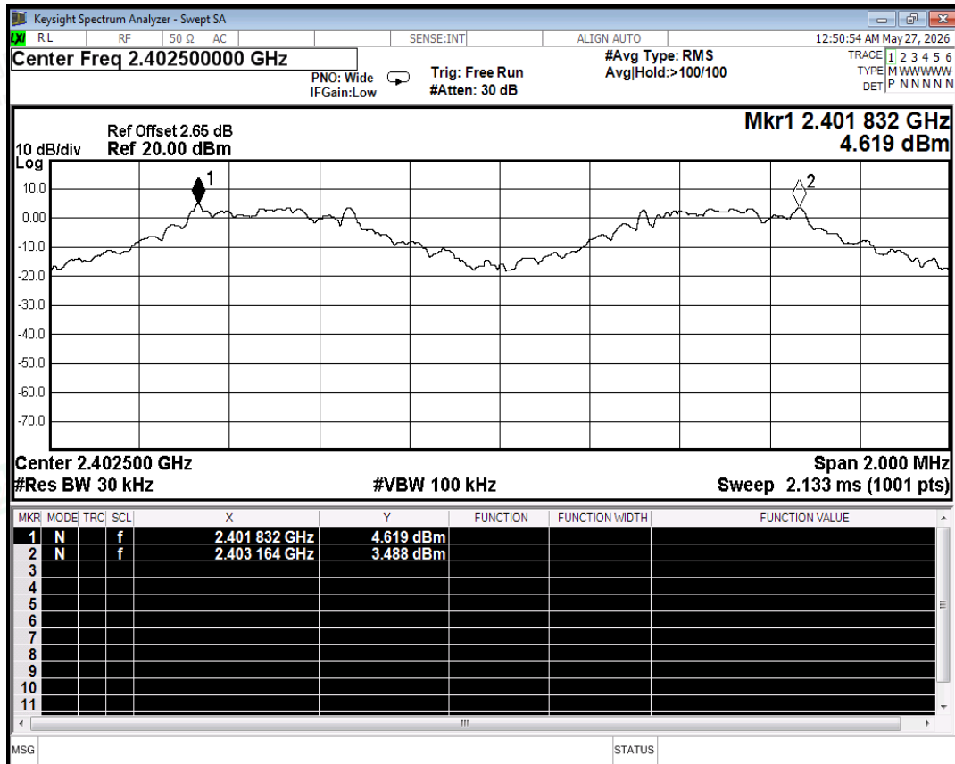
CFS NVNT 1-DH5 2402MHz Ant
