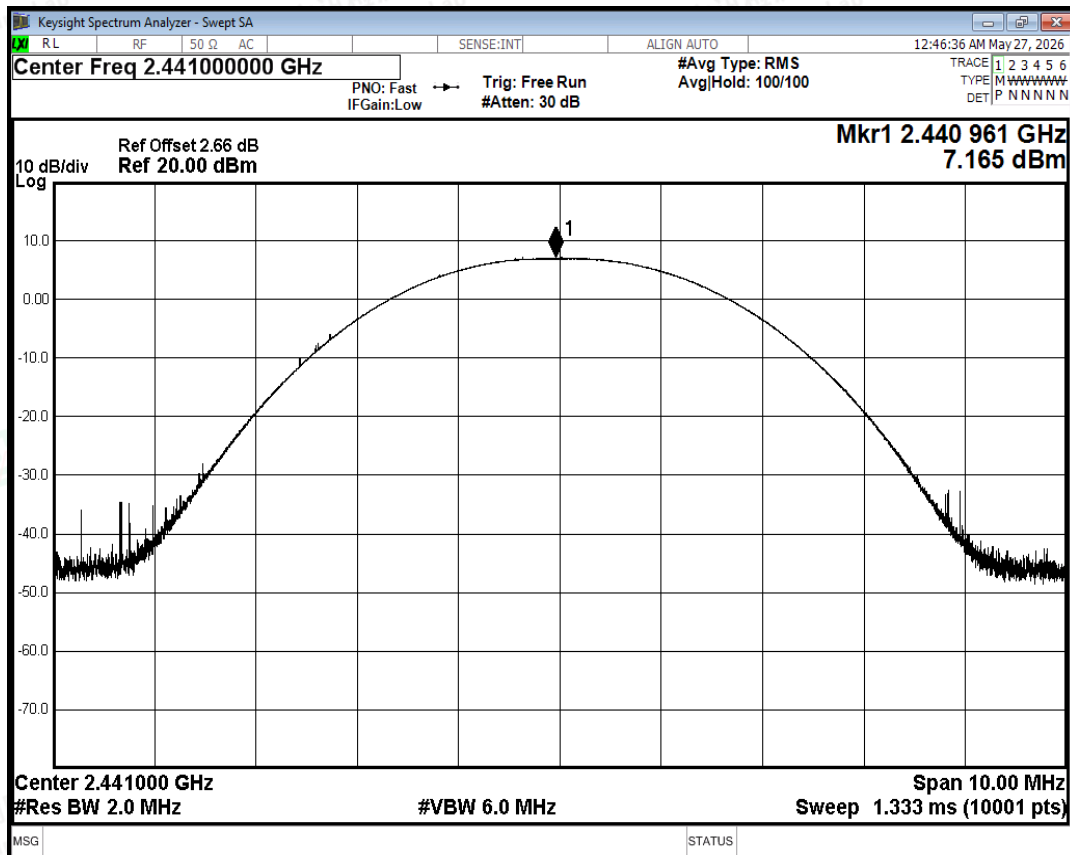
Peak Power NVNT 1-DH5 2441MHz Ant
