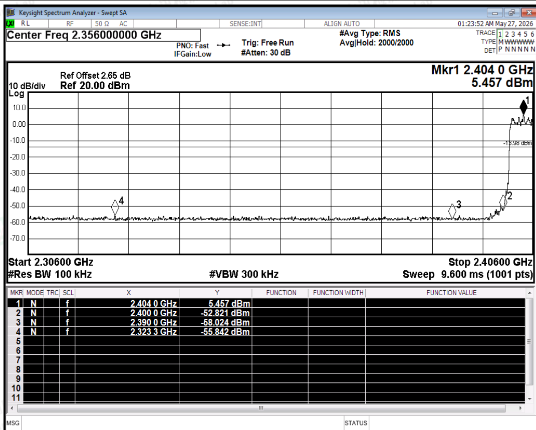
Band Edge(Hopping) NVNT 3-DH5 2402MHz Ant Hopping Emission
