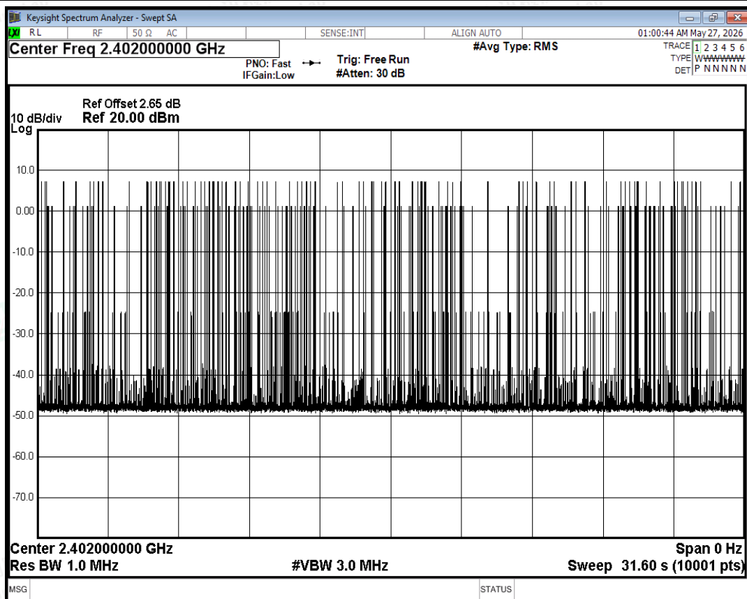
Dwell NVNT 2-DH5 2402MHz Ant Accumulated
