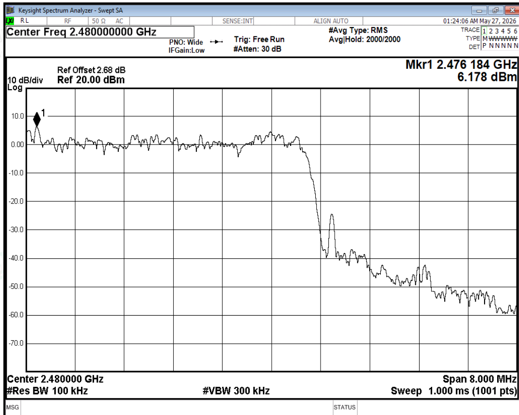
Band Edge(Hopping) NVNT 3-DH5 2480MHz Ant Hopping Ref
