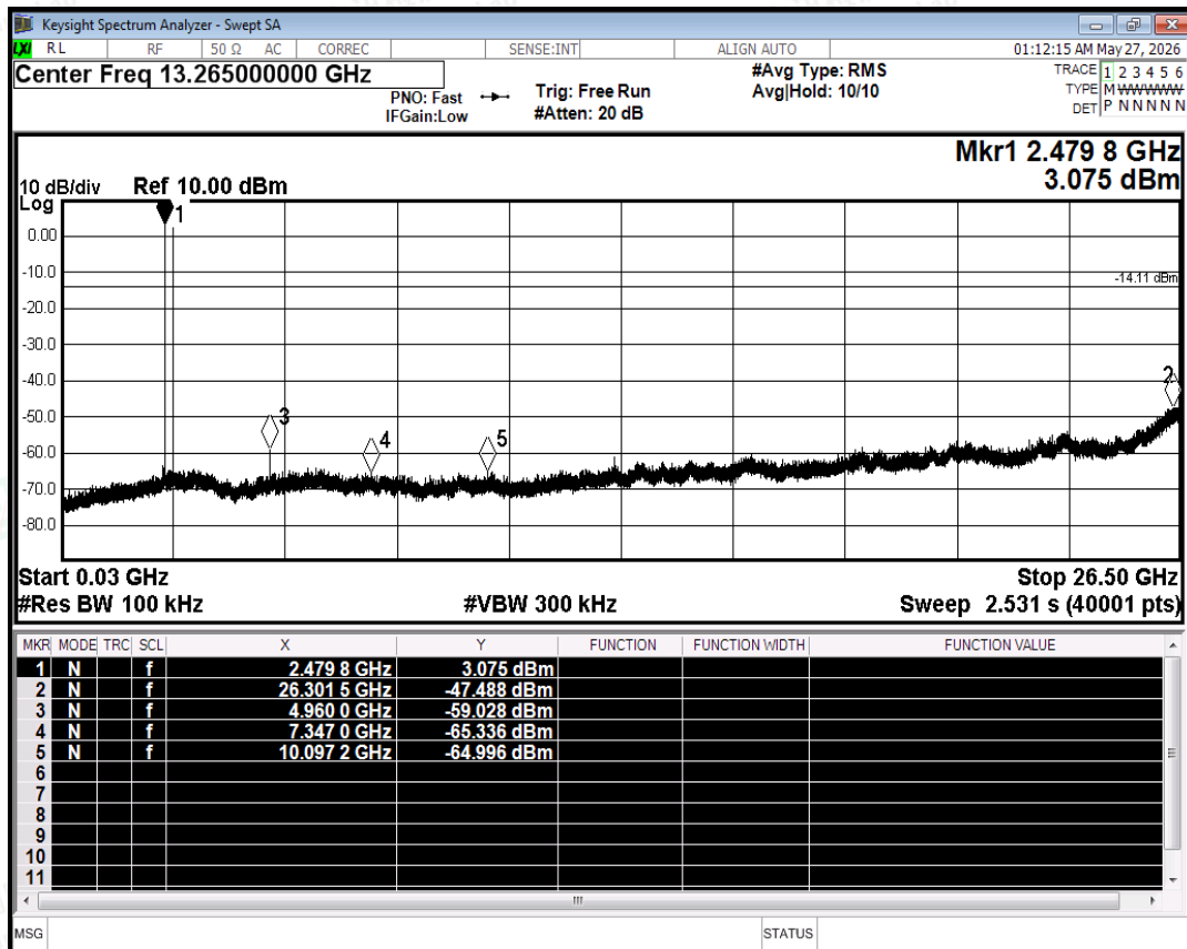
Tx. Spurious NVNT 2-DH5 2480MHz Ant Emission
