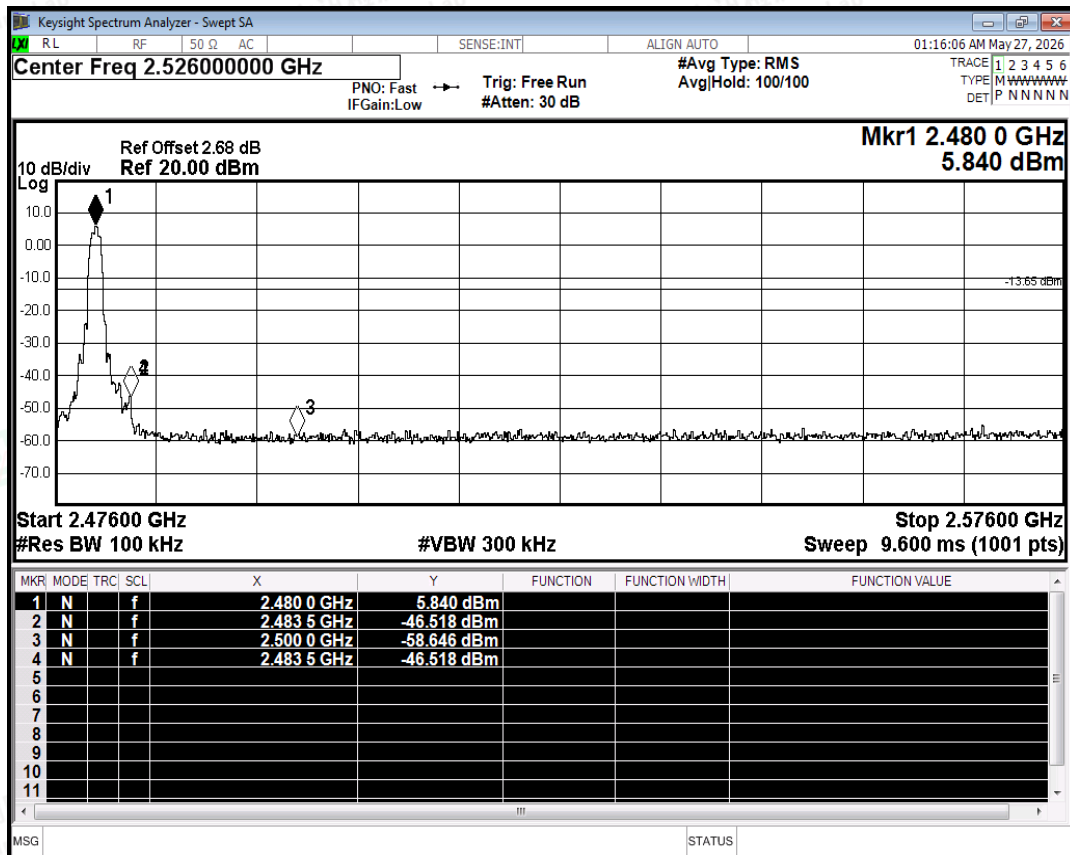
Band Edge NVNT 3-DH5 2480MHz Ant No-Hopping Emission
