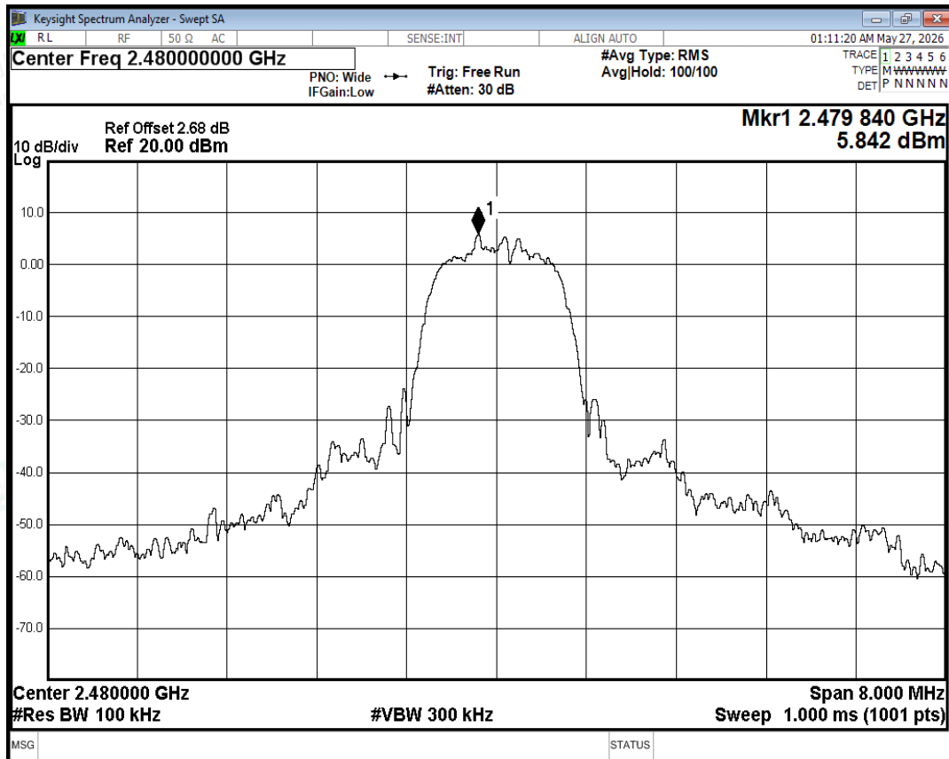
Band Edge NVNT 2-DH5 2480MHz Ant No-Hopping Ref
