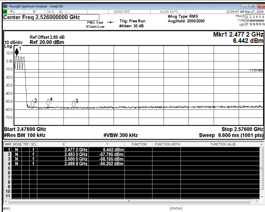
Band Edge(Hopping) NVNT 1-DH5 2480MHz Ant Hopping Emission
