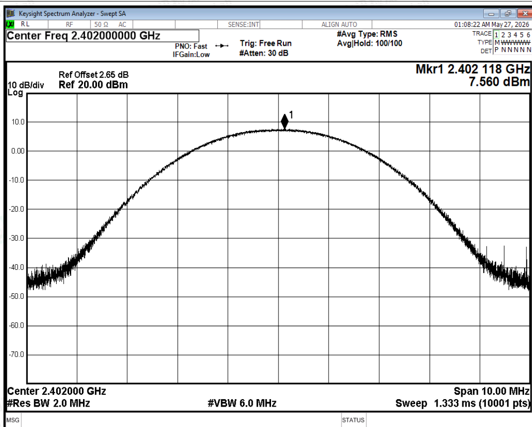
Peak Power NVNT 2-DH5 2402MHz Ant
