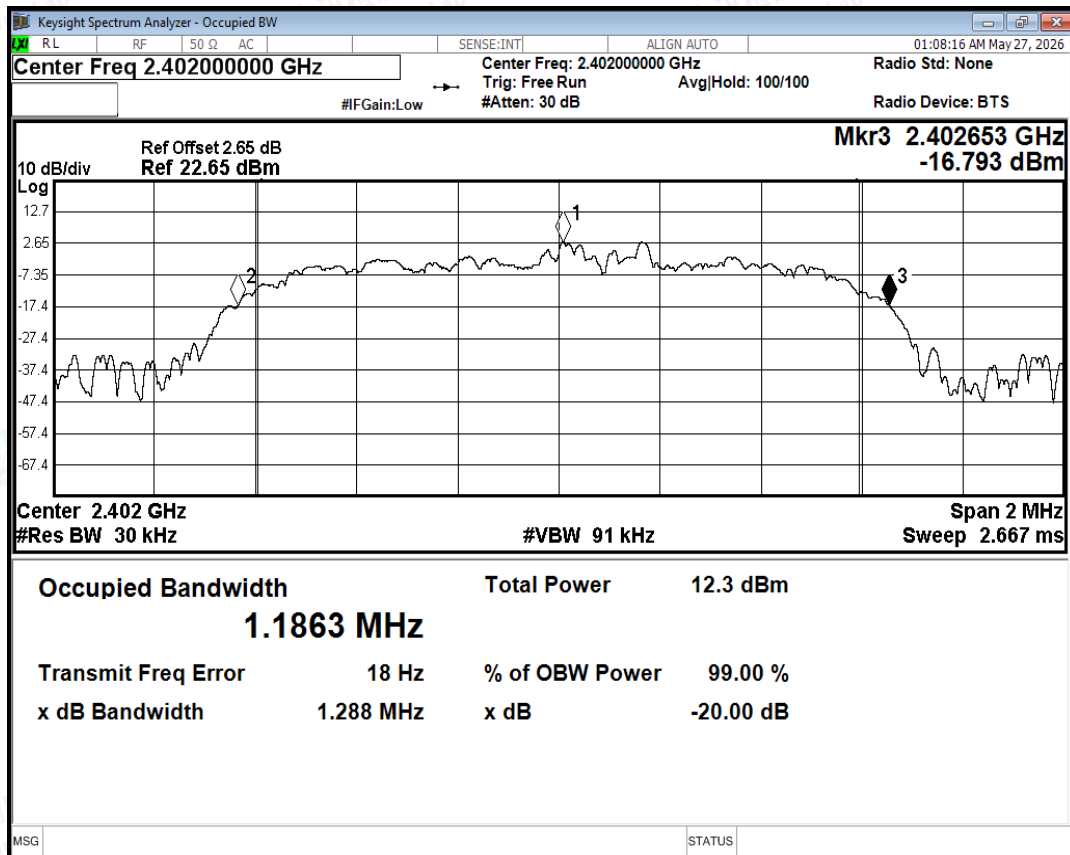
-20dB Bandwidth NVNT 2-DH5 2402MHz Ant
