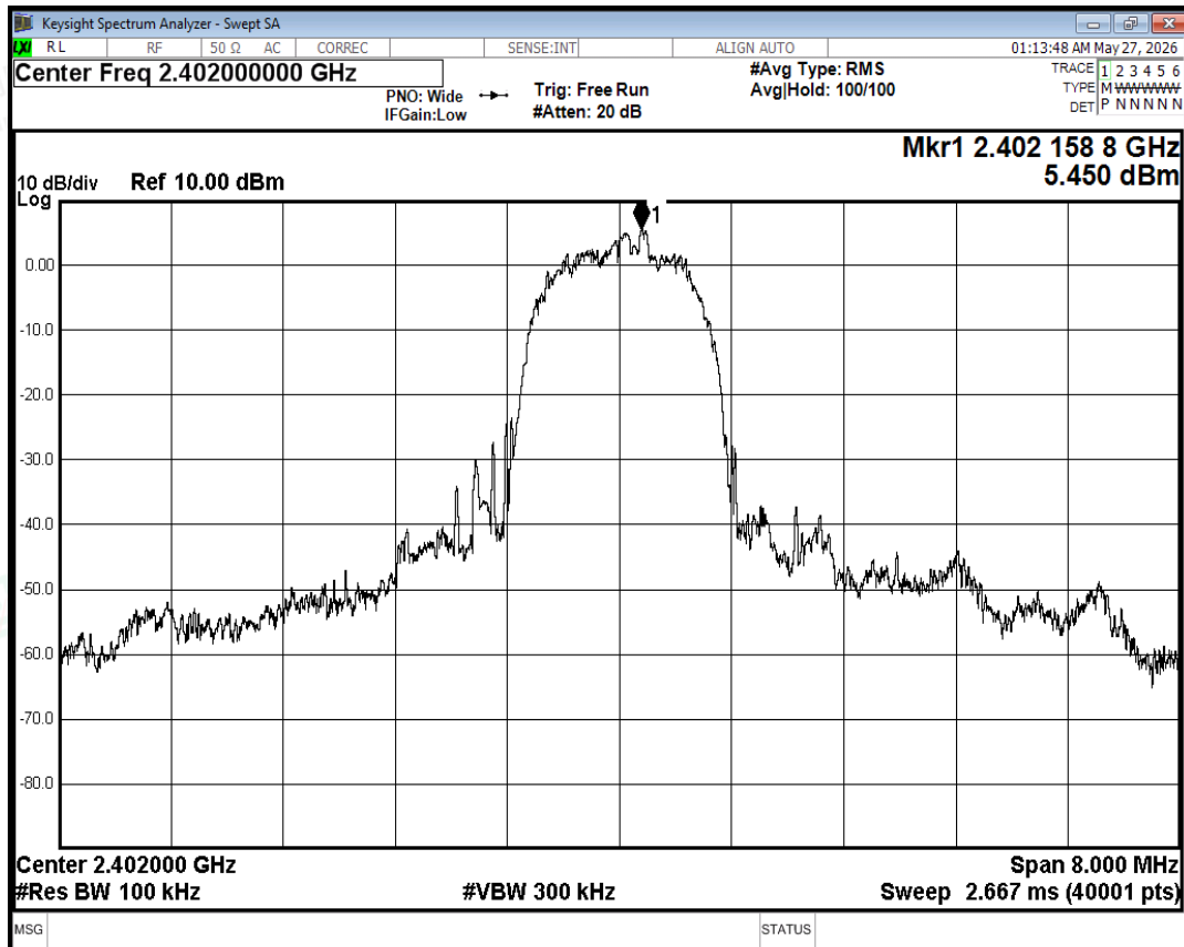
Tx. Spurious NVNT 3-DH5 2402MHz Ant Ref
