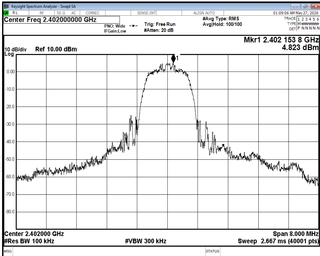
Tx. Spurious NVNT 2-DH5 2402MHz Ant Ref
