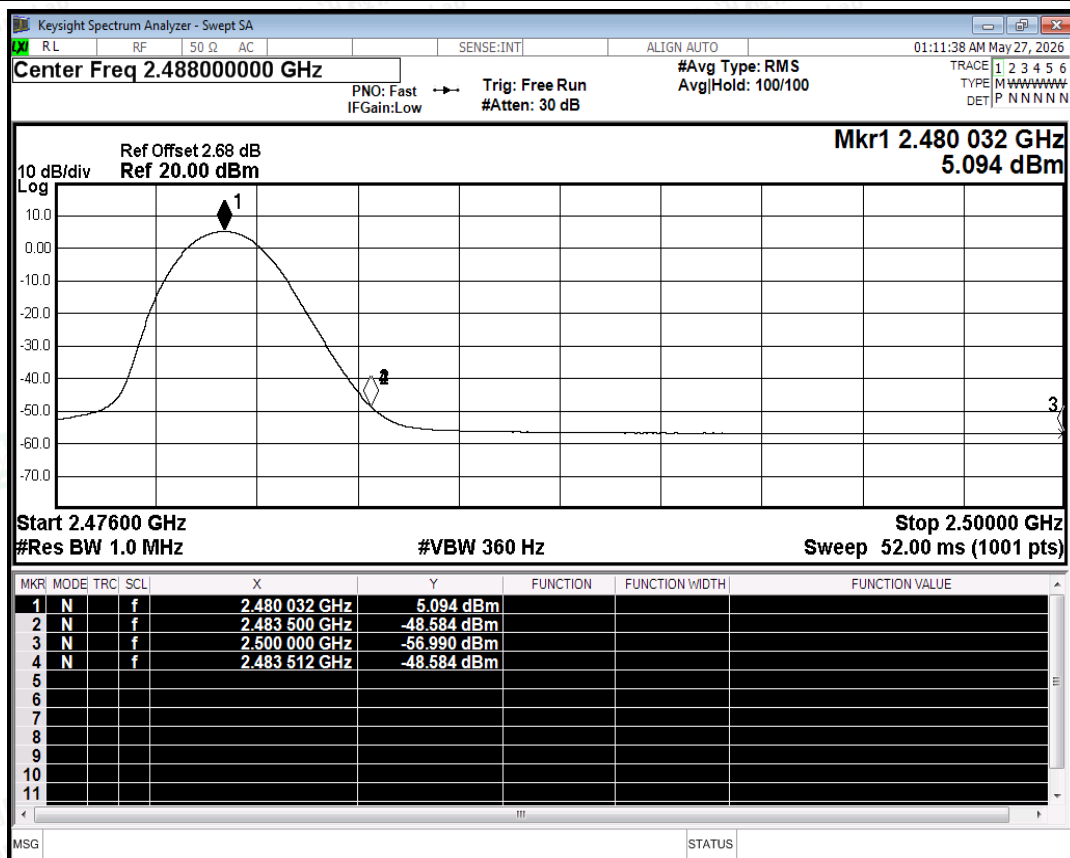
Restrict Band NVNT 2-DH5 2480MHz Ant No-Hopping Average
