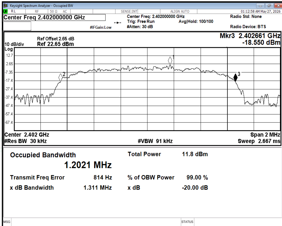
-20dB Bandwidth NVNT 3-DH5 2402MHz Ant
