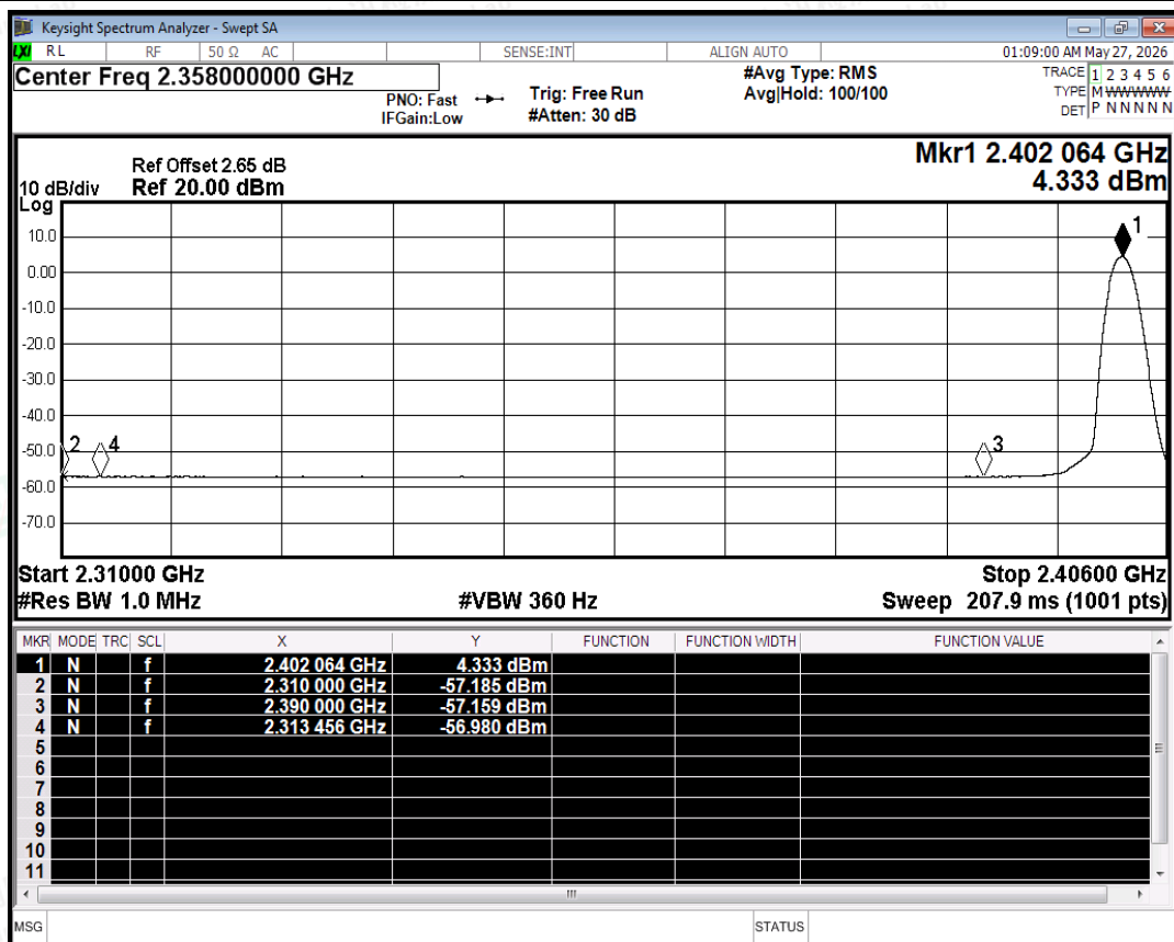
Restrict Band NVNT 2-DH5 2402MHz Ant No-Hopping Average
