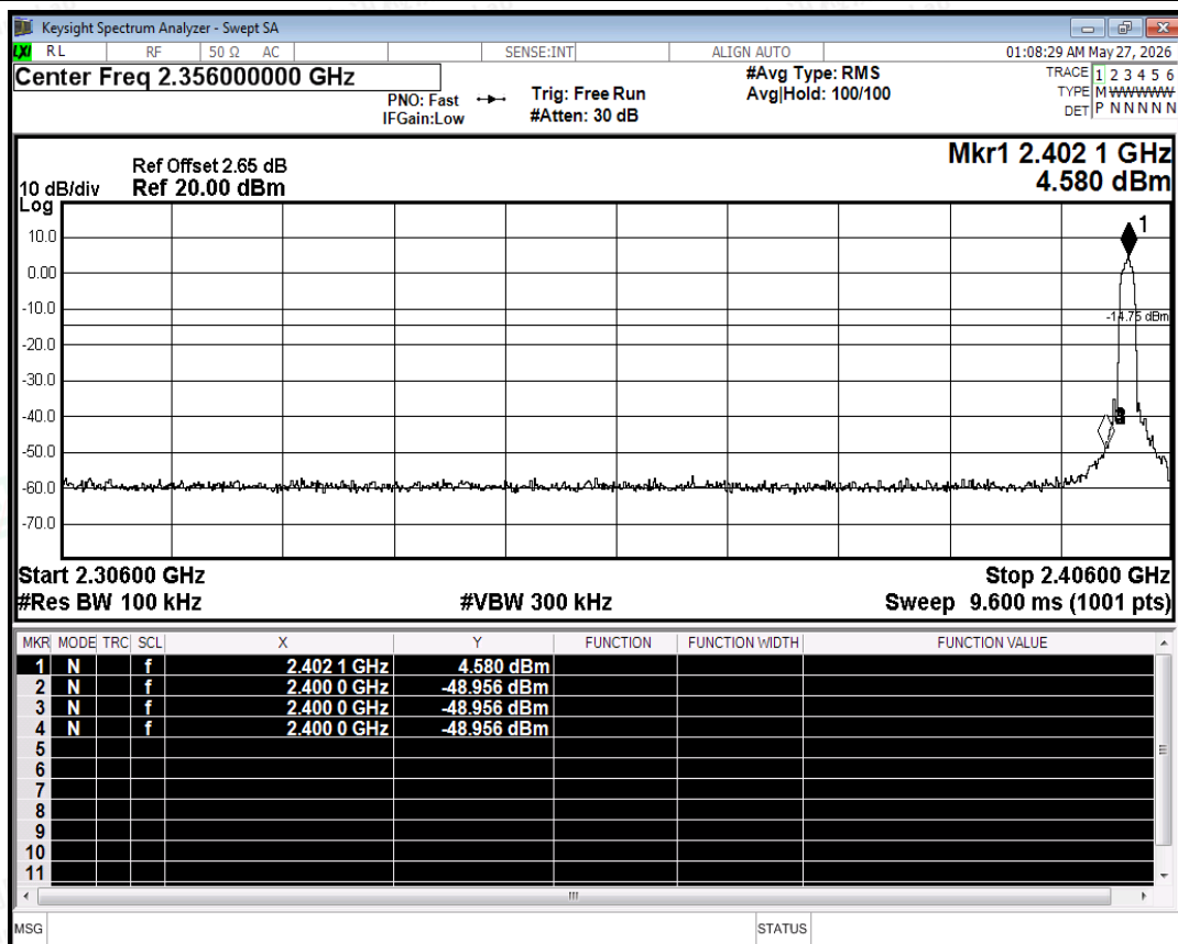
Band Edge NVNT 2-DH5 2402MHz Ant No-Hopping Emission
