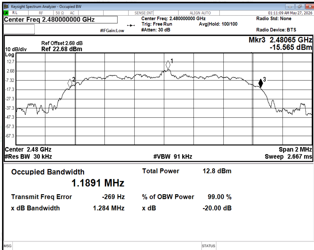
-20dB Bandwidth NVNT 2-DH5 2480MHz Ant
