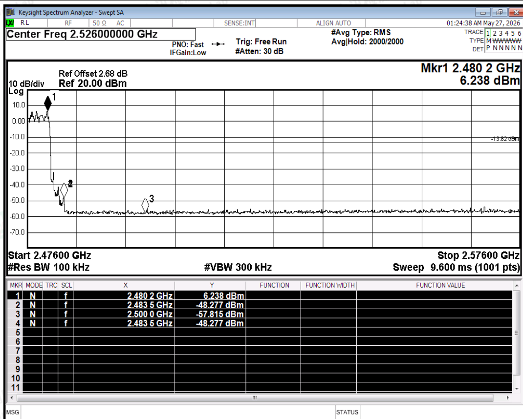
Band Edge(Hopping) NVNT 3-DH5 2480MHz Ant Hopping Emission
