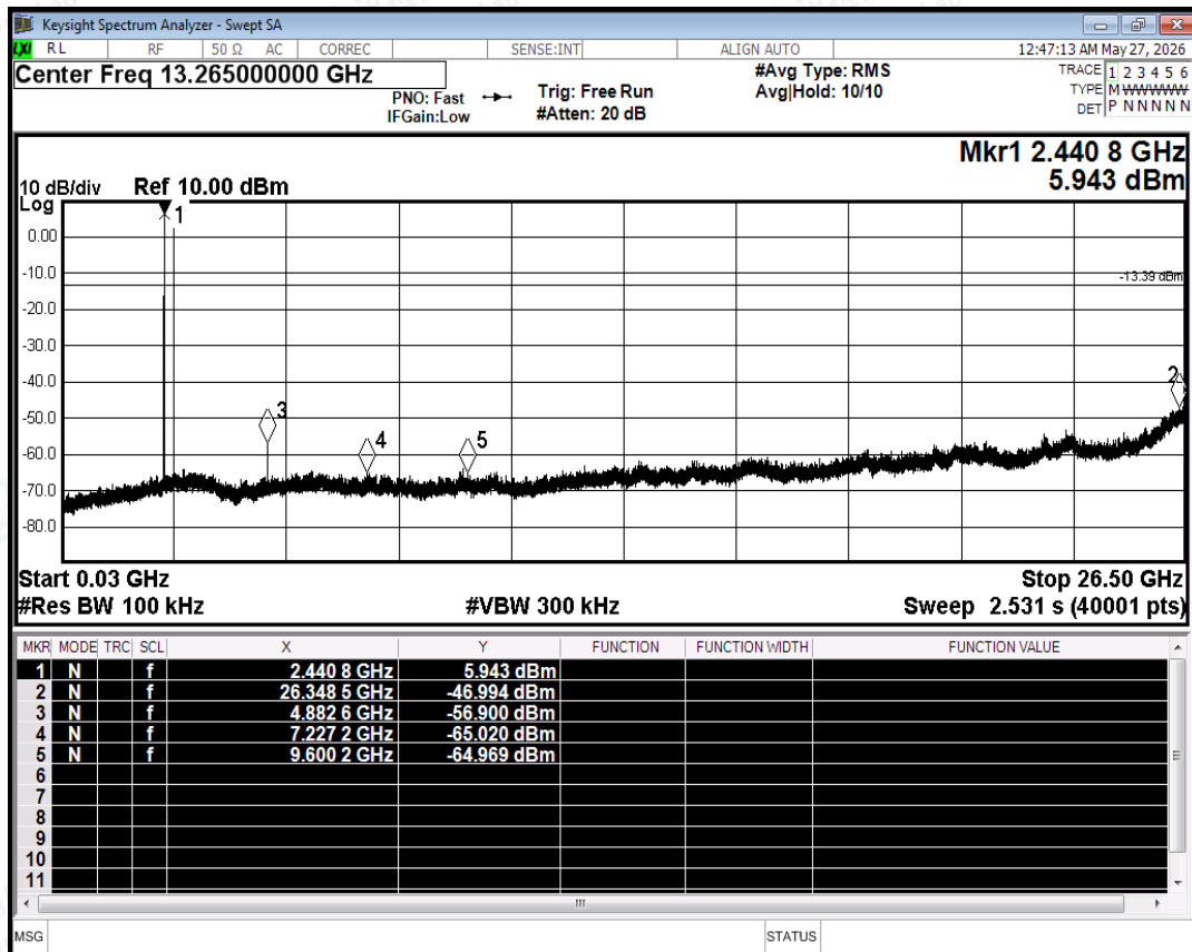
Tx. Spurious NVNT 1-DH5 2441MHz Ant Emission
