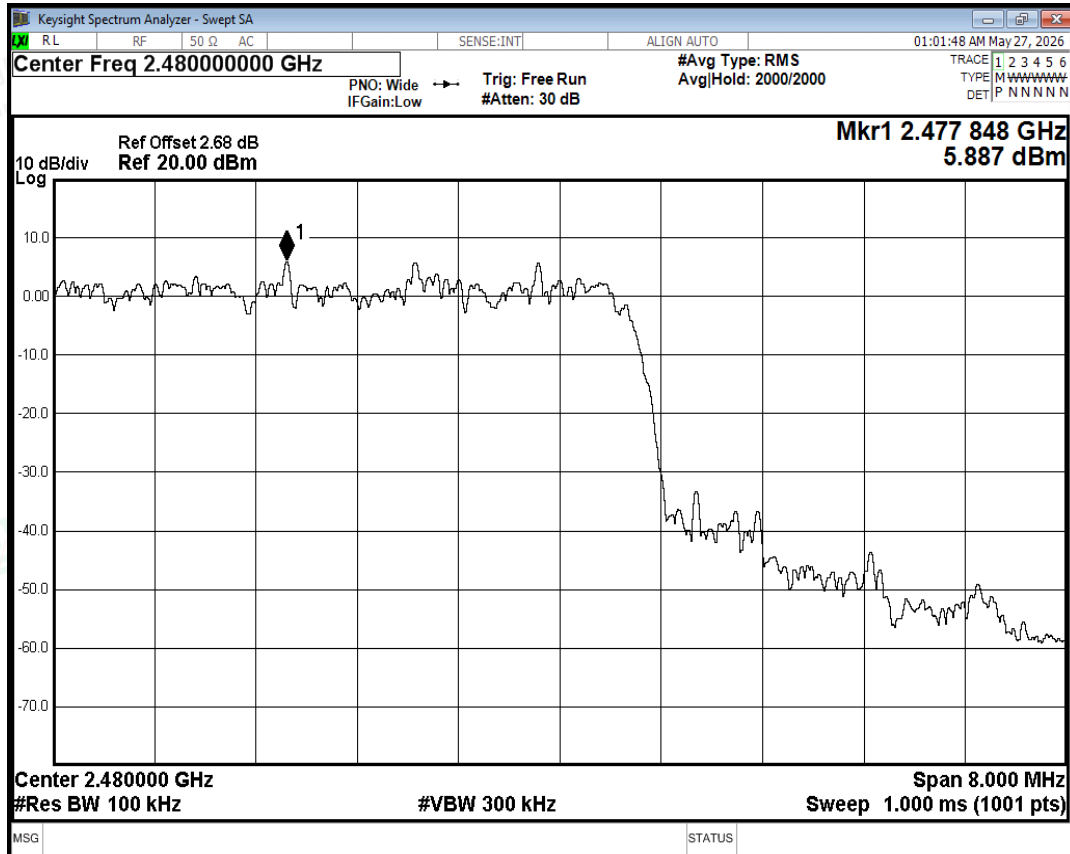
Band Edge(Hopping) NVNT 2-DH5 2480MHz Ant Hopping Ref
