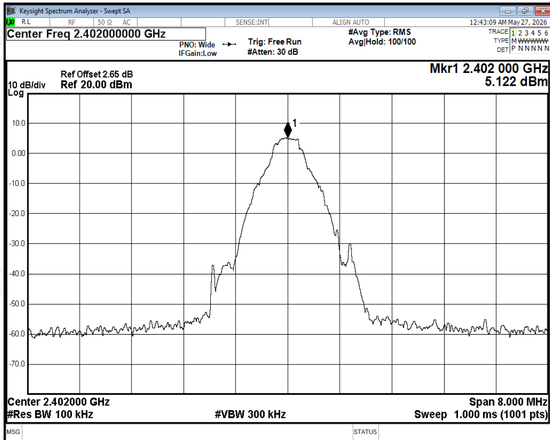
Band Edge NVNT 1-DH5 2402MHz Ant No-Hopping Ref
