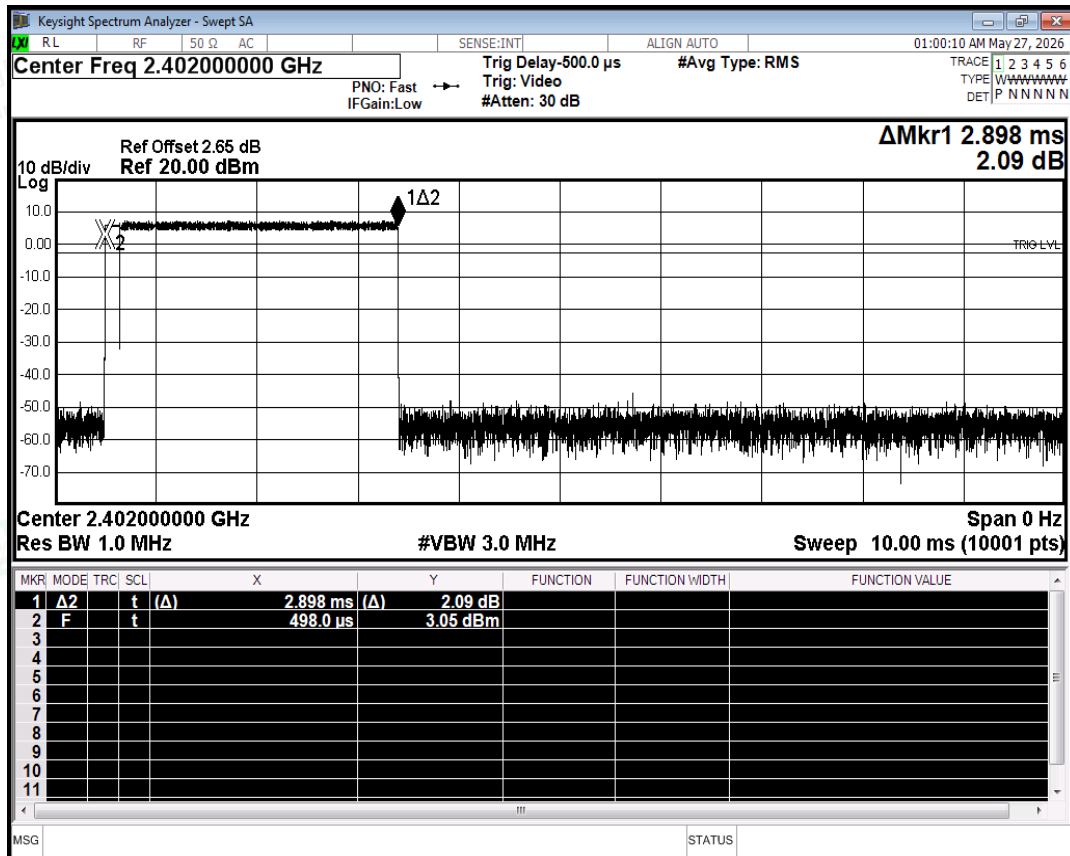
Dwell NVNT 2-DH5 2402MHz Ant One Burst
