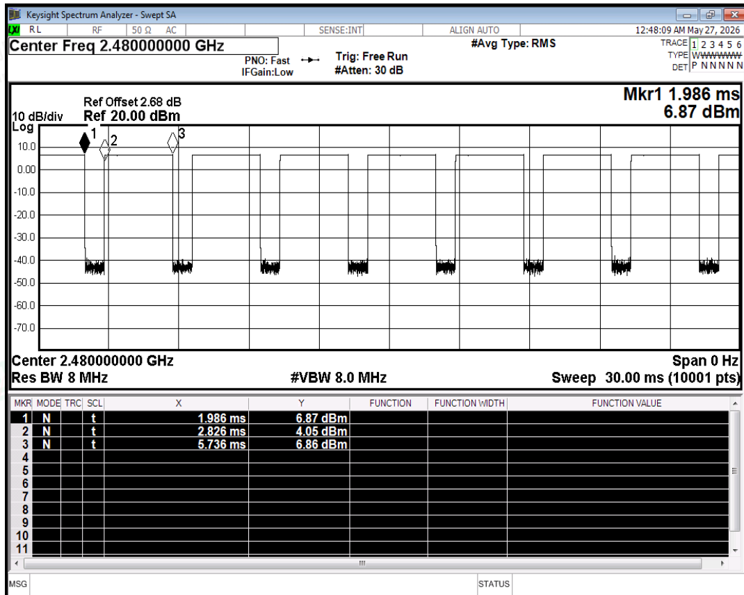
Duty Cycle NVNT 1-DH5 2480MHz Ant
