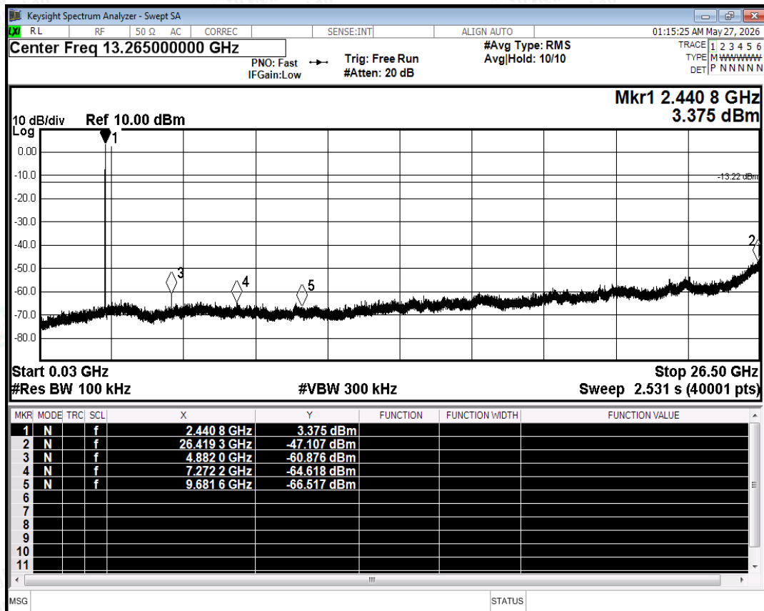
Tx. Spurious NVNT 3-DH5 2441MHz Ant Emission
