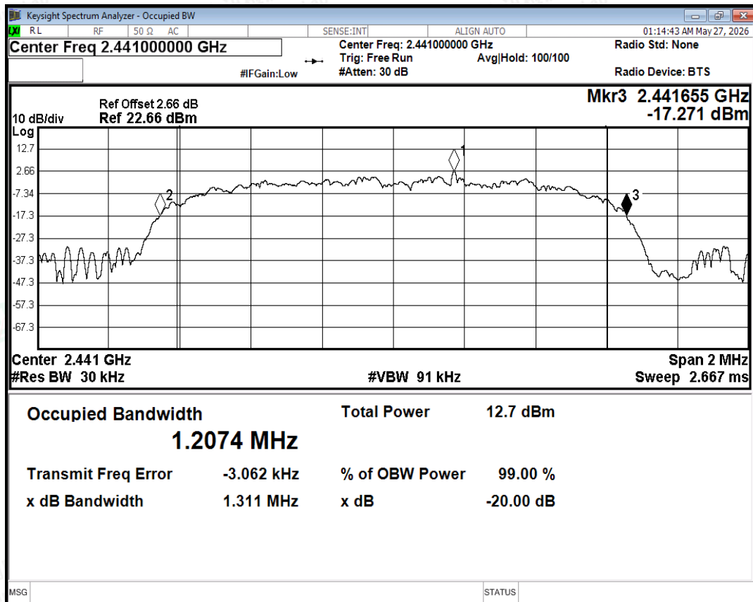
-20dB Bandwidth NVNT 3-DH5 2441MHz Ant
