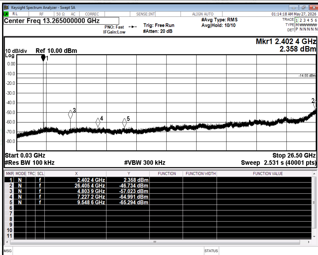
Tx. Spurious NVNT 3-DH5 2402MHz Ant Emission
