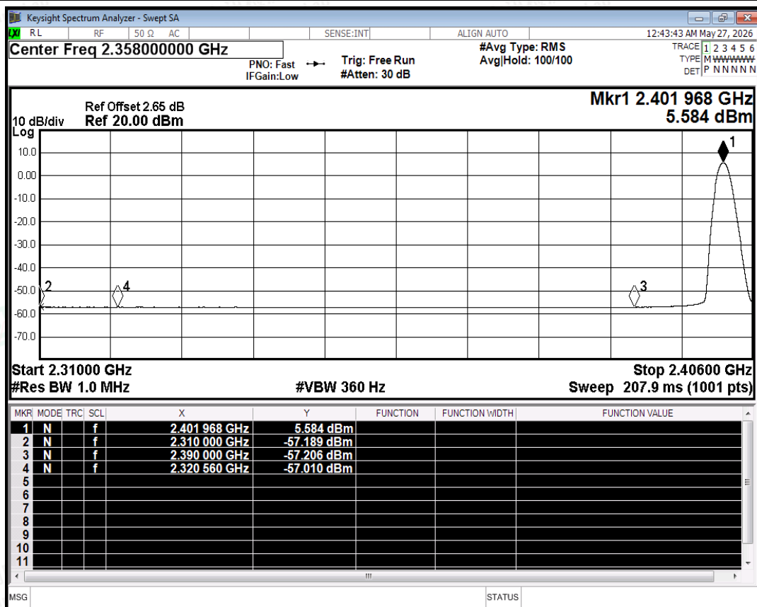
Restrict Band NVNT 1-DH5 2402MHz Ant No-Hopping Average
