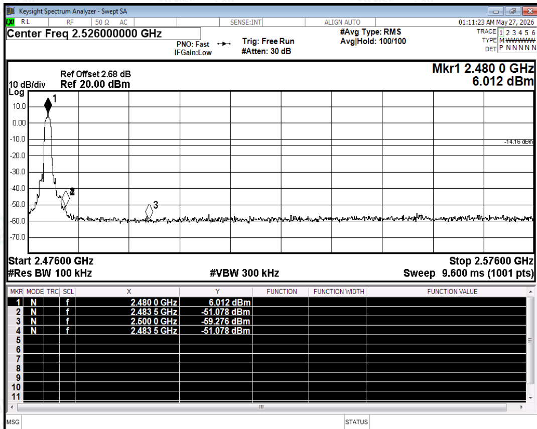
Band Edge NVNT 2-DH5 2480MHz Ant No-Hopping Emission
