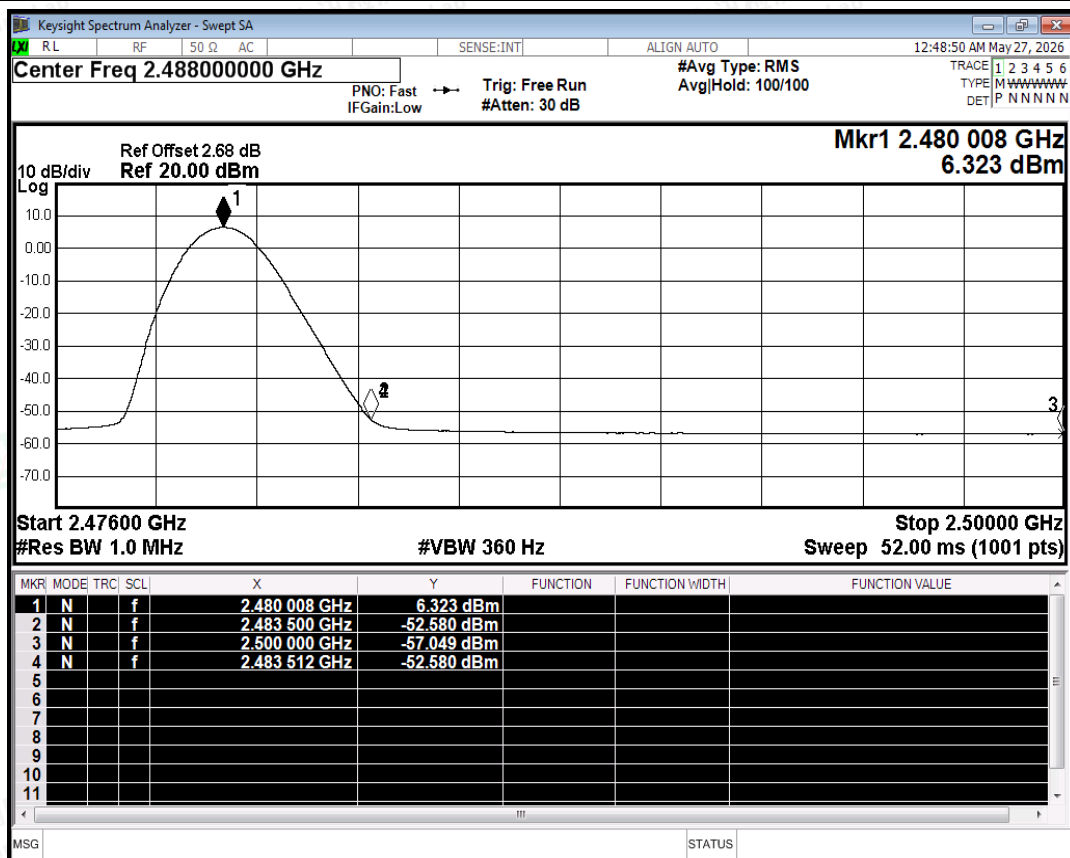
Restrict Band NVNT 1-DH5 2480MHz Ant No-Hopping Average
