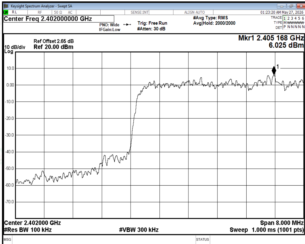
Band Edge(Hopping) NVNT 3-DH5 2402MHz Ant Hopping Ref
