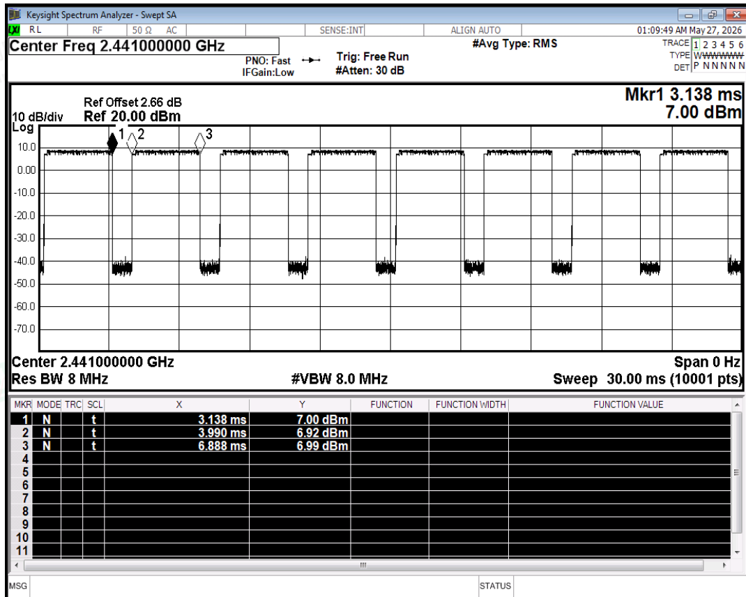
Duty Cycle NVNT 2-DH5 2441MHz Ant
