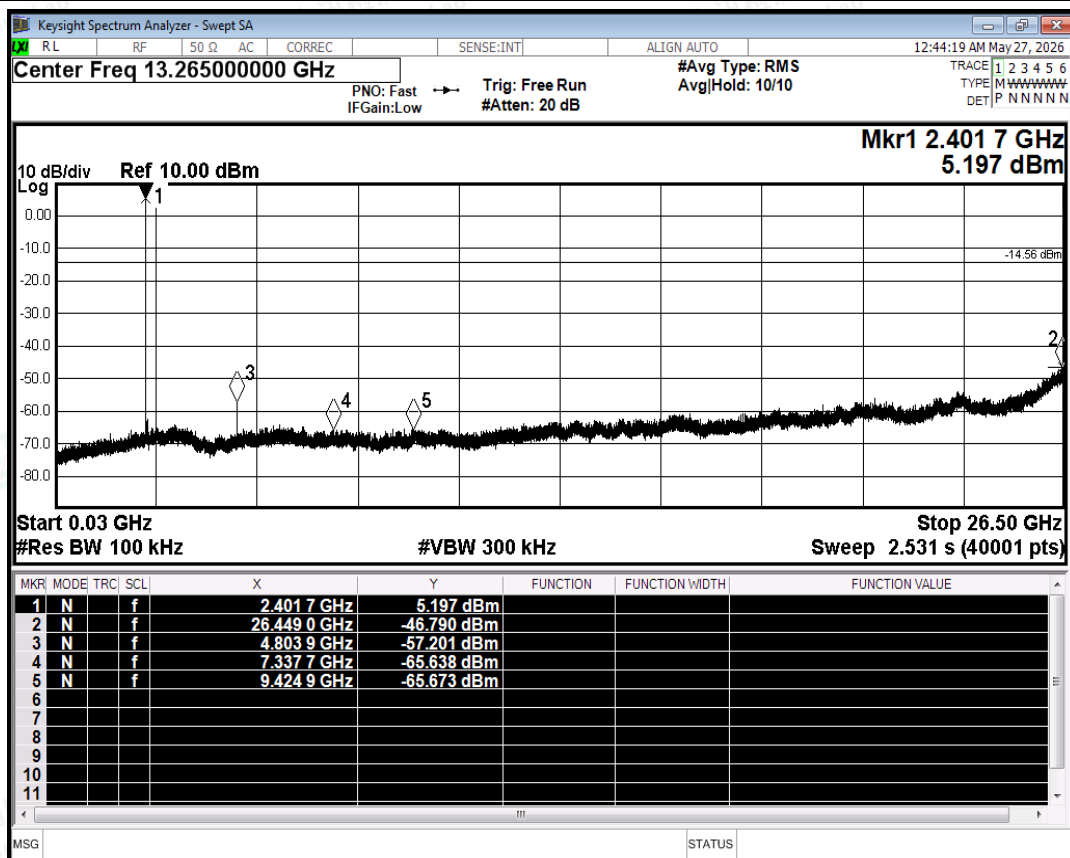
Tx. Spurious NVNT 1-DH5 2402MHz Ant Emission
