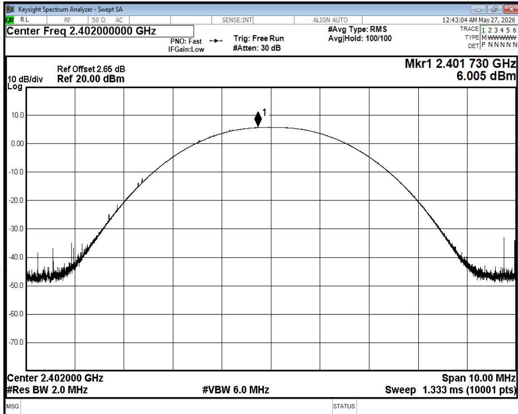
Peak Power NVNT 1-DH5 2402MHz Ant
