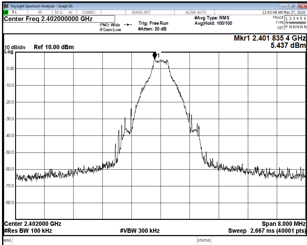
Tx. Spurious NVNT 1-DH5 2402MHz Ant Ref
