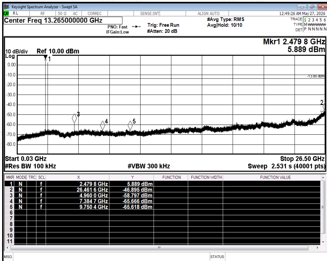
Tx. Spurious NVNT 1-DH5 2480MHz Ant Emission
