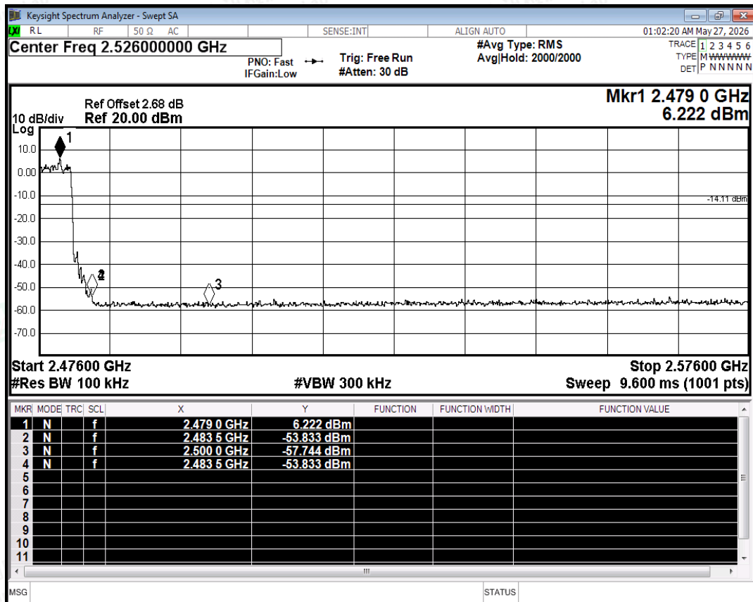
Band Edge(Hopping) NVNT 2-DH5 2480MHz Ant Hopping Emission
