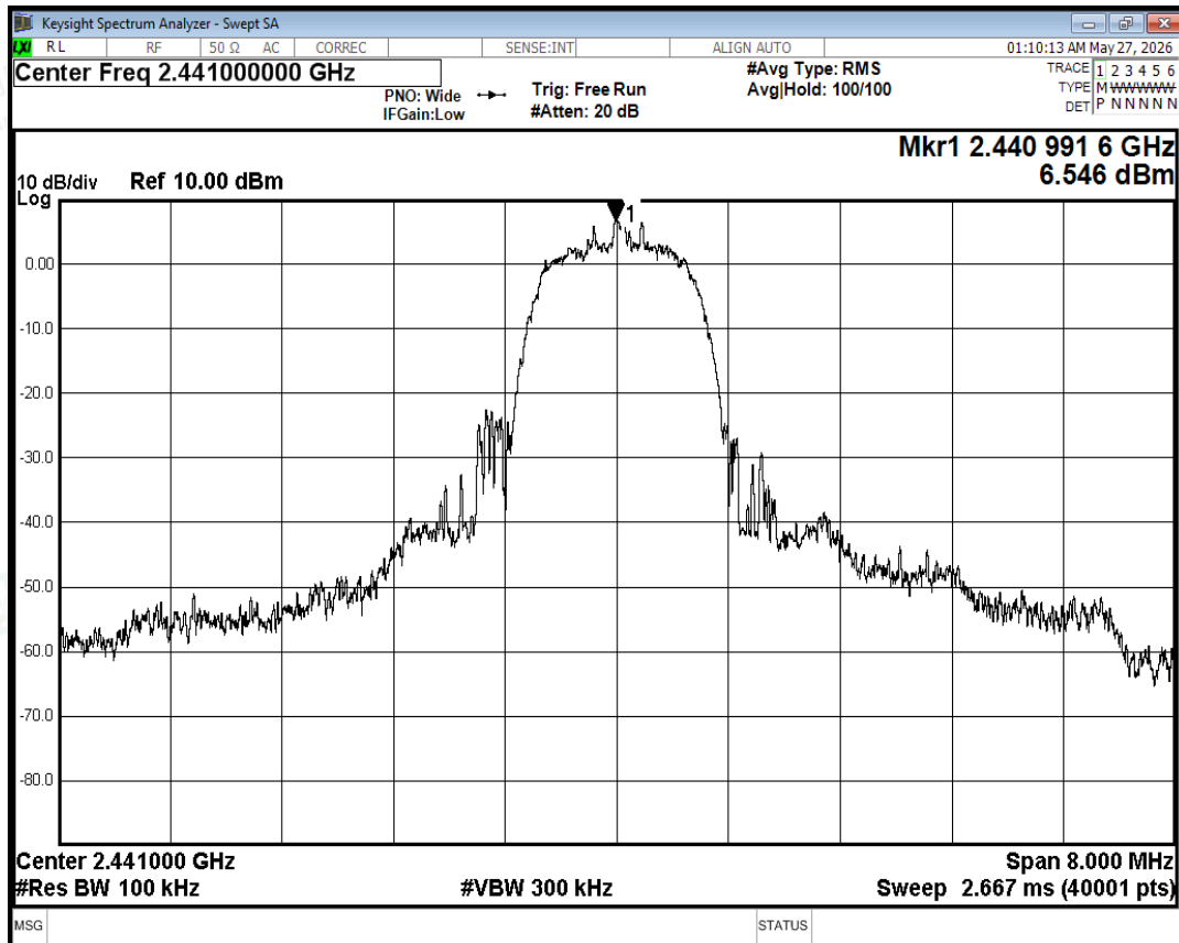
Tx. Spurious NVNT 2-DH5 2441MHz Ant Ref
