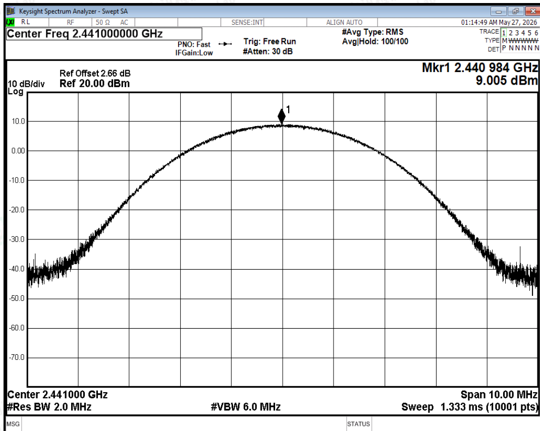
Peak Power NVNT 3-DH5 2441MHz Ant
