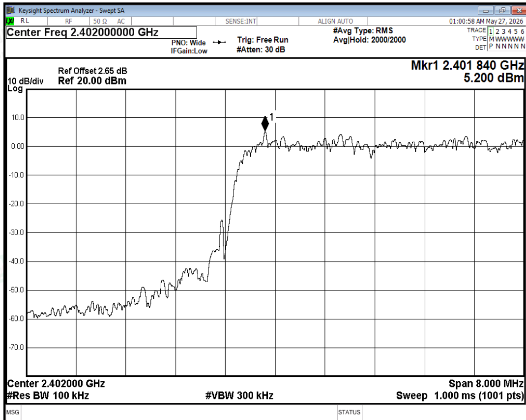
Band Edge(Hopping) NVNT 2-DH5 2402MHz Ant Hopping Ref
