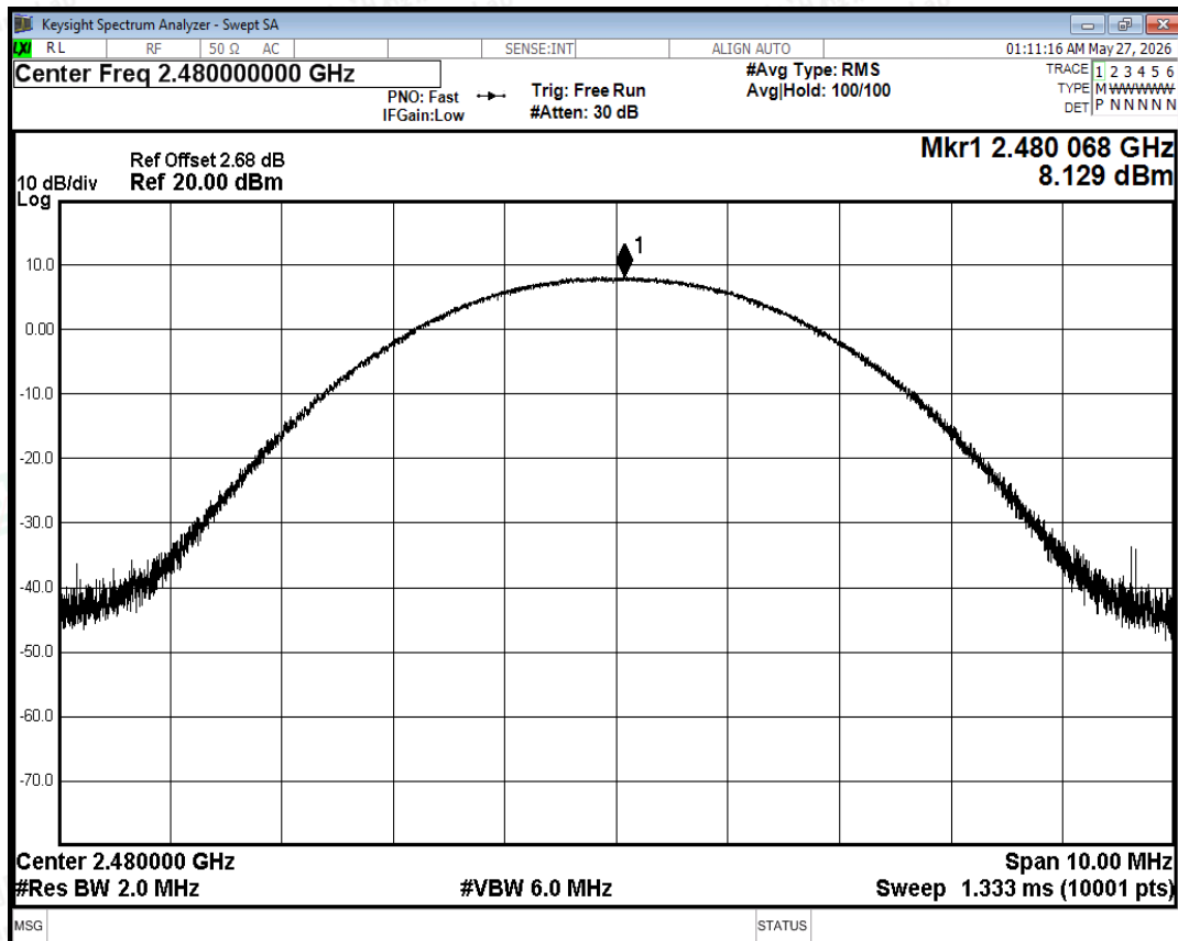
Peak Power NVNT 2-DH5 2480MHz Ant
