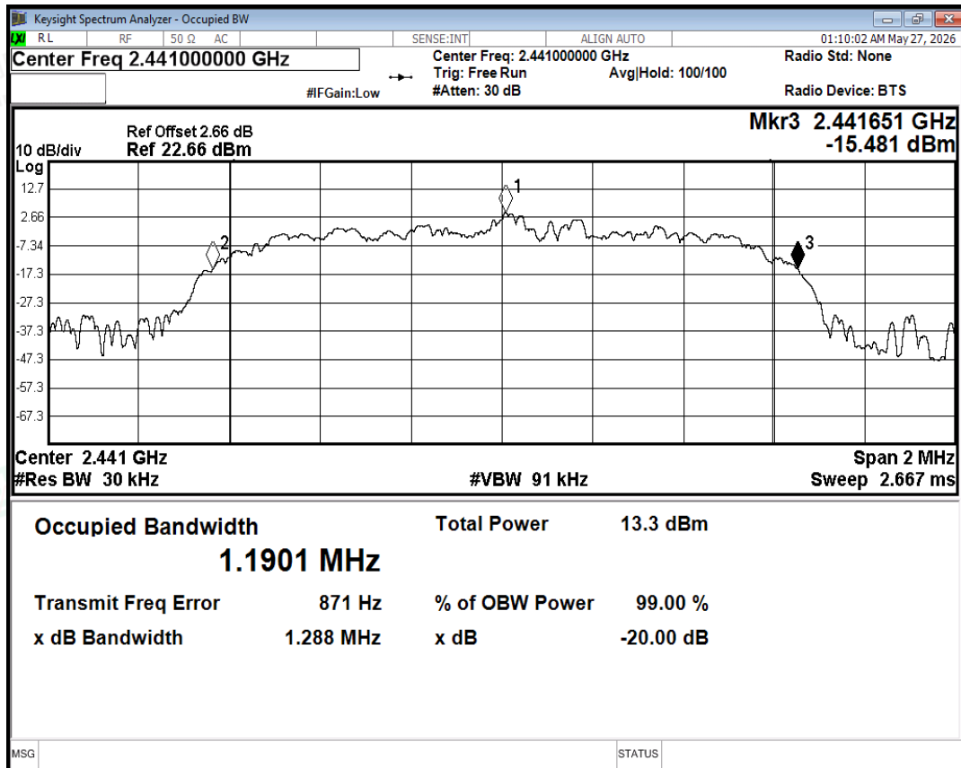
-20dB Bandwidth NVNT 2-DH5 2441MHz Ant
