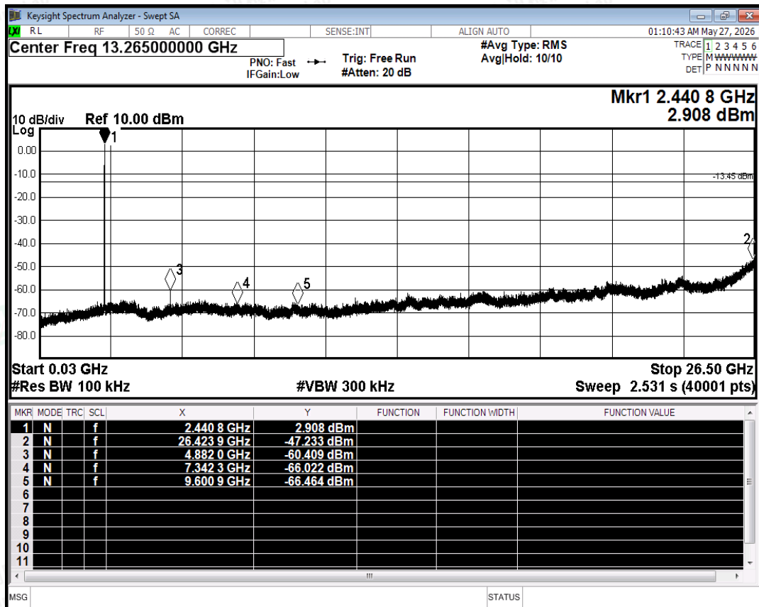
Tx. Spurious NVNT 2-DH5 2441MHz Ant Emission
