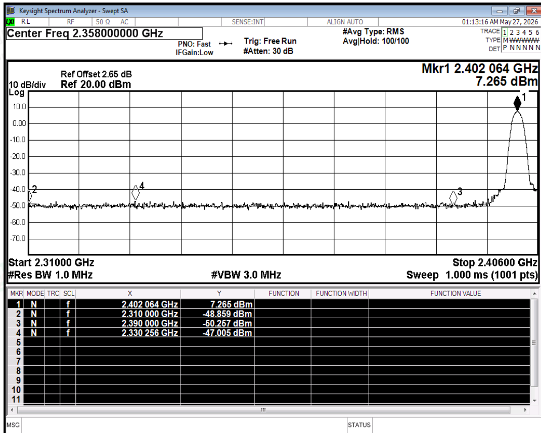
Restrict Band NVNT 3-DH5 2402MHz Ant No-Hopping Peak
