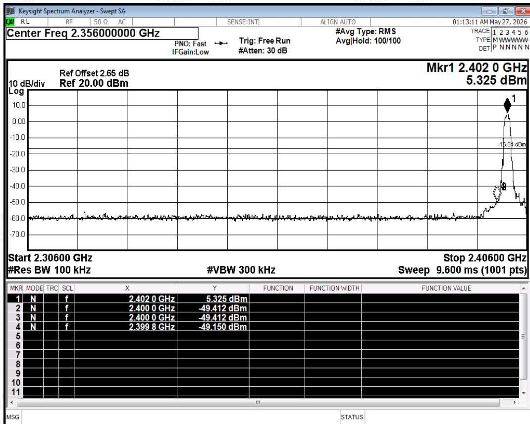
Band Edge NVNT 3-DH5 2402MHz Ant No-Hopping Emission
