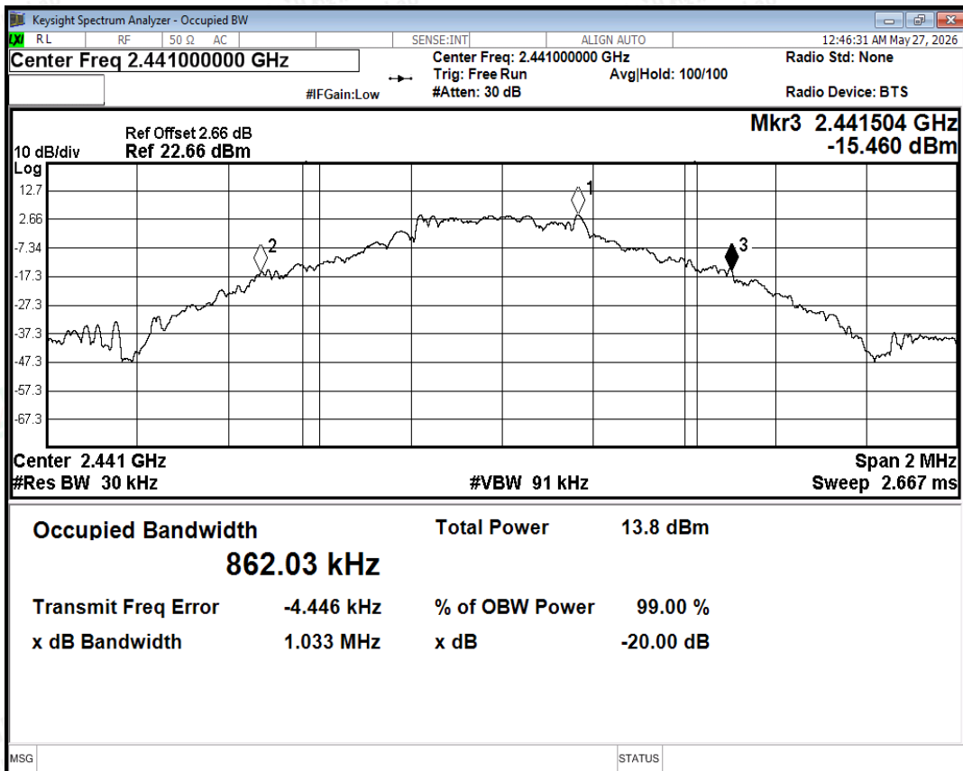
-20dB Bandwidth NVNT 1-DH5 2441MHz Ant
