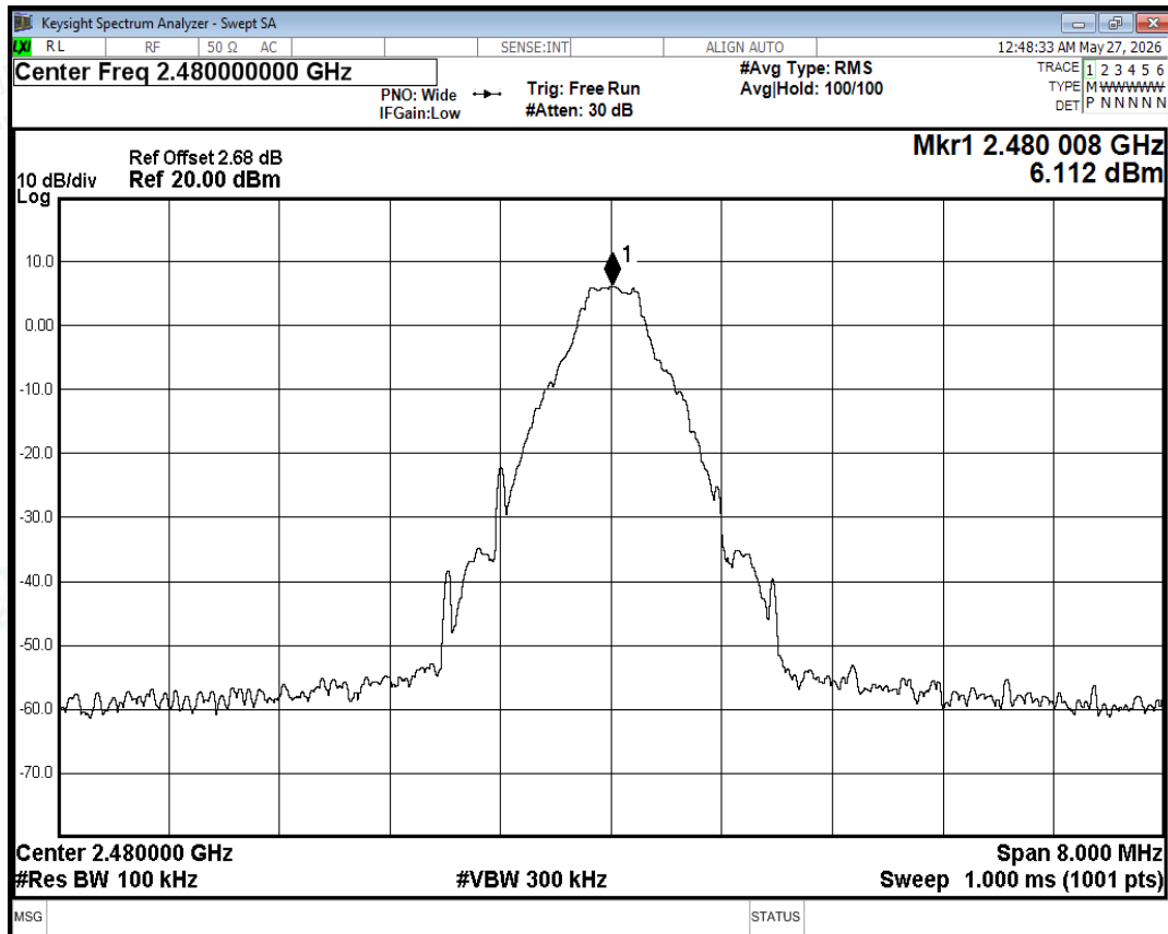
Band Edge NVNT 1-DH5 2480MHz Ant No-Hopping Ref
