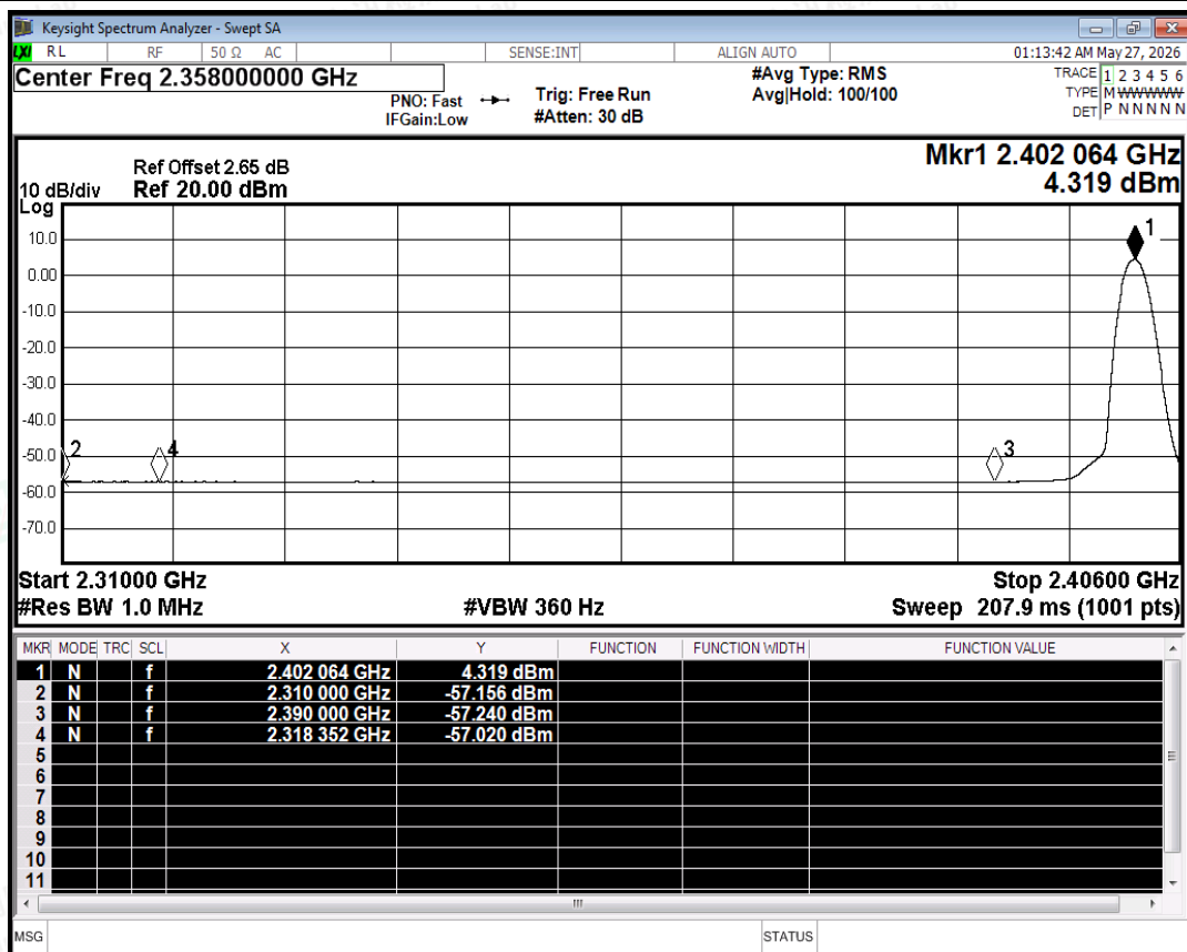
Restrict Band NVNT 3-DH5 2402MHz Ant No-Hopping Average
