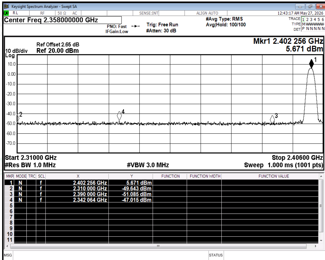
Restrict Band NVNT 1-DH5 2402MHz Ant No-Hopping Peak
