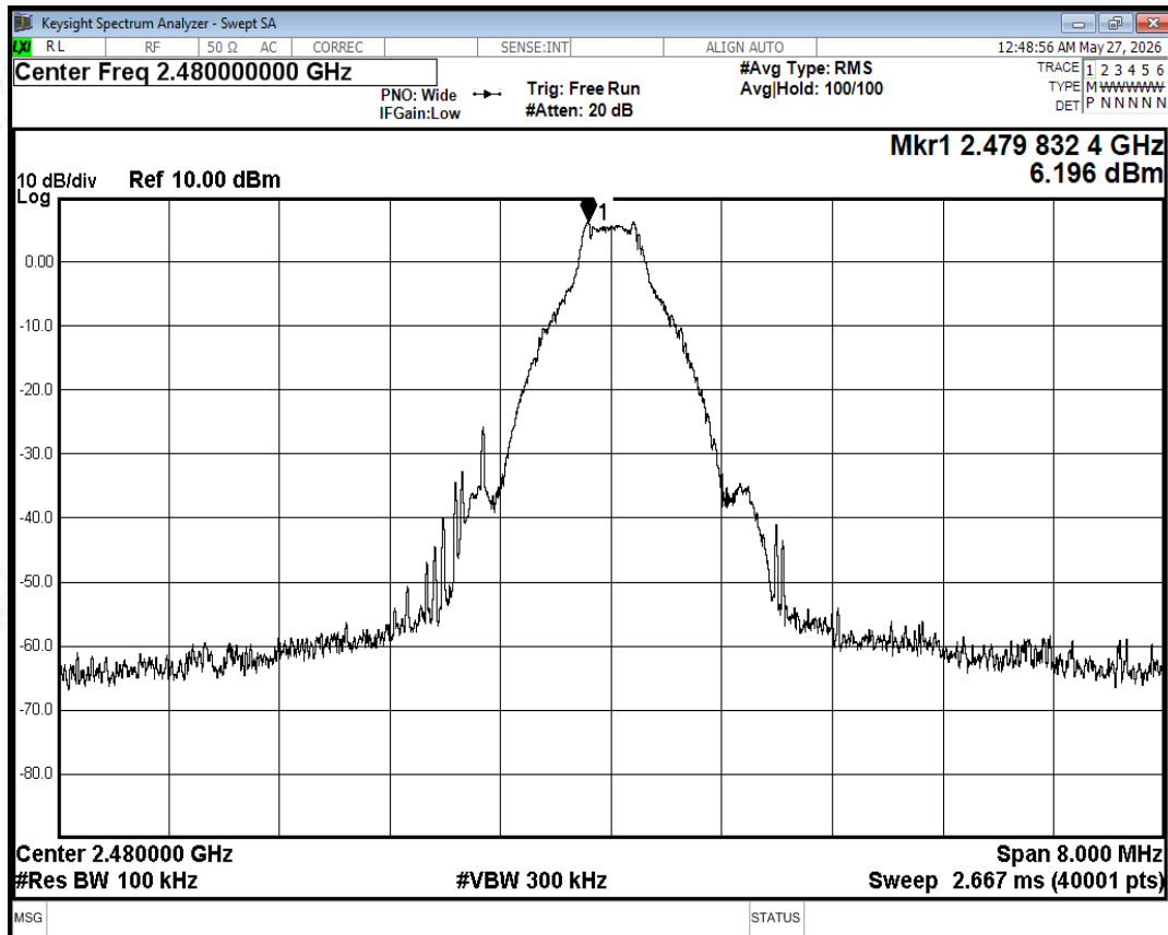
Tx. Spurious NVNT 1-DH5 2480MHz Ant Ref
