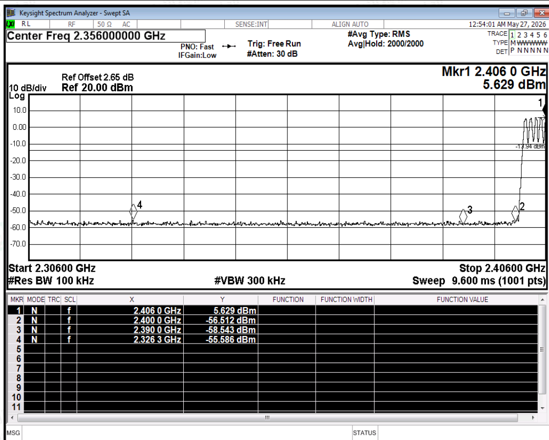
Band Edge(Hopping) NVNT 1-DH5 2402MHz Ant Hopping Emission
