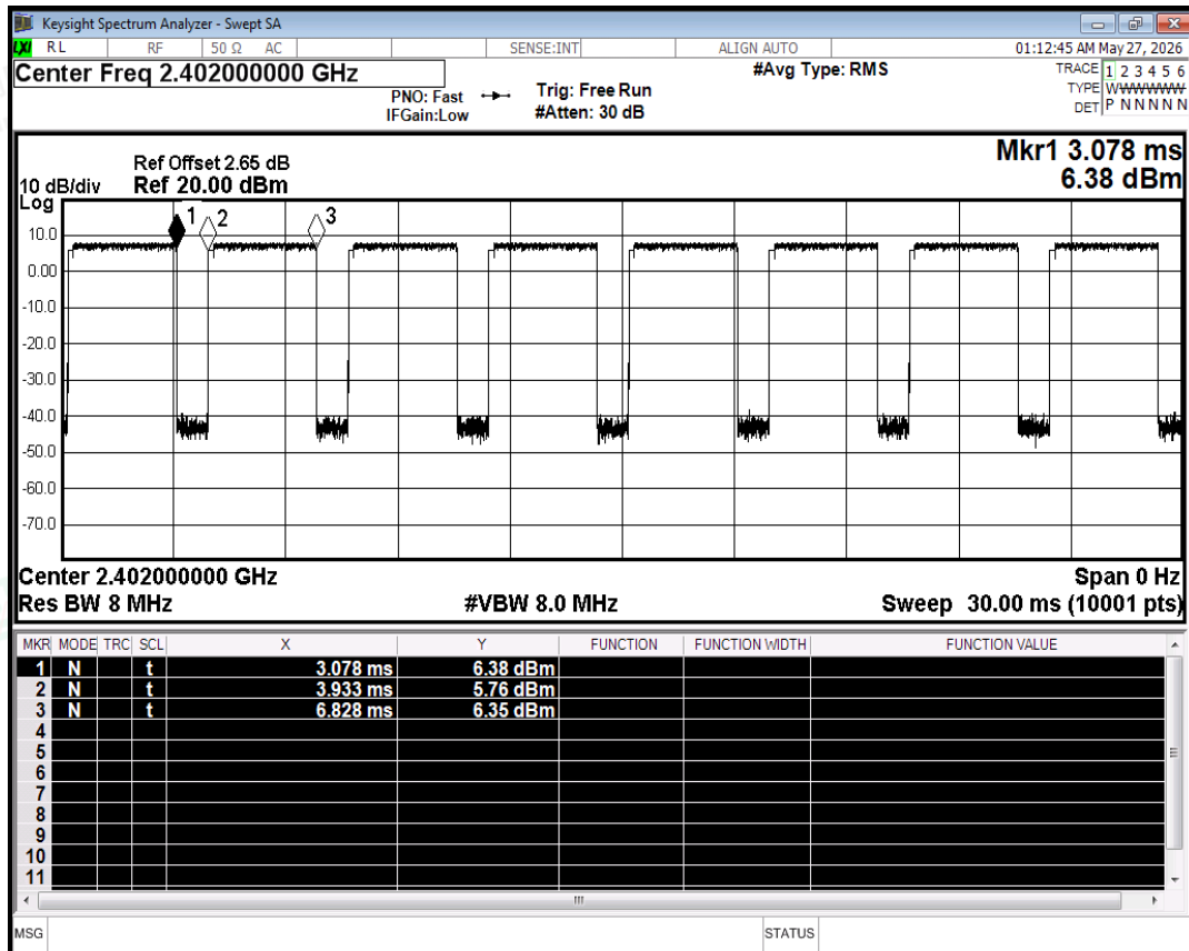
Duty Cycle NVNT 3-DH5 2402MHz Ant
