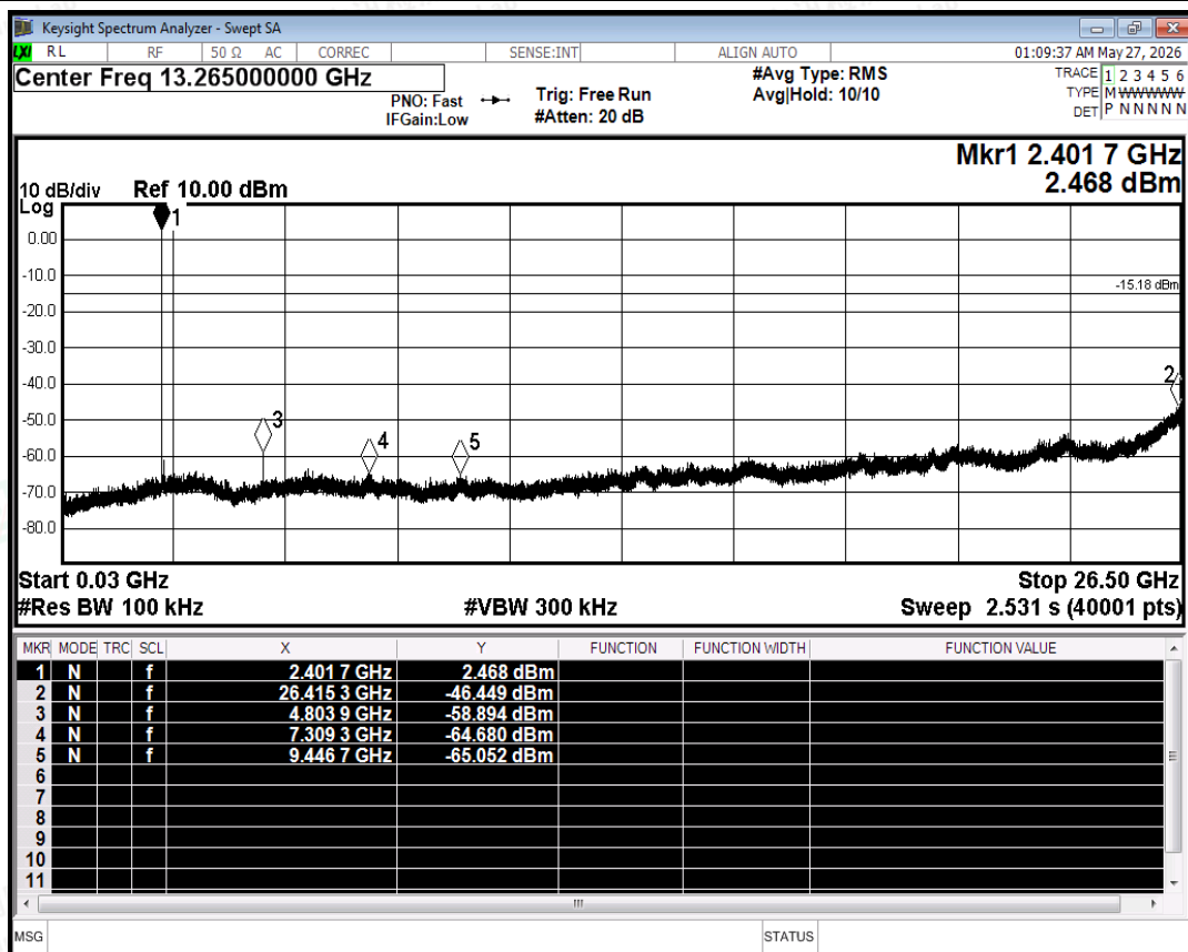
Tx. Spurious NVNT 2-DH5 2402MHz Ant Emission
