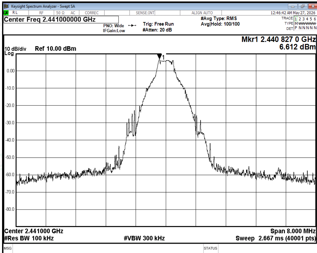
Tx. Spurious NVNT 1-DH5 2441MHz Ant Ref
