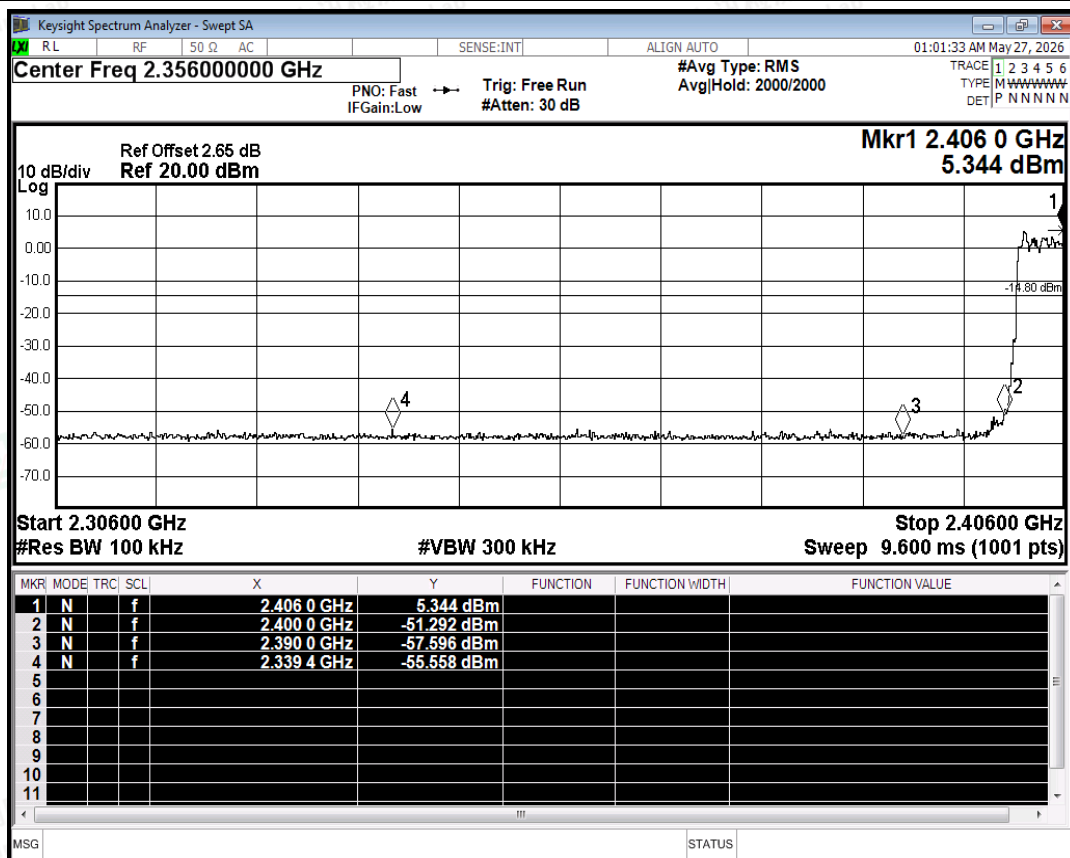
Band Edge(Hopping) NVNT 2-DH5 2402MHz Ant Hopping Emission
