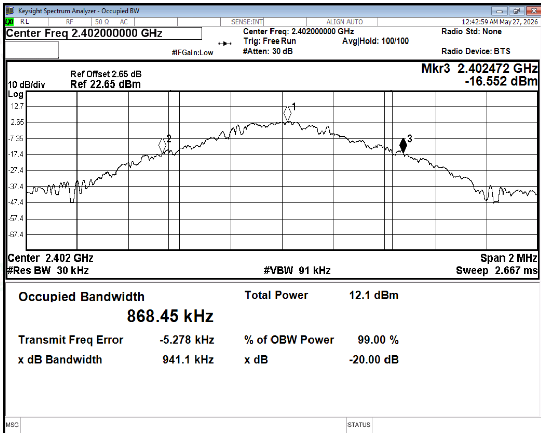
-20dB Bandwidth NVNT 1-DH5 2402MHz Ant
