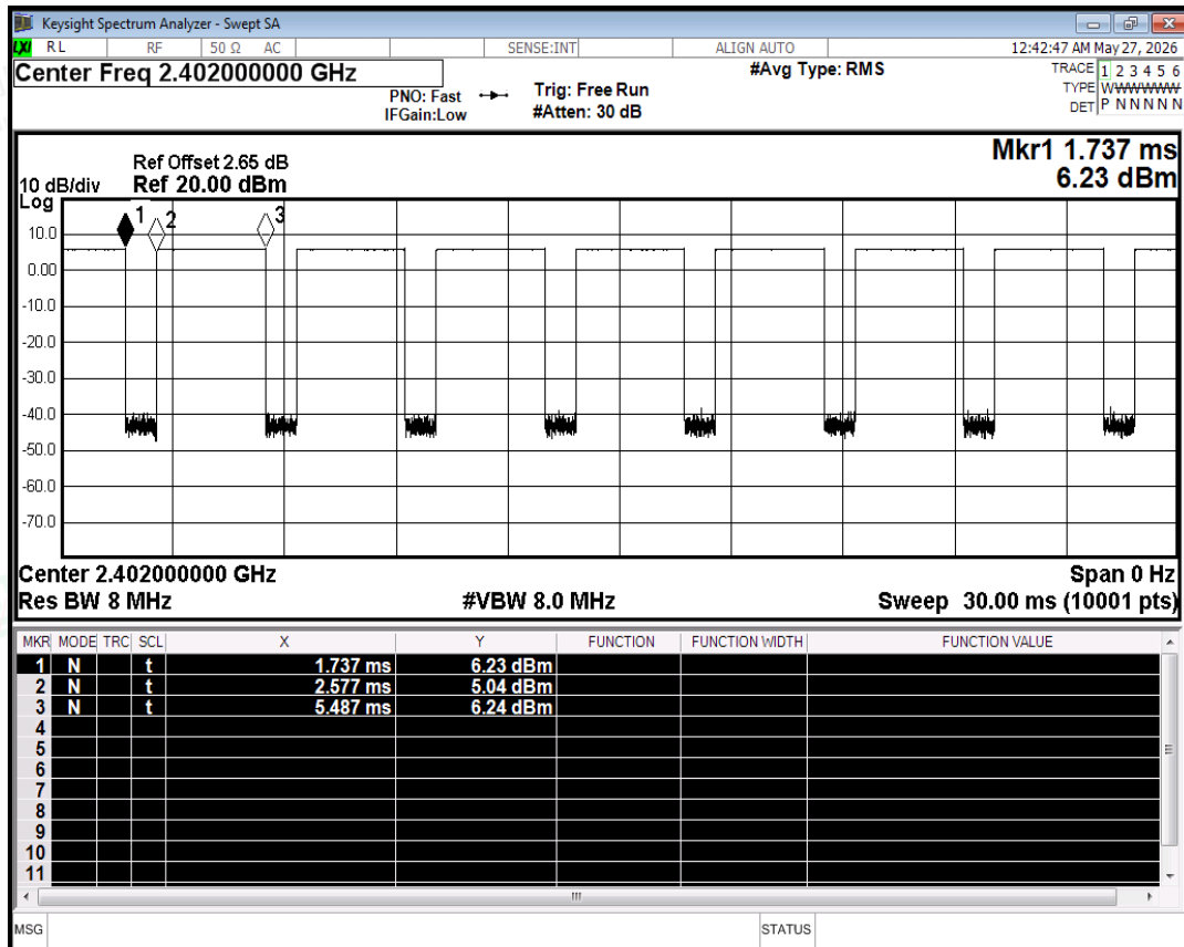
Duty Cycle NVNT 1-DH5 2402MHz Ant
