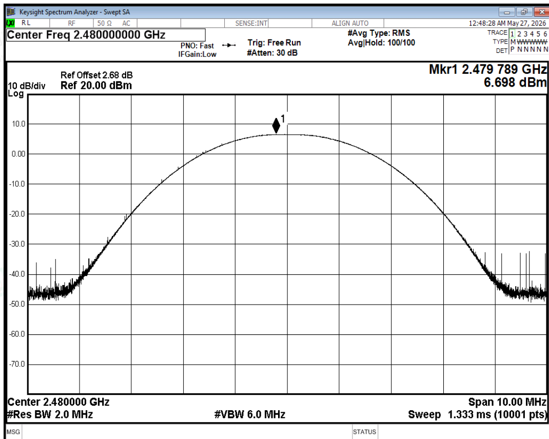
Peak Power NVNT 1-DH5 2480MHz Ant
