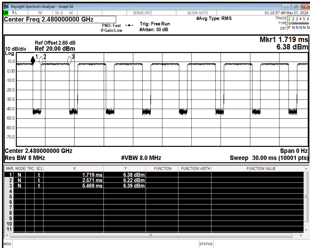
Duty Cycle NVNT 2-DH5 2480MHz Ant
