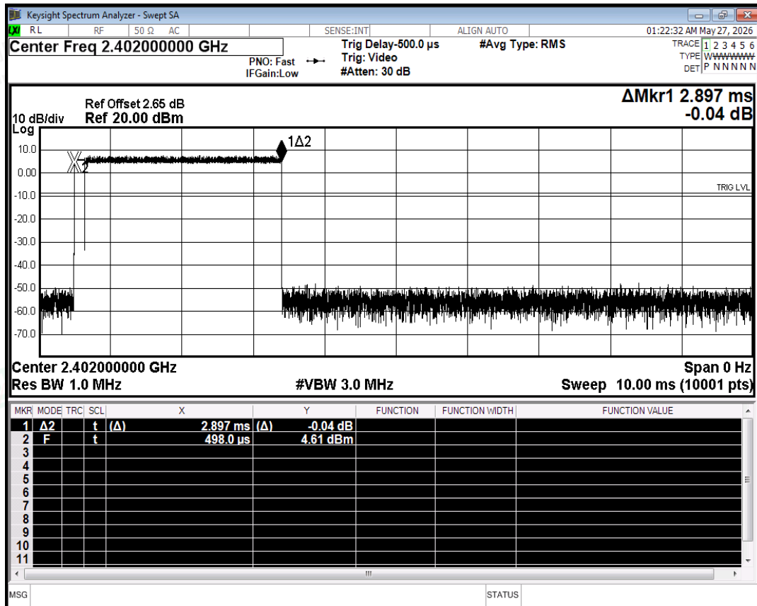
Dwell NVNT 3-DH5 2402MHz Ant One Burst
