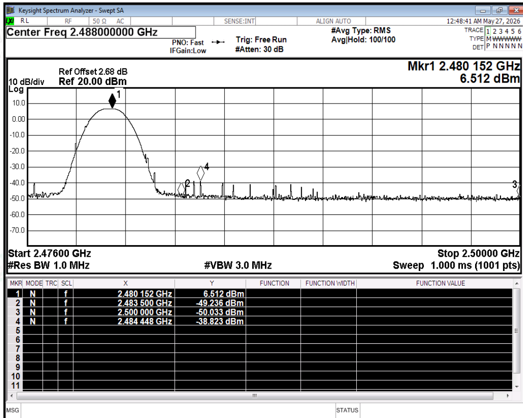
Restrict Band NVNT 1-DH5 2480MHz Ant No-Hopping Peak
