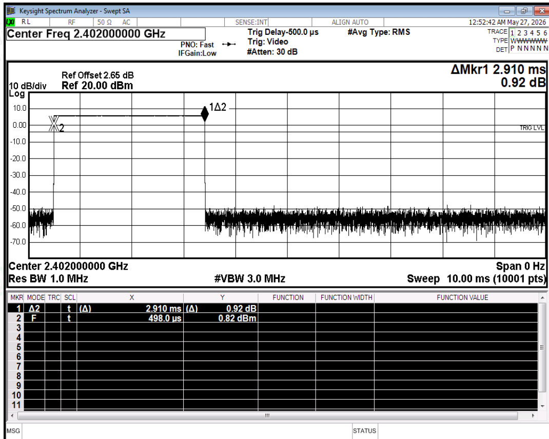
Dwell NVNT 1-DH5 2402MHz Ant One Burst
