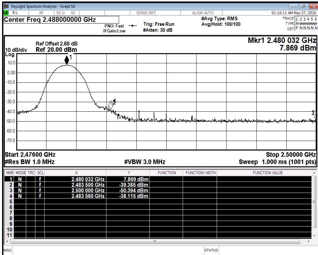
Restrict Band NVNT 3-DH5 2480MHz Ant No-Hopping Peak
