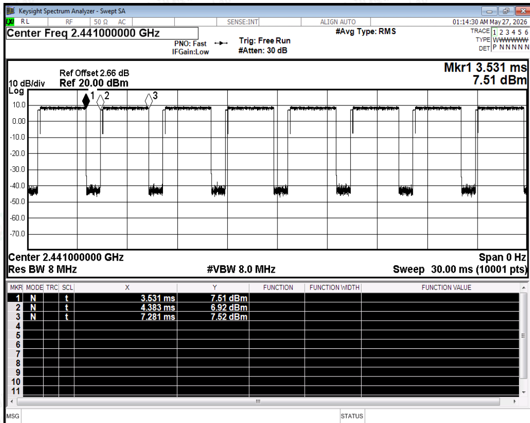
Duty Cycle NVNT 3-DH5 2441MHz Ant
