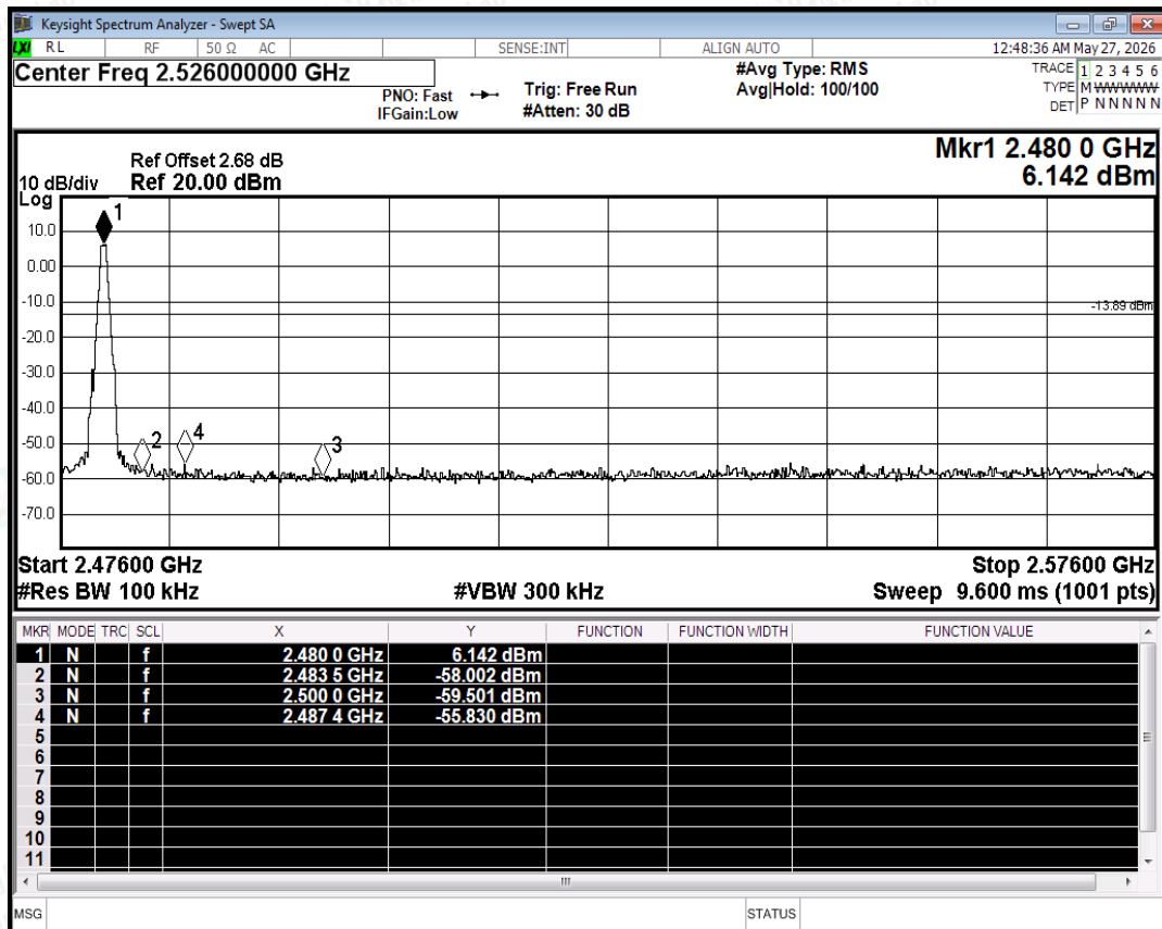
Band Edge NVNT 1-DH5 2480MHz Ant No-Hopping Emission
