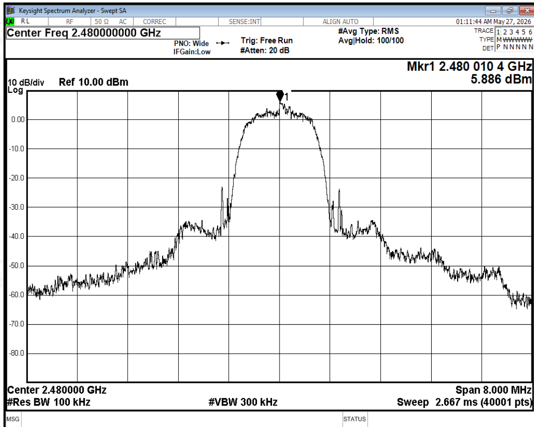
Tx. Spurious NVNT 2-DH5 2480MHz Ant Ref
