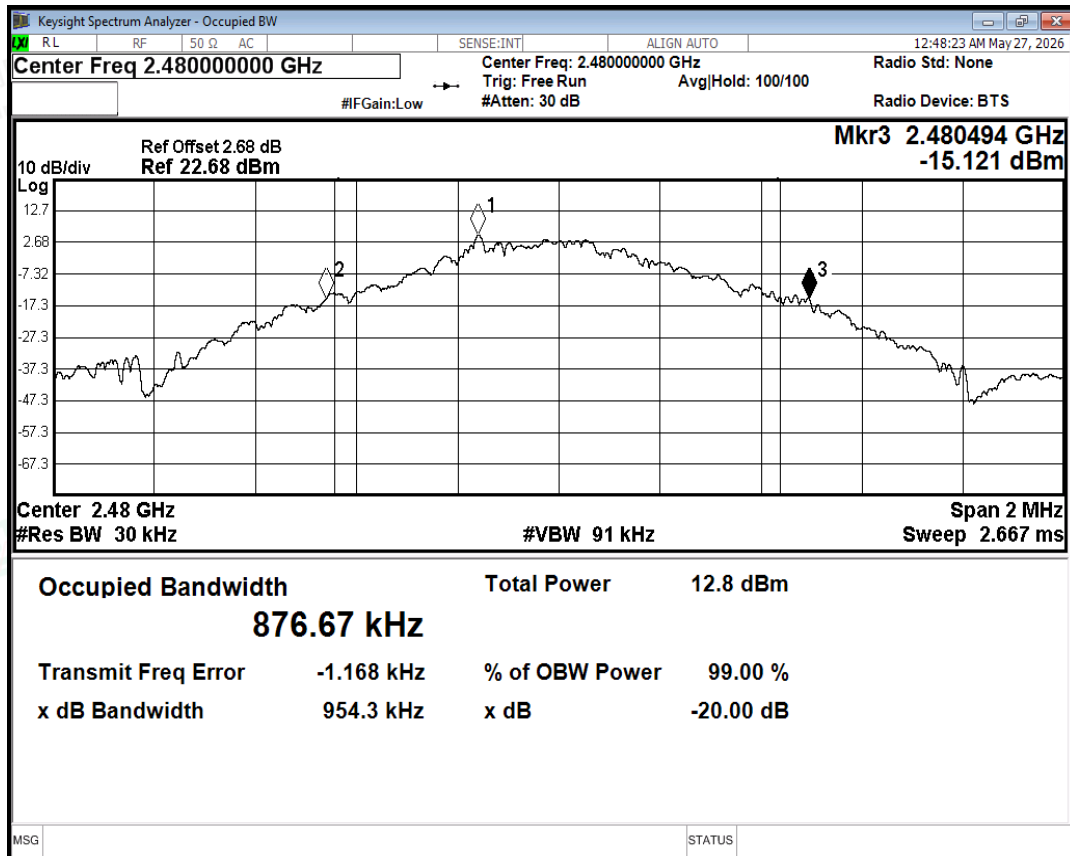
-20dB Bandwidth NVNT 1-DH5 2480MHz Ant
