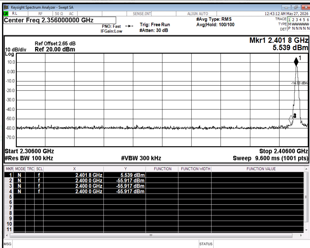
Band Edge NVNT 1-DH5 2402MHz Ant No-Hopping Emission
