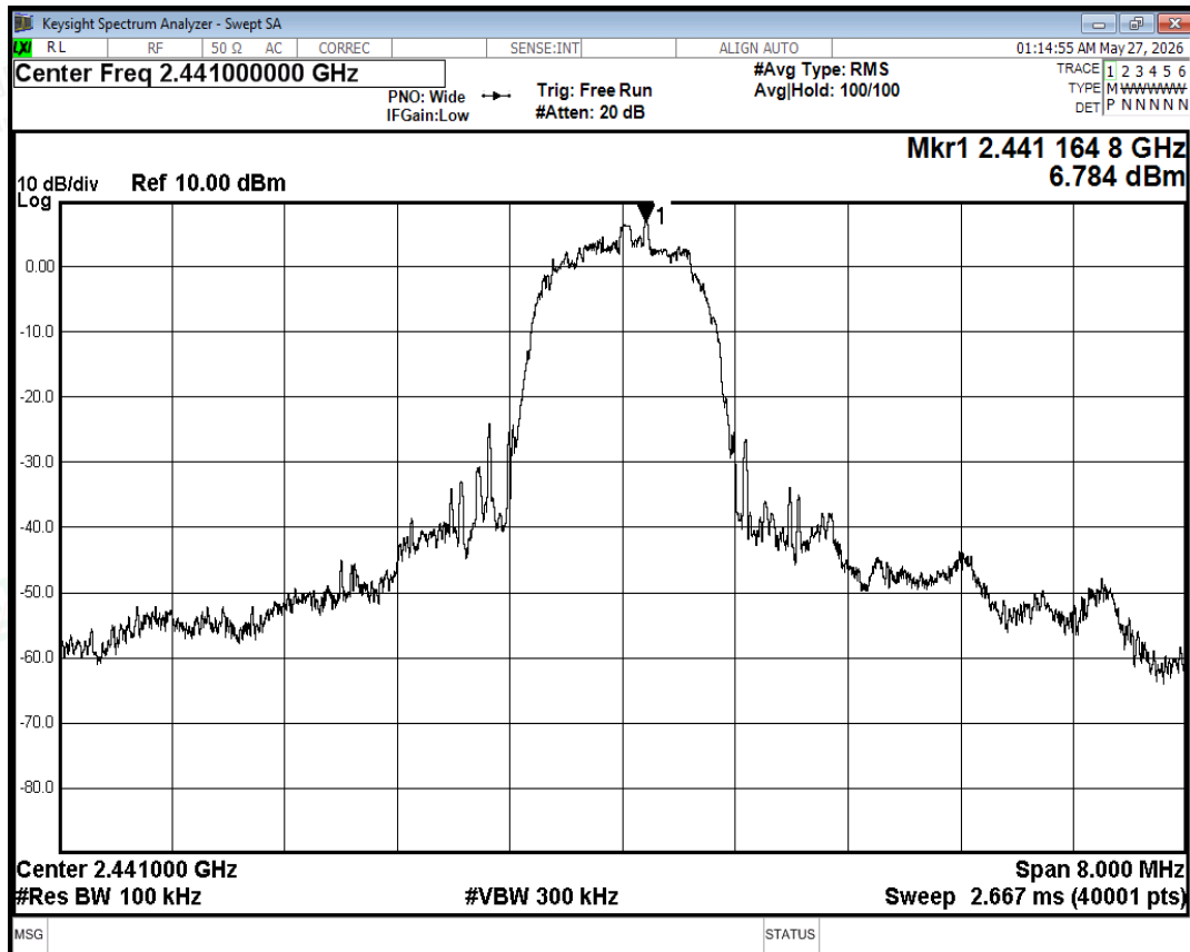
Tx. Spurious NVNT 3-DH5 2441MHz Ant Ref
