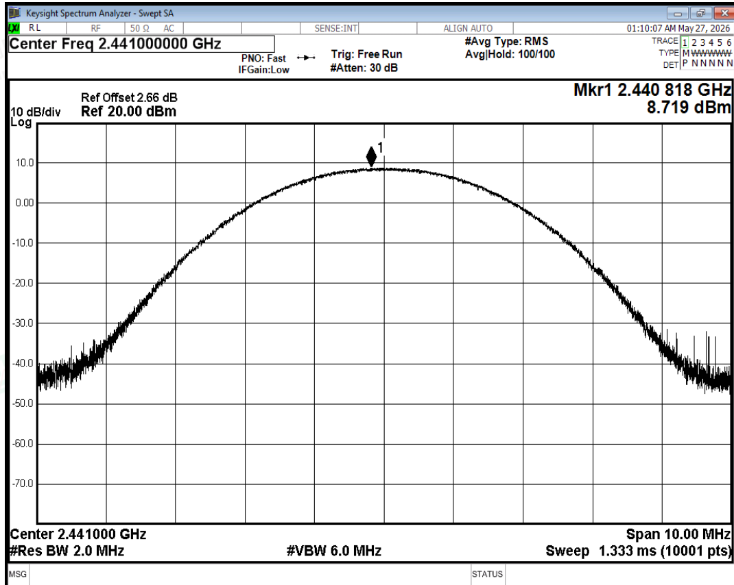
Peak Power NVNT 2-DH5 2441MHz Ant
