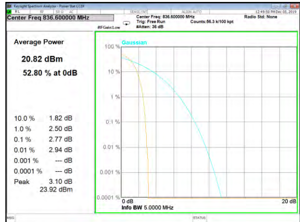
HSPA5_Middle_
