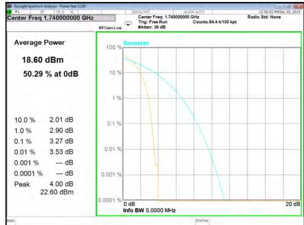
HSPA4_Middle_
