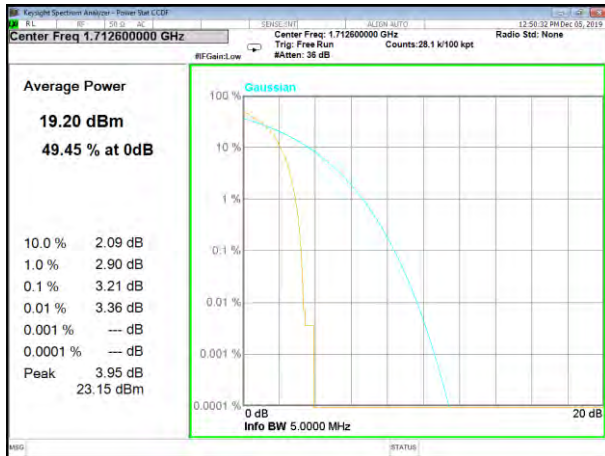
HSPA4_Lower
