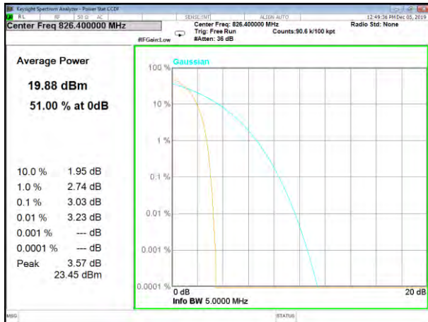
HSPA5_Lower_
