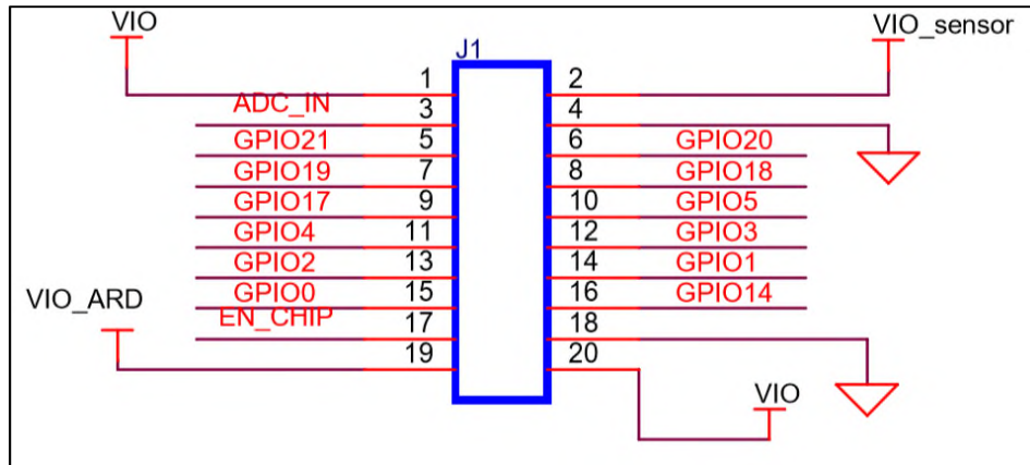
Figure 5: IO Header
