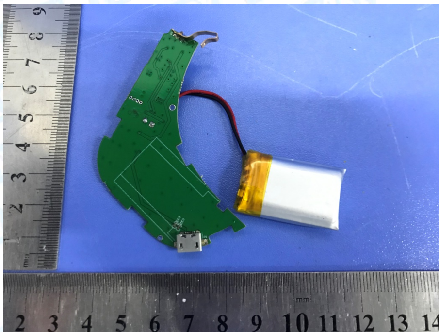
Photo 13 Apperance of PCB
