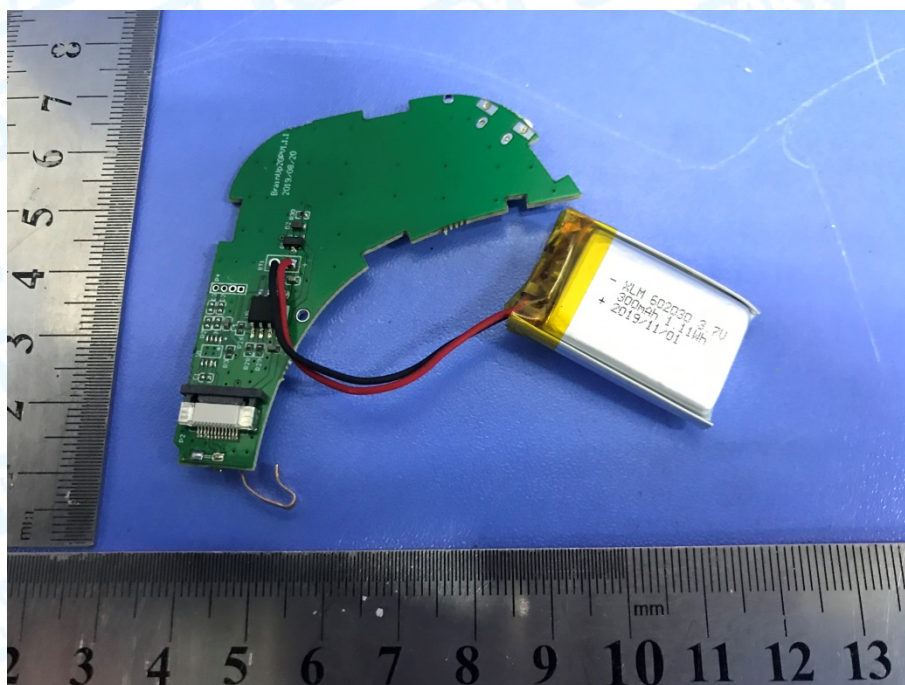
Photo 11 Apperance of PCB
