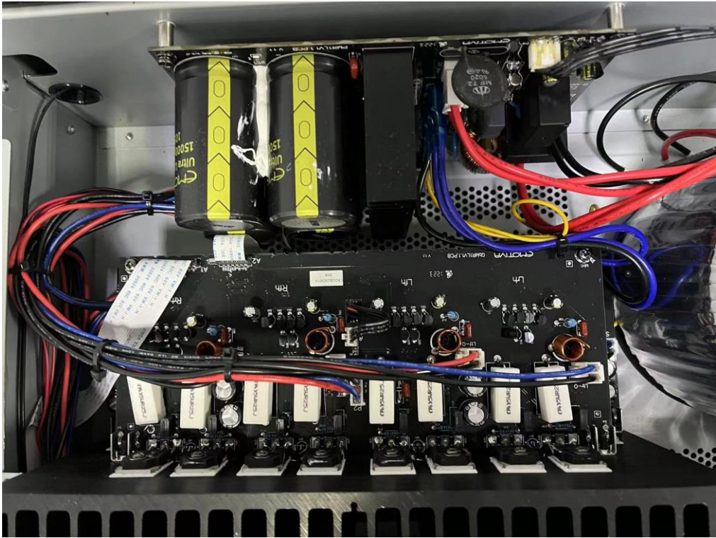
Internal Photos M/N: BASX MR1L
