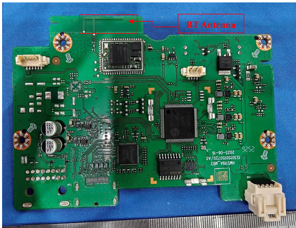
Photo 12: Internal View for BT Antenna
