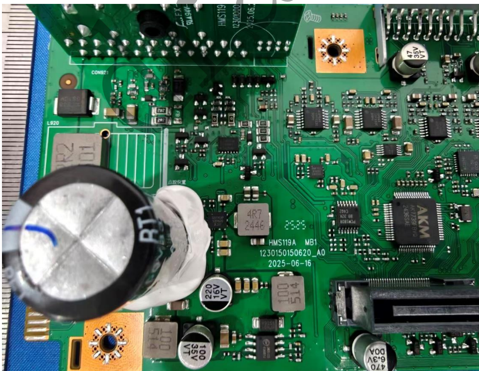
Photo 10: Internal View for PCB C
