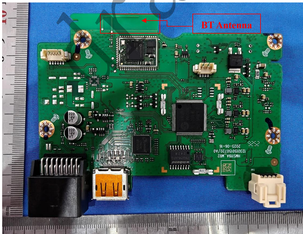
Photo 12: Internal View for BT Antenna
