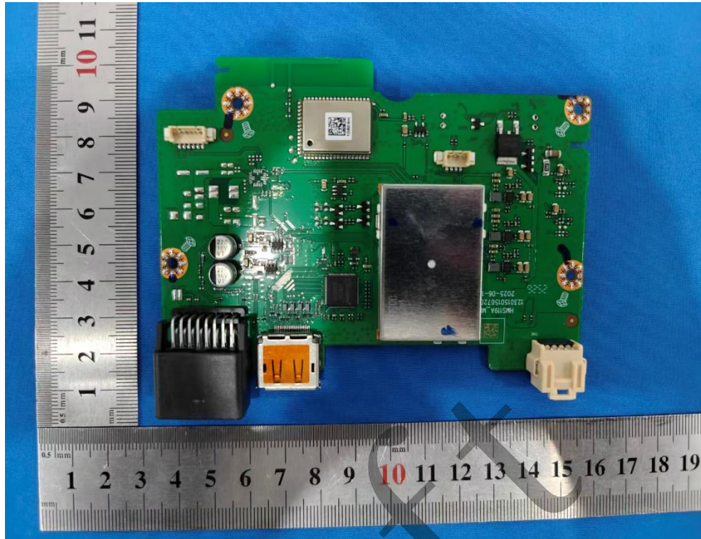
Photo 3: Internal View for PCB B
