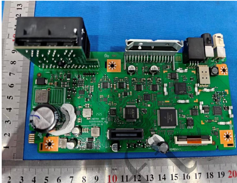
Photo 11: Internal View for PCB C
