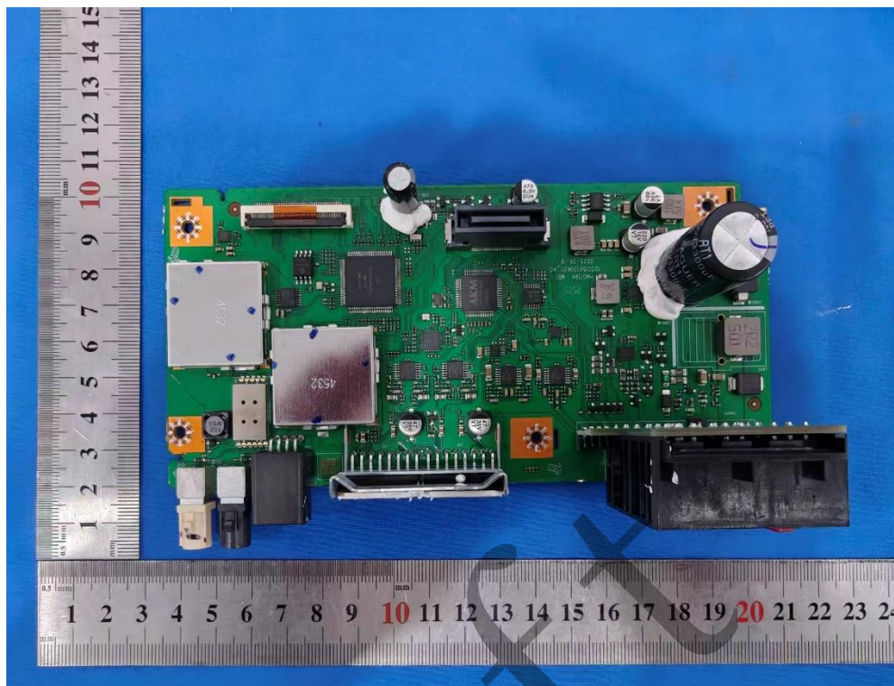
Photo 7: Internal View for PCB C
