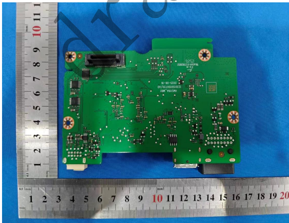
Photo 4: Internal View for PCB B
