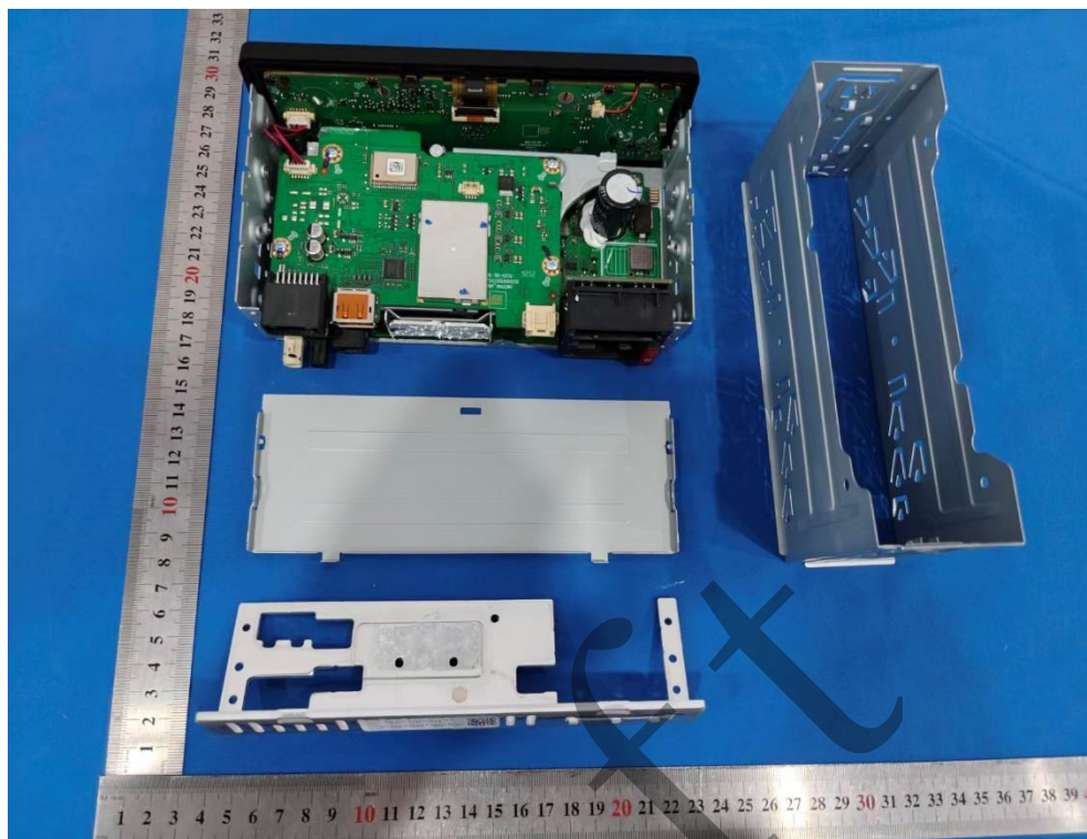
Photo 1: Internal View
