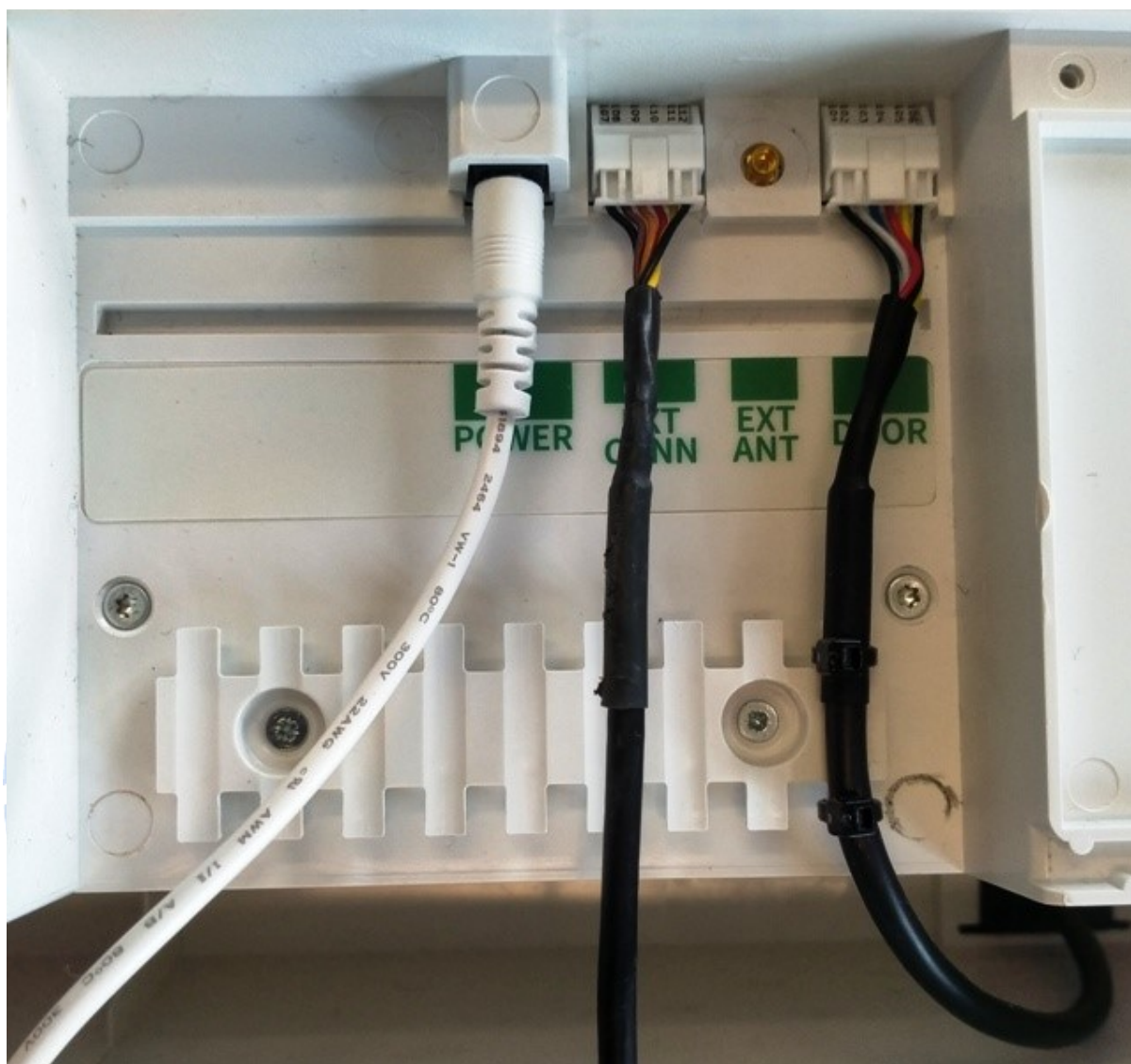
Rear of Cabinet – Cable attached to main board during testing
