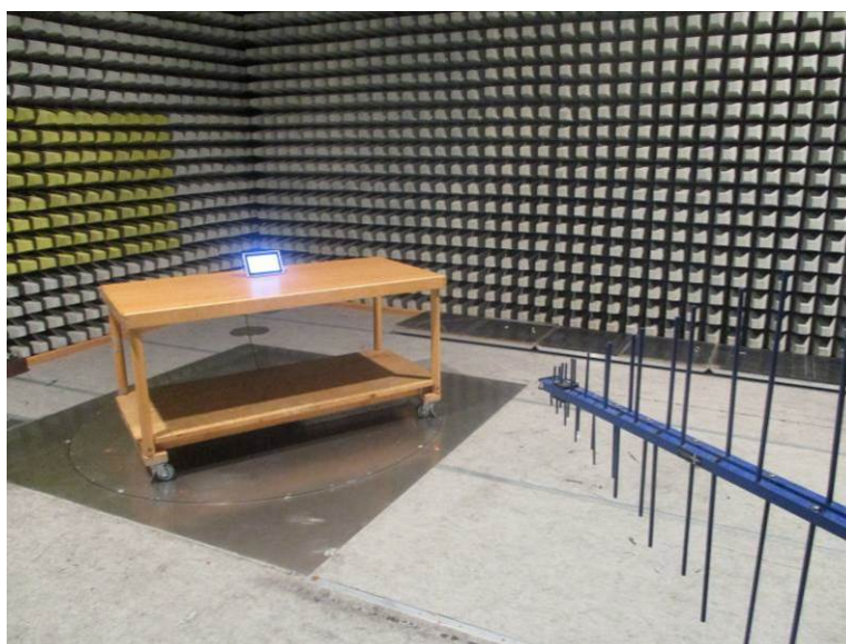
Figure 6-1: test setup for Radiated disturbances 30 MHz to 1000 MHz
