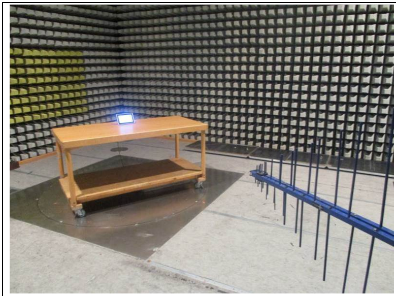
Figure 1: test setup Radiated disturbances 30 MHz to 1000 MHz
