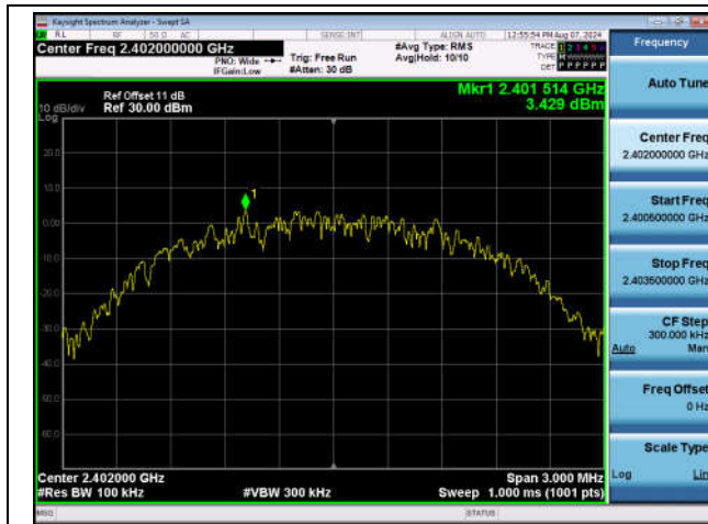
BLE_2M-Ant1-2402-0~Reference-PASS
