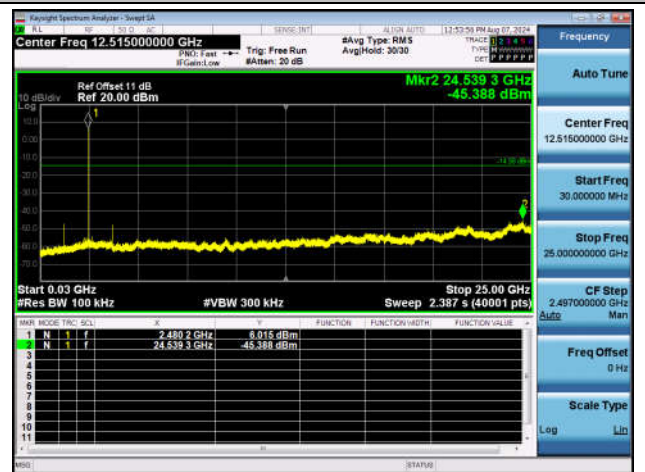
BLE_1M-Ant1-2480-30~25000-PASS
