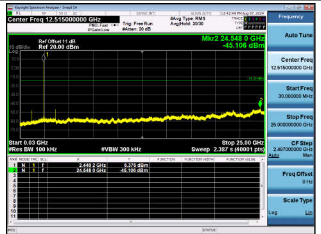
BLE_1M-Ant1-2440-30~25000-PASS
