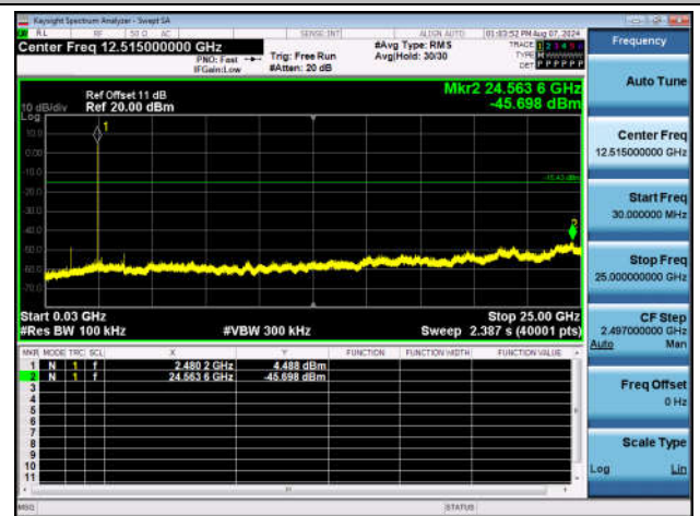
BLE_2M-Ant1-2480-30~25000-PASS
