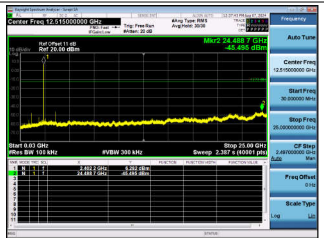
BLE_1M-Ant1-2402-30~25000-PASS
