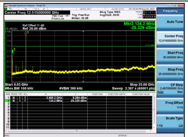
2DH5-Ant1-2480-30~25000-PASS
