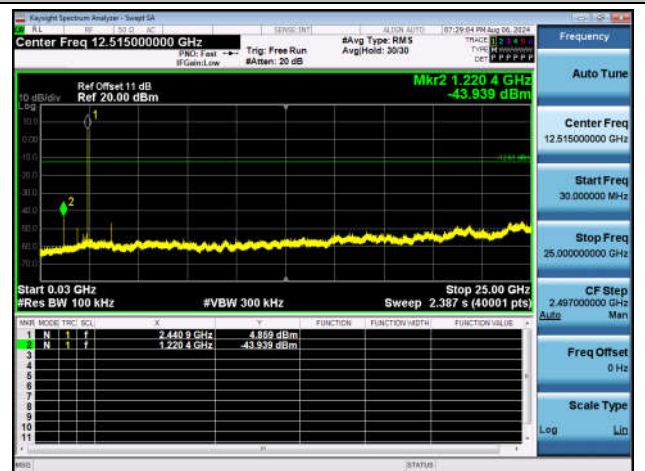
2DH5-Ant1-2441-30~25000-PASS
