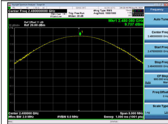
3DH5-Ant1-2480-PASS
