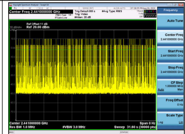
2DH5-Ant1-Hop-PASS
