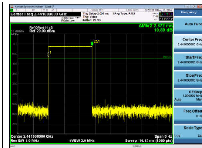
DH5-Ant1-Hop-PASS
