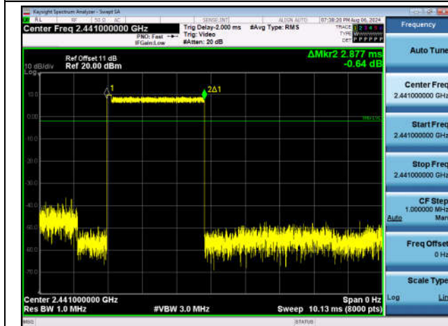
2DH5-Ant1-Hop-PASS
