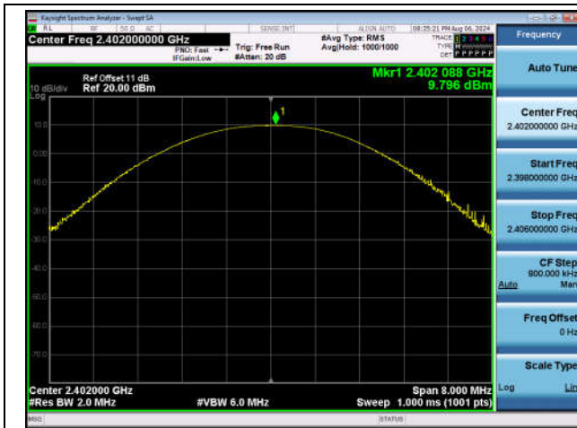
3DH5-Ant1-2402-PASS
