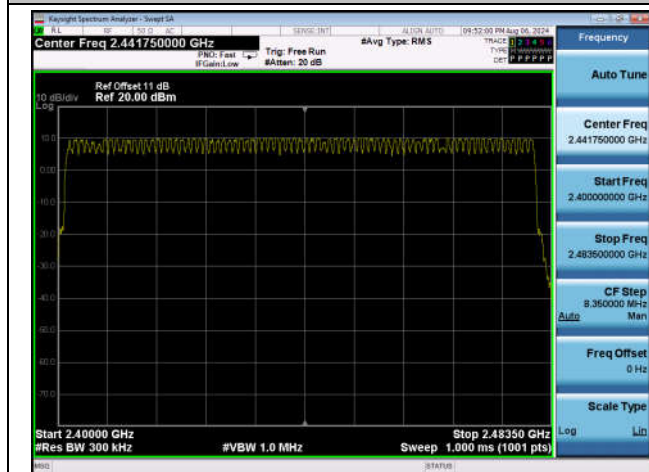
3DH5-Ant1-Hop-PASS
