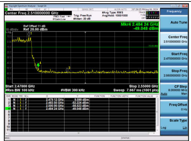
2DH5-Ant1-Hop_2480-PASS
