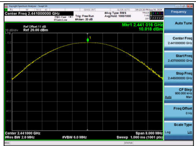
3DH5-Ant1-2441-PASS
