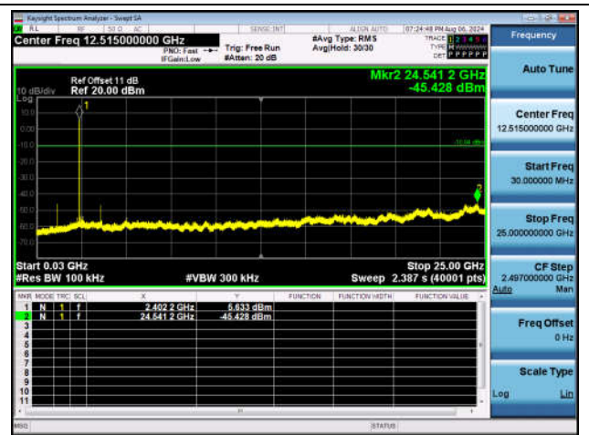
2DH5-Ant1-2402-30~25000-PASS
