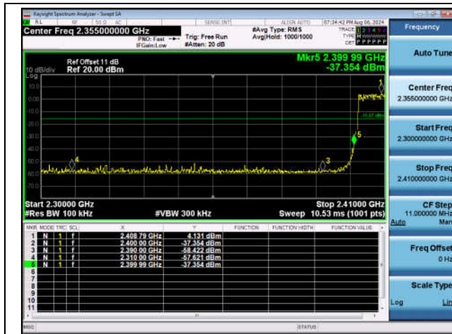
2DH5-Ant1-Hop_2402-PASS
