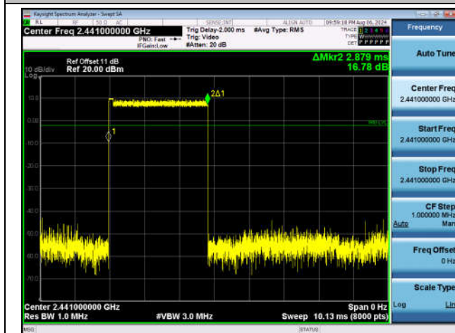
3DH5-Ant1-Hop-PASS
