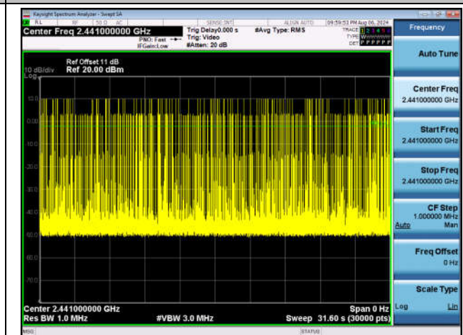
3DH5-Ant1-Hop-PASS
