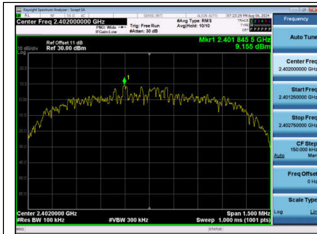
2DH5-Ant1-2402-0~Reference-PASS
