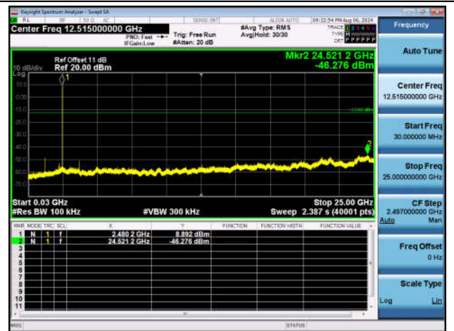
3DH5-Ant1-2480-30~25000-PASS
