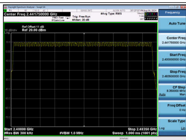
2DH5-Ant1-Hop-PASS
