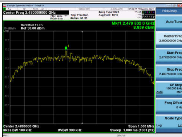
2DH5-Ant1-2480-0~Reference-PASS
