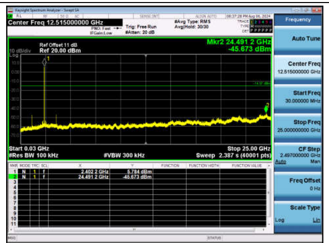
3DH5-Ant1-2402-30~25000-PASS
