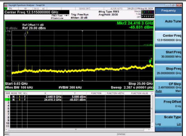
3DH5-Ant1-2441-30~25000-PASS
