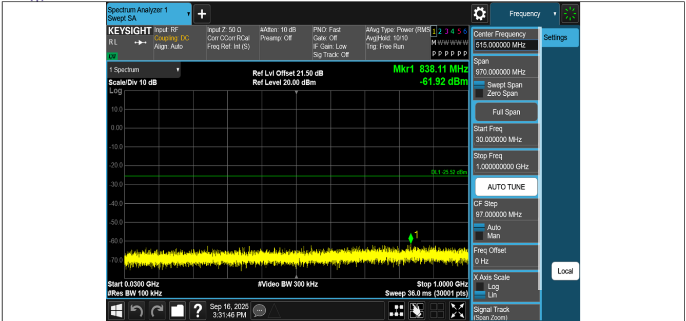
11B-CDD-Ant1-2412-30~1000-PASS
