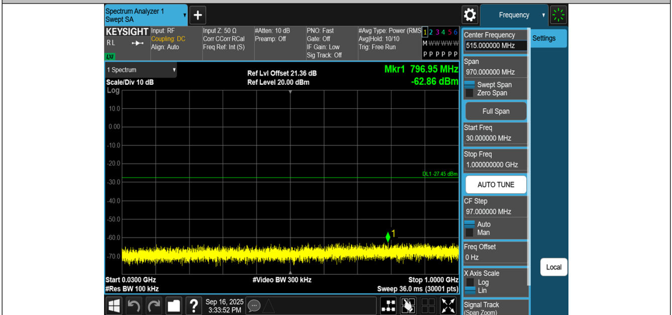
11B-CDD-Ant2-2412-30~1000-PASS
