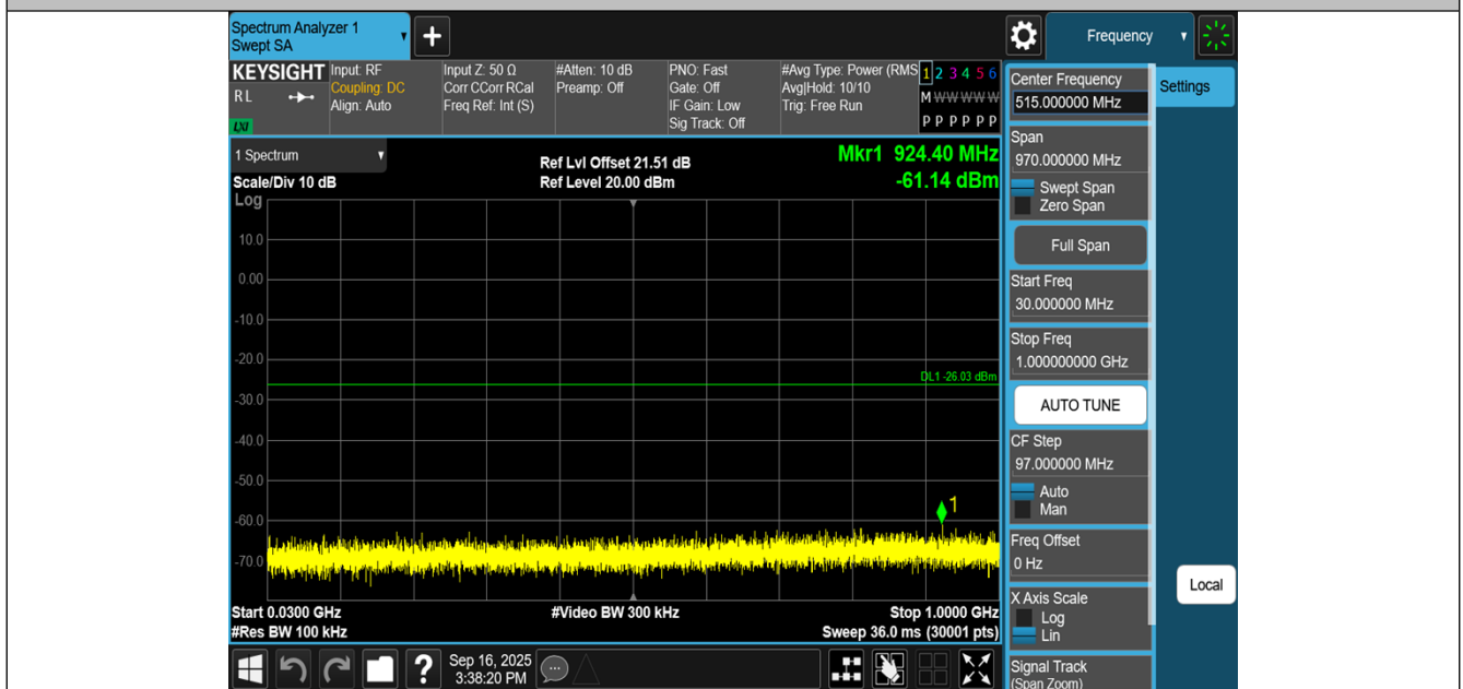
11B-CDD-Ant2-2437-30~1000-PASS
