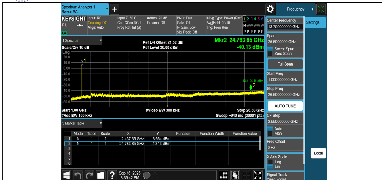
11B-CDD-Ant1-2437-1000~26500-PASS
