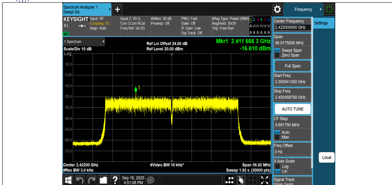
11AX40MIMO-Ant2-2422-PASS
