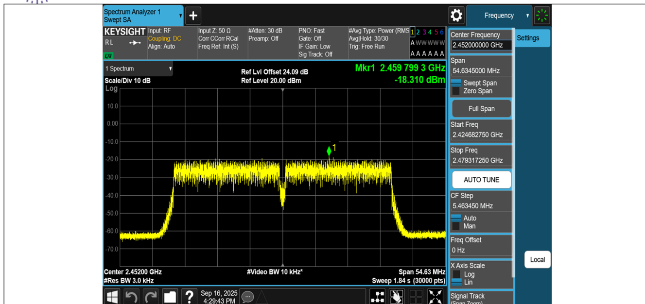
11N40MIMO-Ant2-2452-PASS
