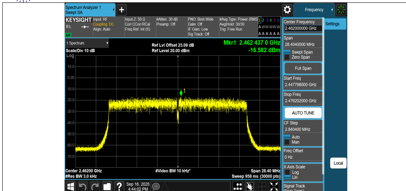
11AX20MIMO-Ant2-2462-PASS
