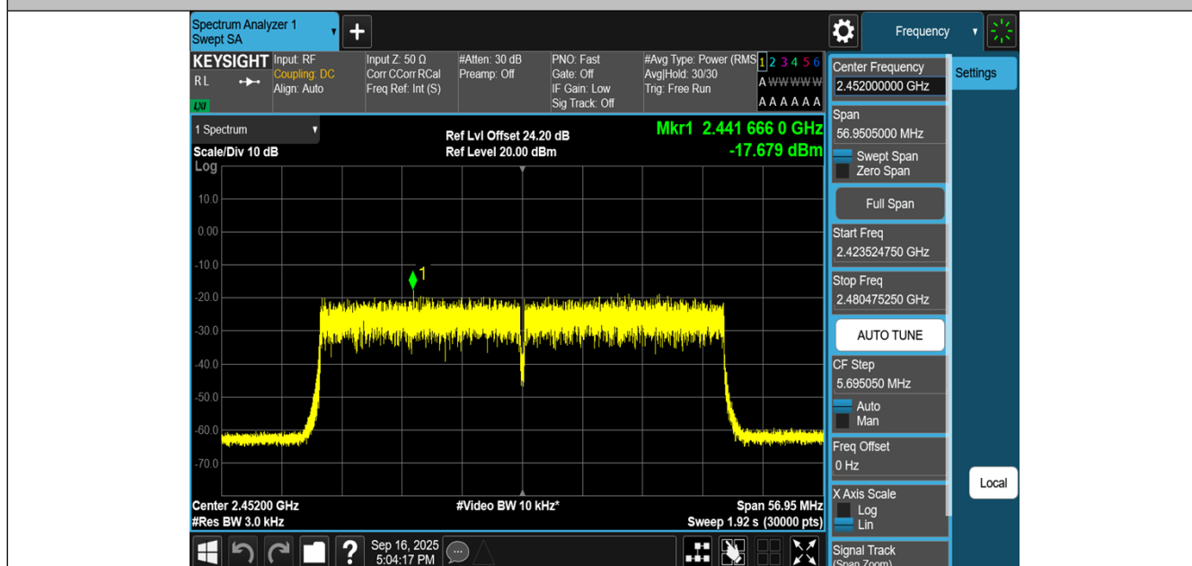
11AX40MIMO-Ant1-2452-PASS
