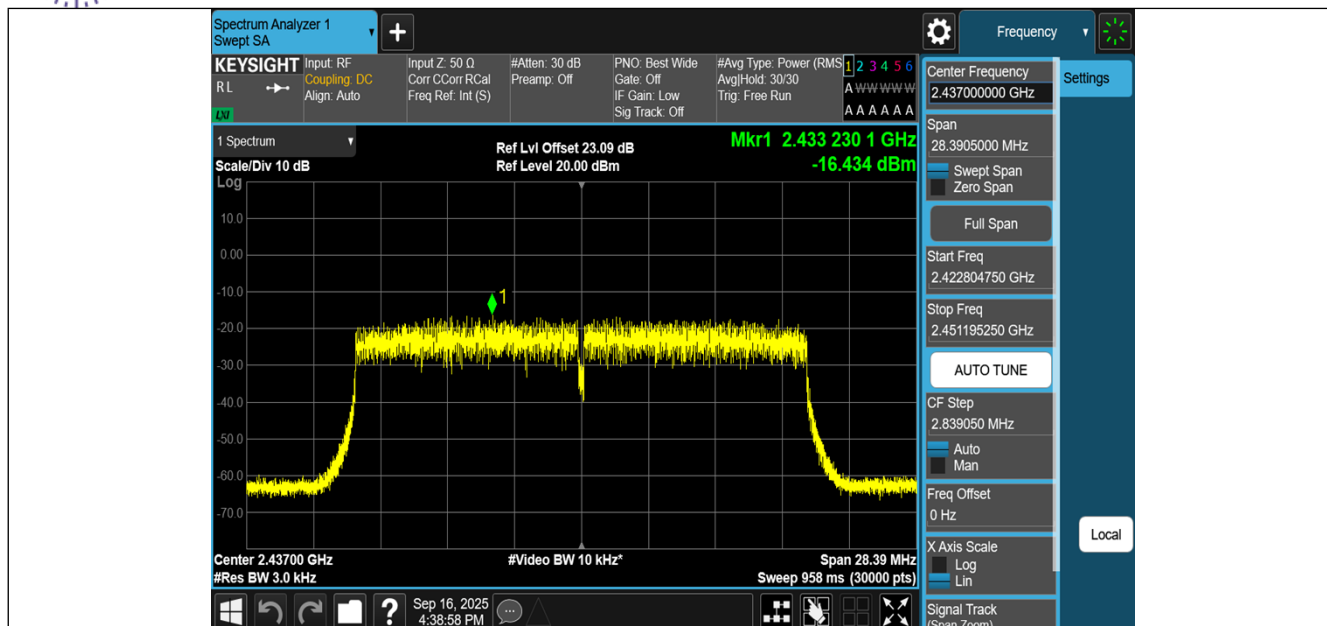
11AX20MIMO-Ant2-2437-PASS
