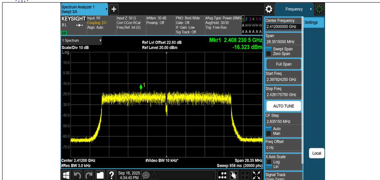
11AX20MIMO-Ant2-2412-PASS
