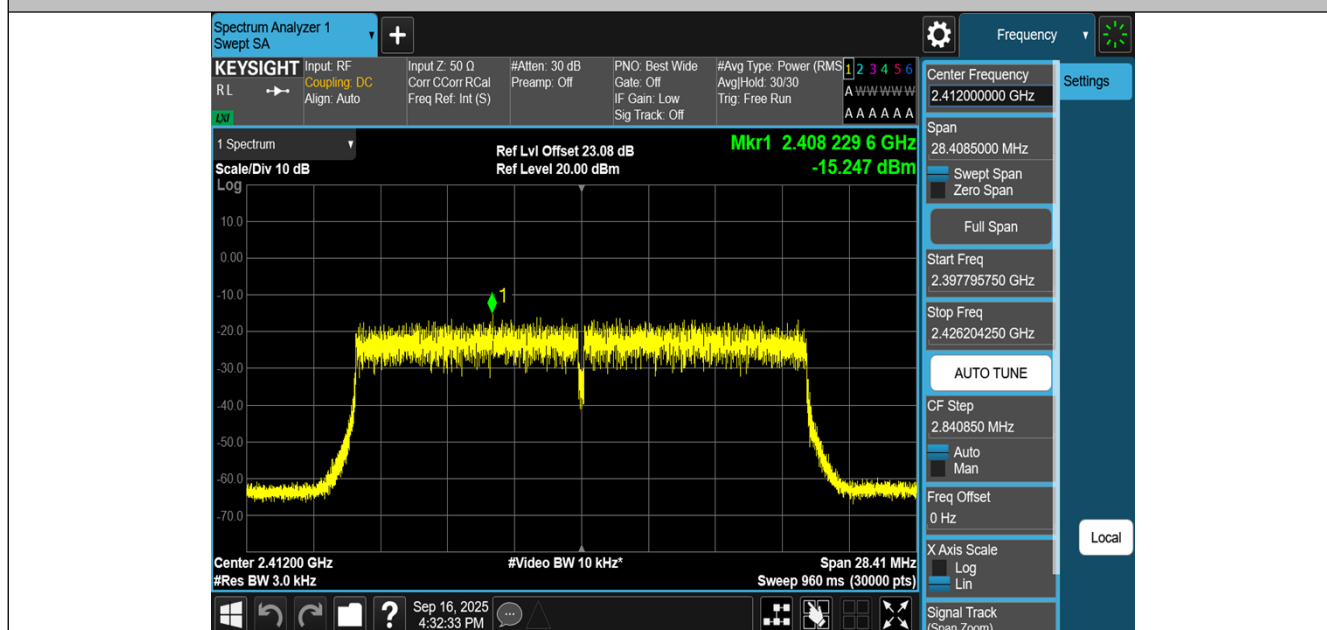
11AX20MIMO-Ant1-2412-PASS
