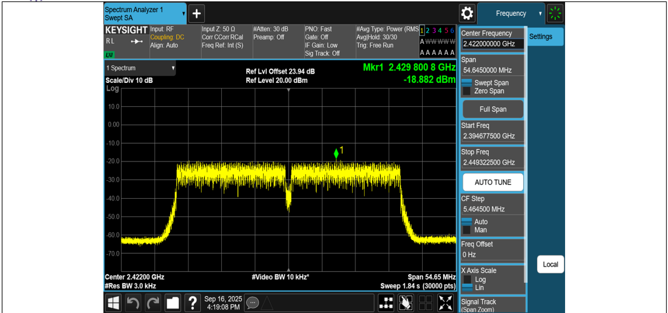
11N40MIMO-Ant2-2422-PASS
