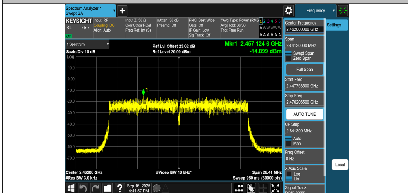
11AX20MIMO-Ant1-2462-PASS
