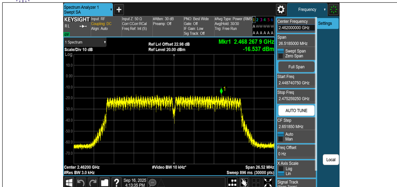
11N20MIMO-Ant2-2462-PASS
