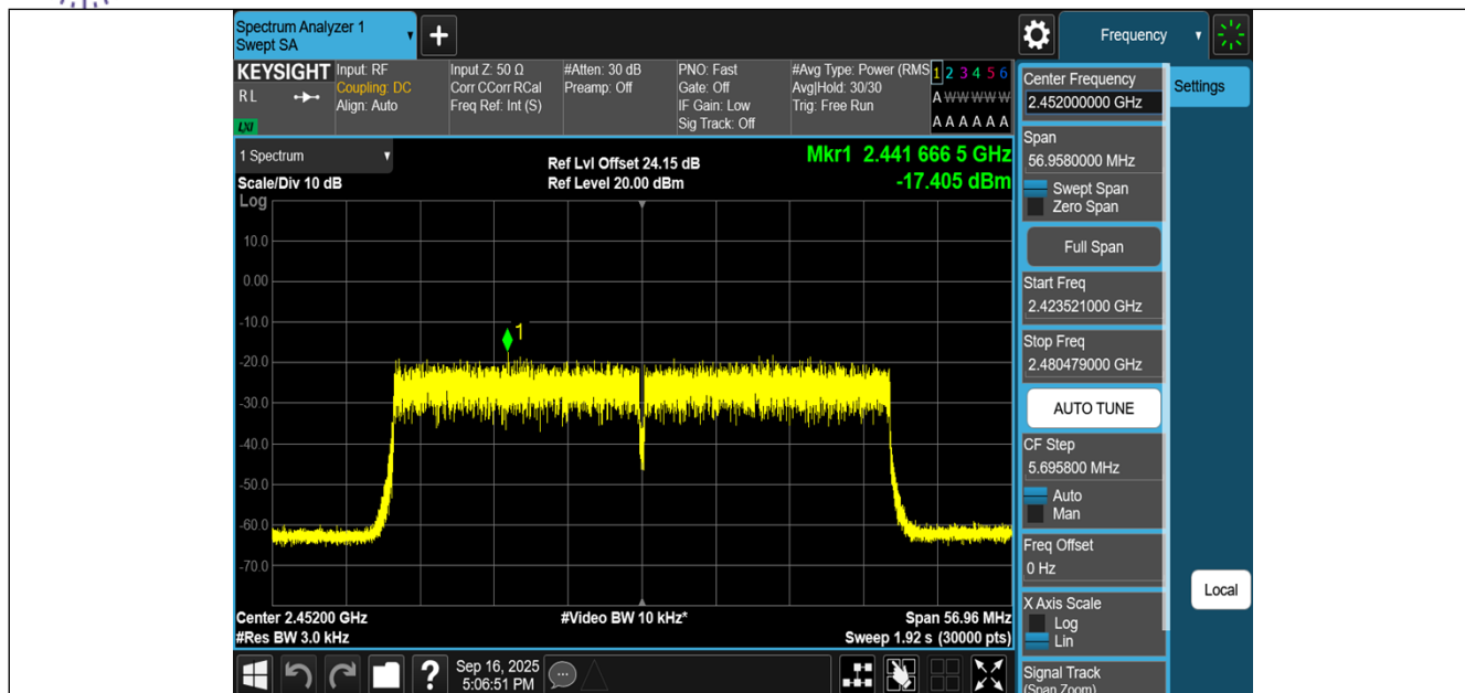
11AX40MIMO-Ant2-2452-PASS
