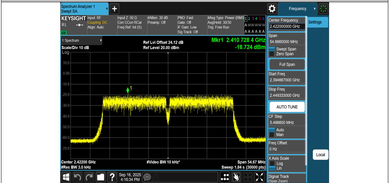
11N40MIMO-Ant1-2422-PASS
