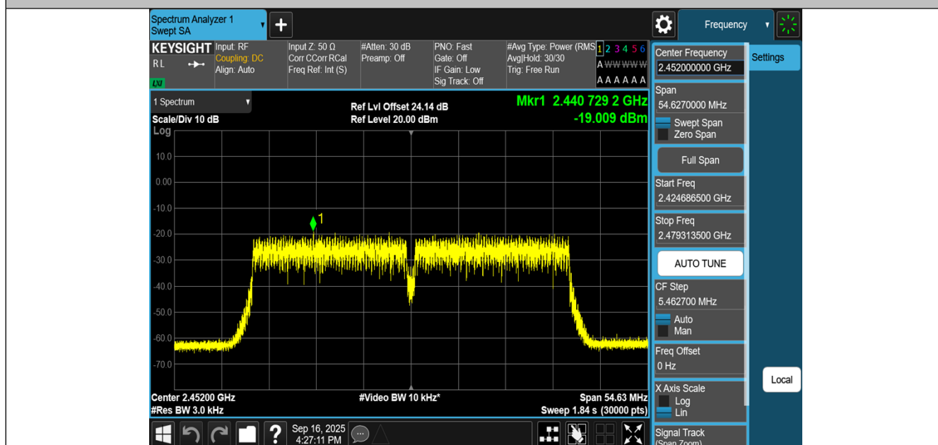
11N40MIMO-Ant1-2452-PASS
