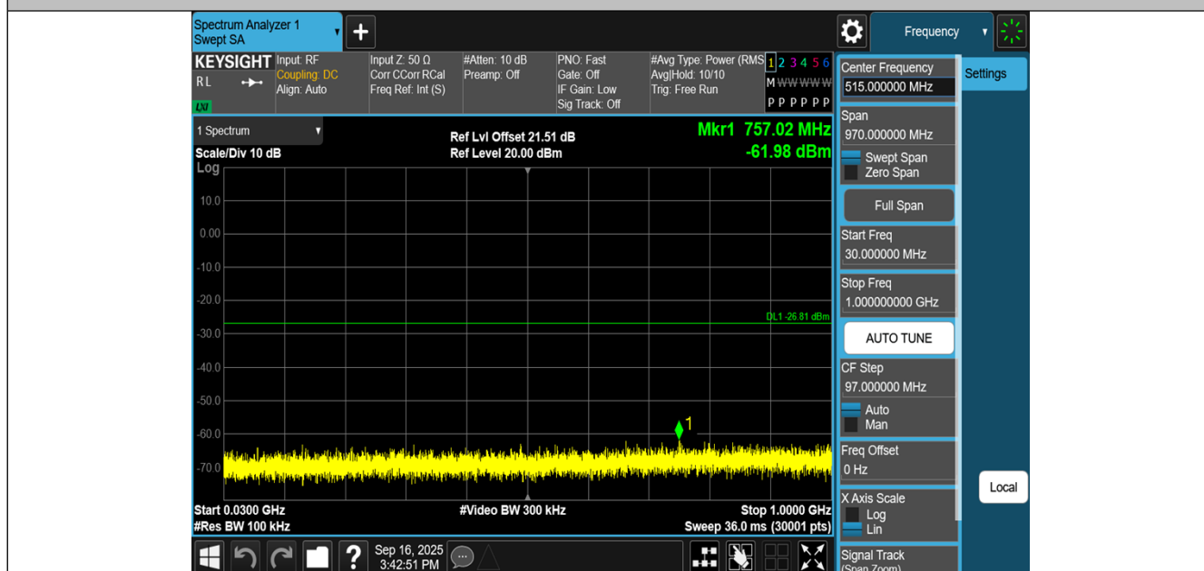
11B-CDD-Ant2-2462-30~1000-PASS
