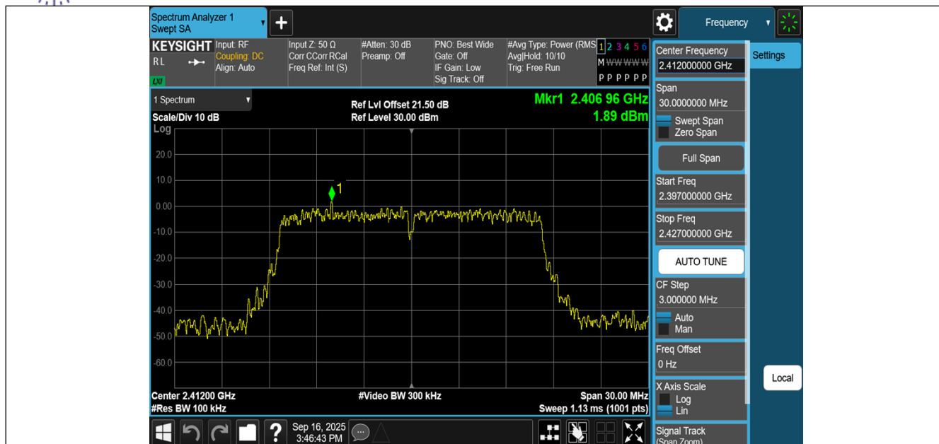
11G-CDD-Ant1-2412-0~Reference-PASS
