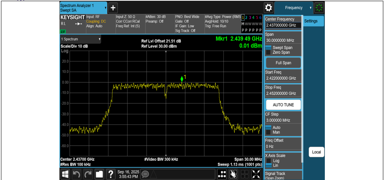
11G-CDD-Ant2-2437-0~Reference-PASS
