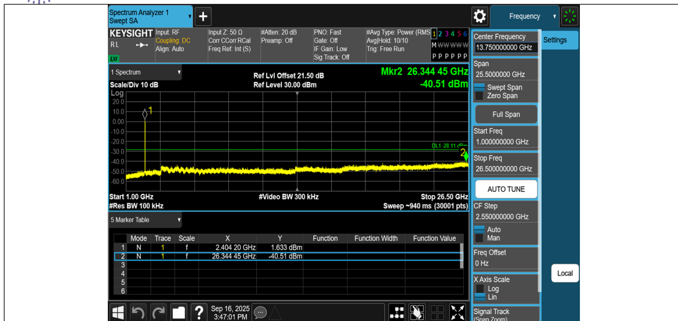
11G-CDD-Ant1-2412-1000~26500-PASS
