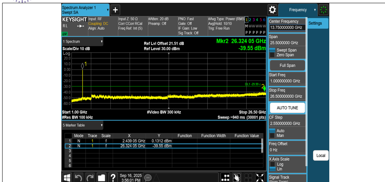
11G-CDD-Ant2-2437-1000~26500-PASS
