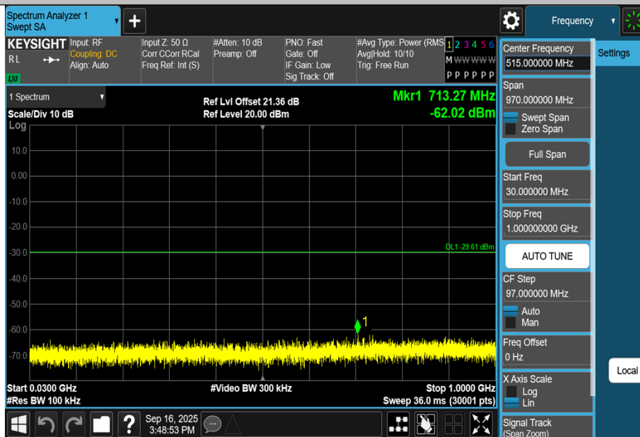
11G-CDD-Ant2-2412-30~1000-PASS
