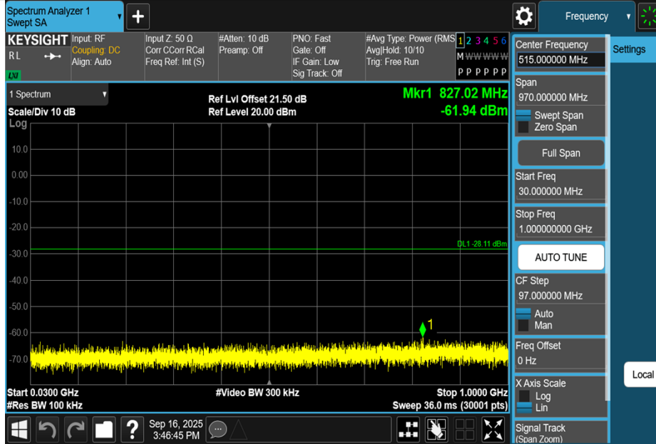
11G-CDD-Ant1-2412-30~1000-PASS
