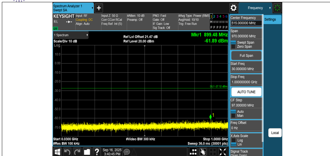
11B-CDD-Ant1-2462-30~1000-PASS
