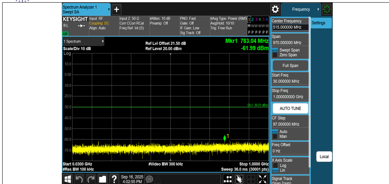
11N20MIMO-Ant1-2412-30~1000-PASS
