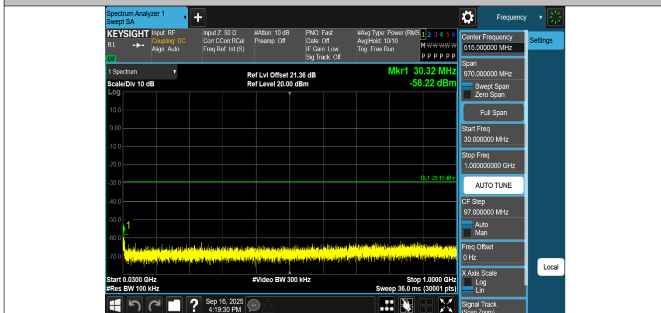
11N40MIMO-Ant2-2422-30~1000-PASS
