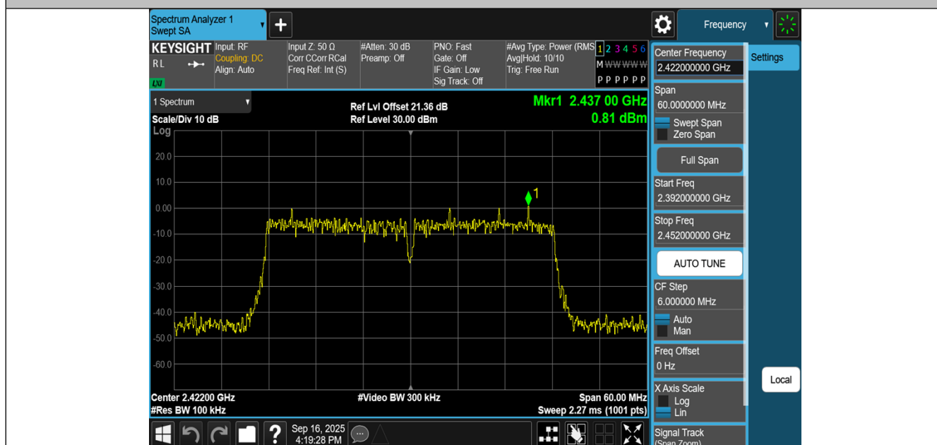
11N40MIMO-Ant2-2422-0~Reference-PASS
