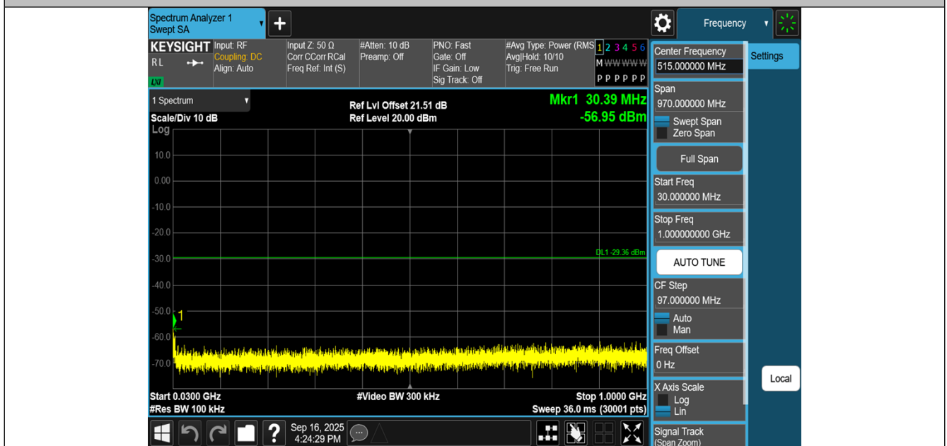
11N40MIMO-Ant2-2437-30~1000-PASS
