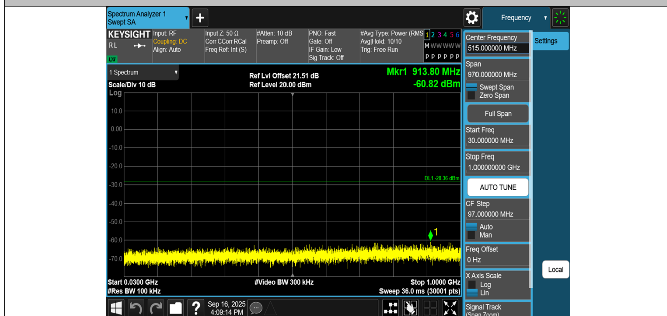
11N20MIMO-Ant2-2437-30~1000-PASS
