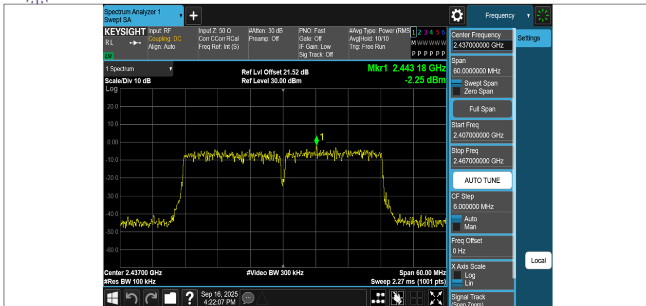
11N40MIMO-Ant1-2437-0~Reference-PASS
