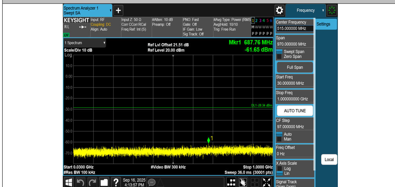
11N20MIMO-Ant2-2462-30~1000-PASS
