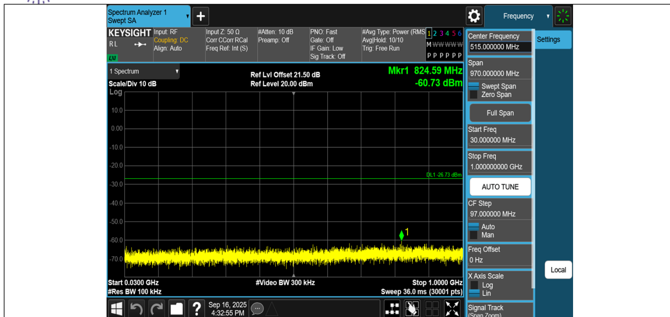
11AX20MIMO-Ant1-2412-30~1000-PASS
