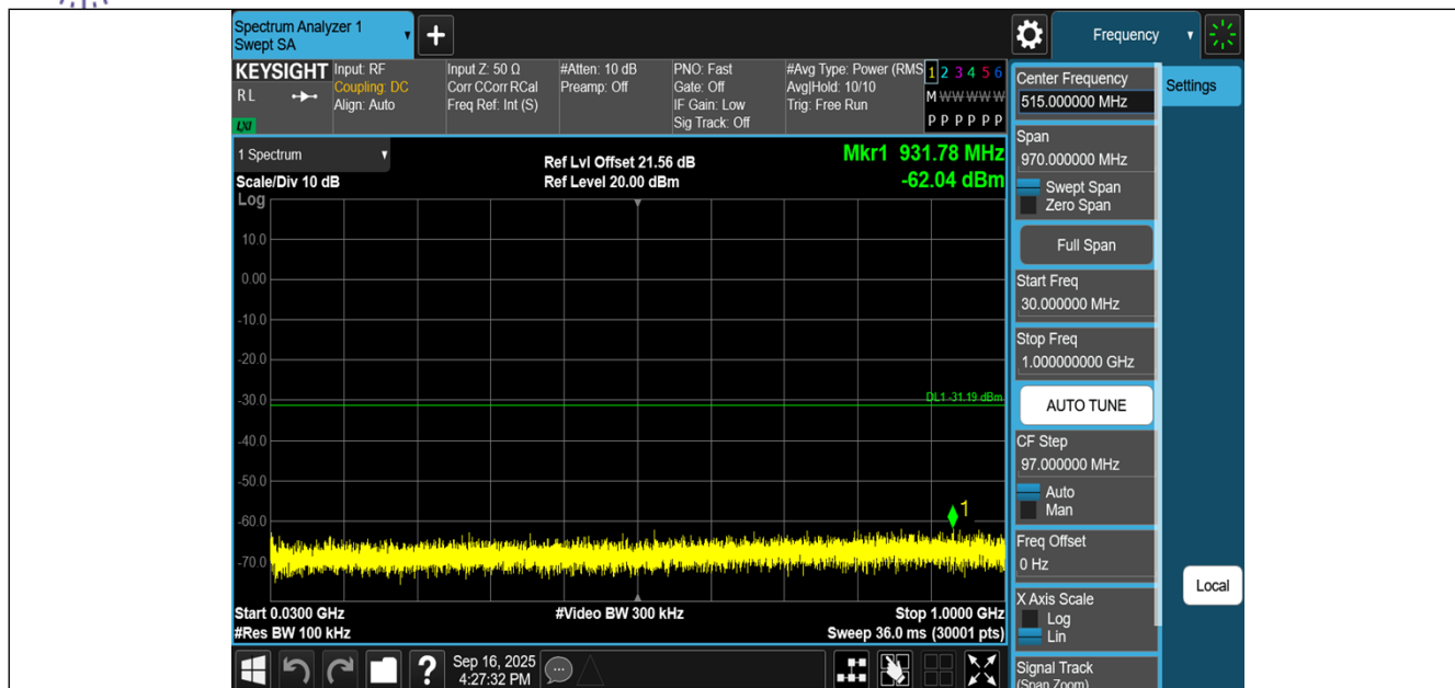
11N40MIMO-Ant1-2452-30~1000-PASS
