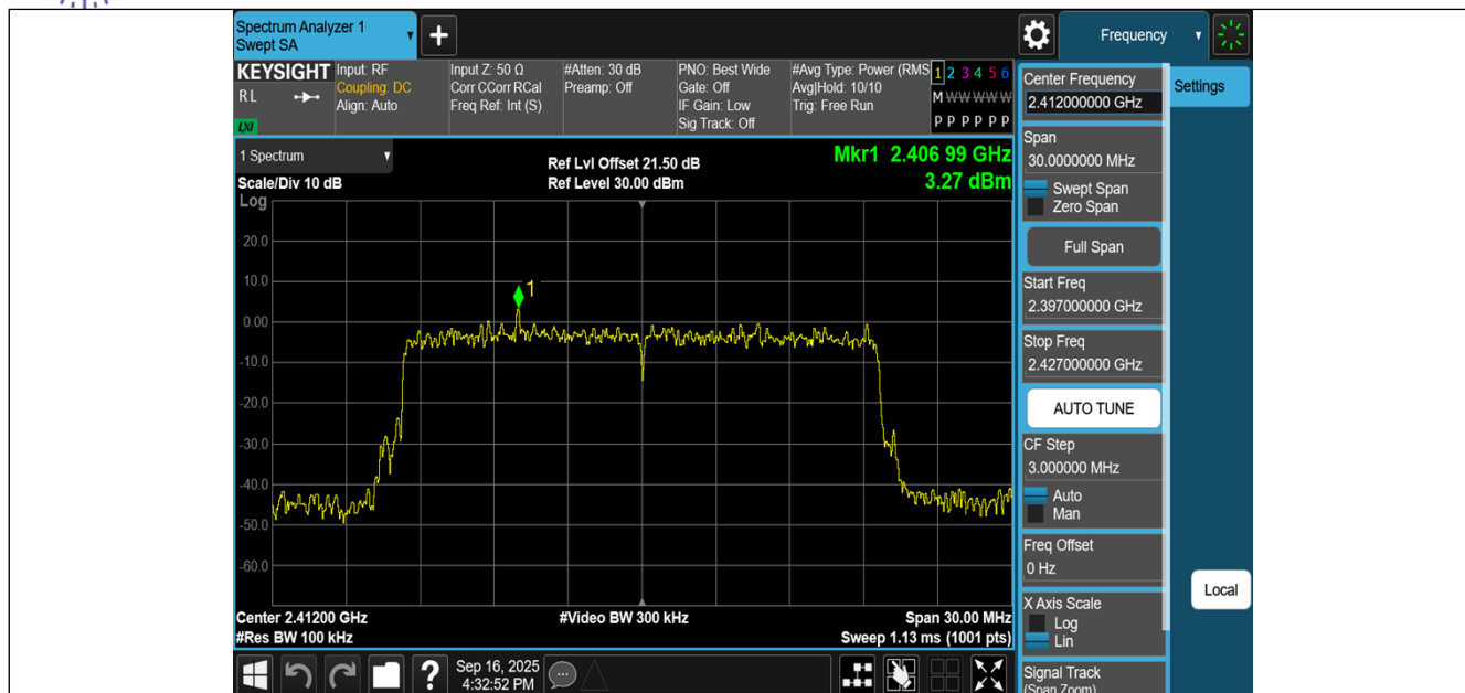
11AX20MIMO-Ant1-2412-0~Reference-PASS
