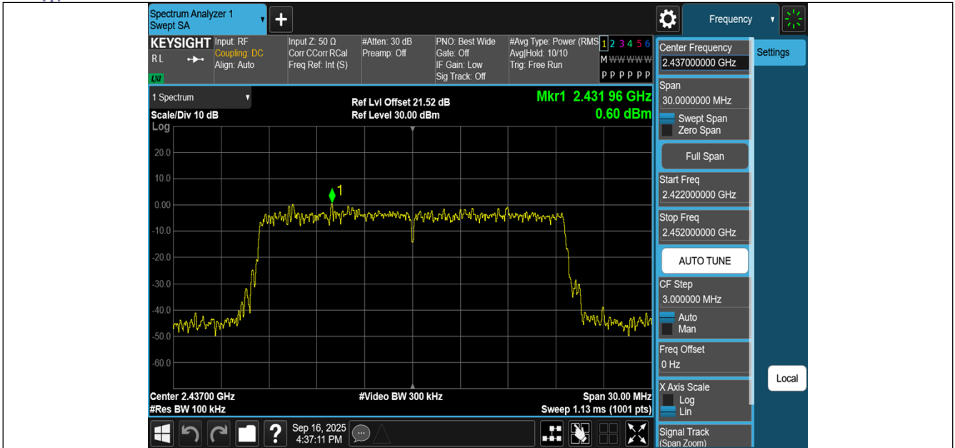
11AX20MIMO-Ant1-2437-0~Reference-PASS
