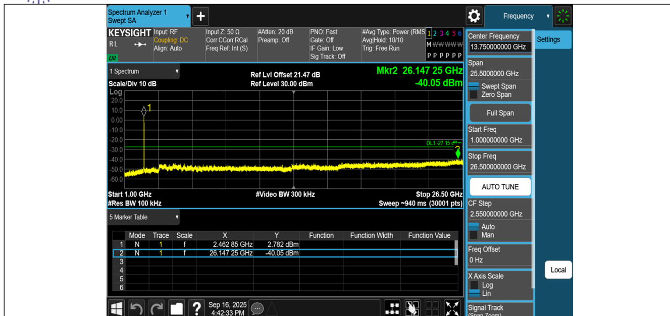
11AX20MIMO-Ant1-2462-1000~26500-PASS
