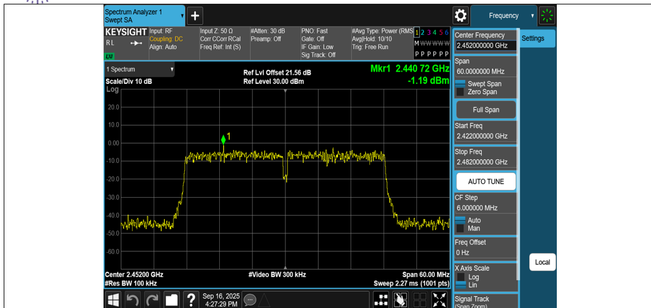
11N40MIMO-Ant1-2452-0~Reference-PASS
