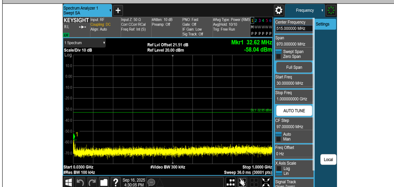
11N40MIMO-Ant2-2452-30~1000-PASS
