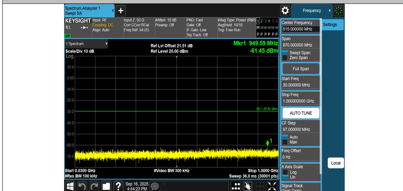
11AX20MIMO-Ant2-2462-30~1000-PASS
