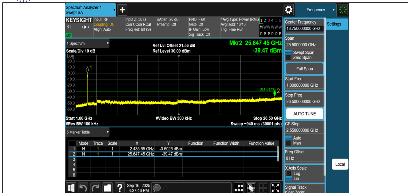
11N40MIMO-Ant1-2452-1000~26500-PASS
