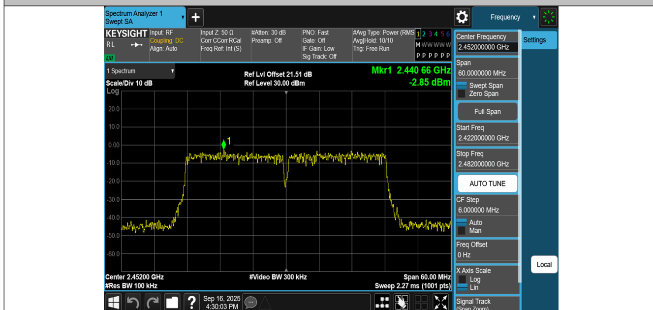
11N40MIMO-Ant2-2452-0~Reference-PASS
