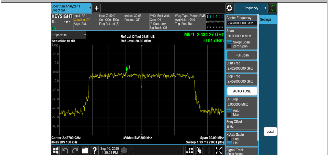
11AX20MIMO-Ant2-2437-0~Reference-PASS
