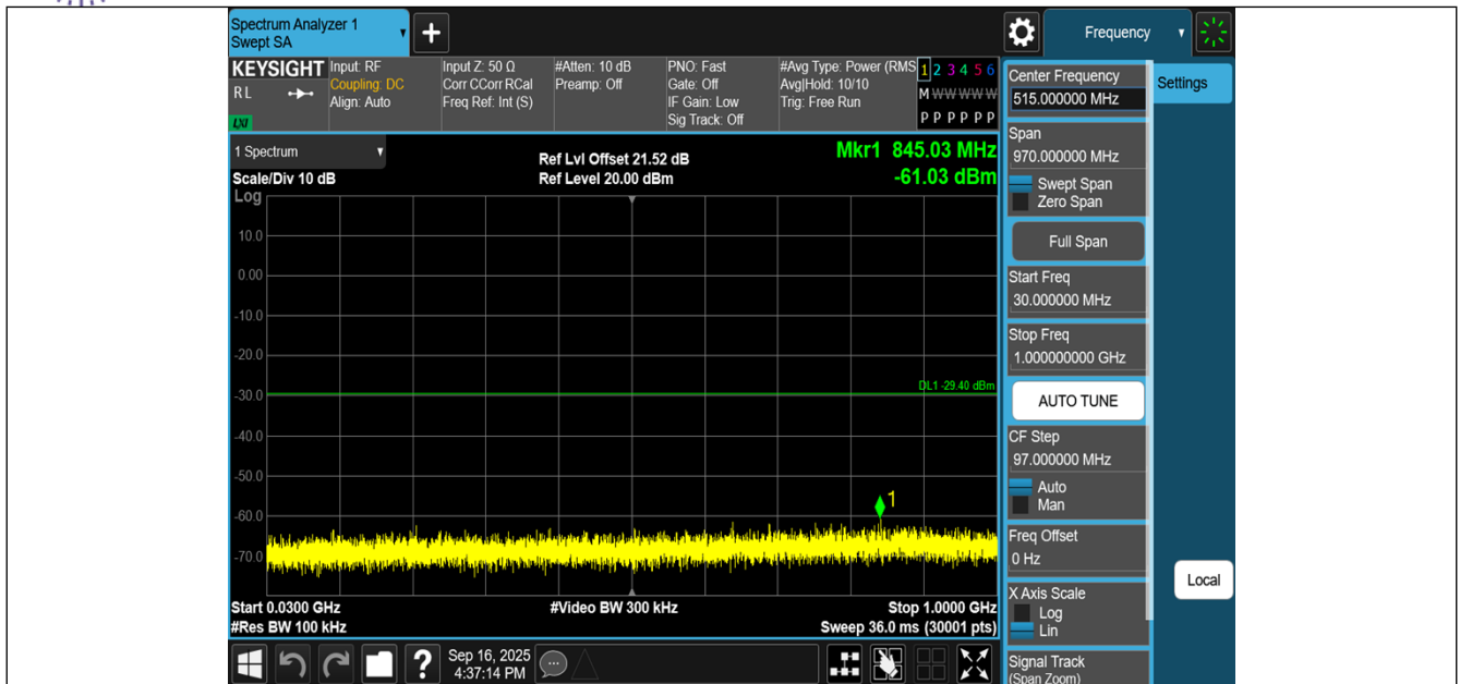
11AX20MIMO-Ant1-2437-30~1000-PASS
