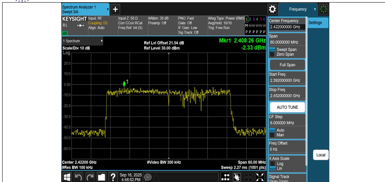
11AX40MIMO-Ant1-2422-0~Reference-PASS
