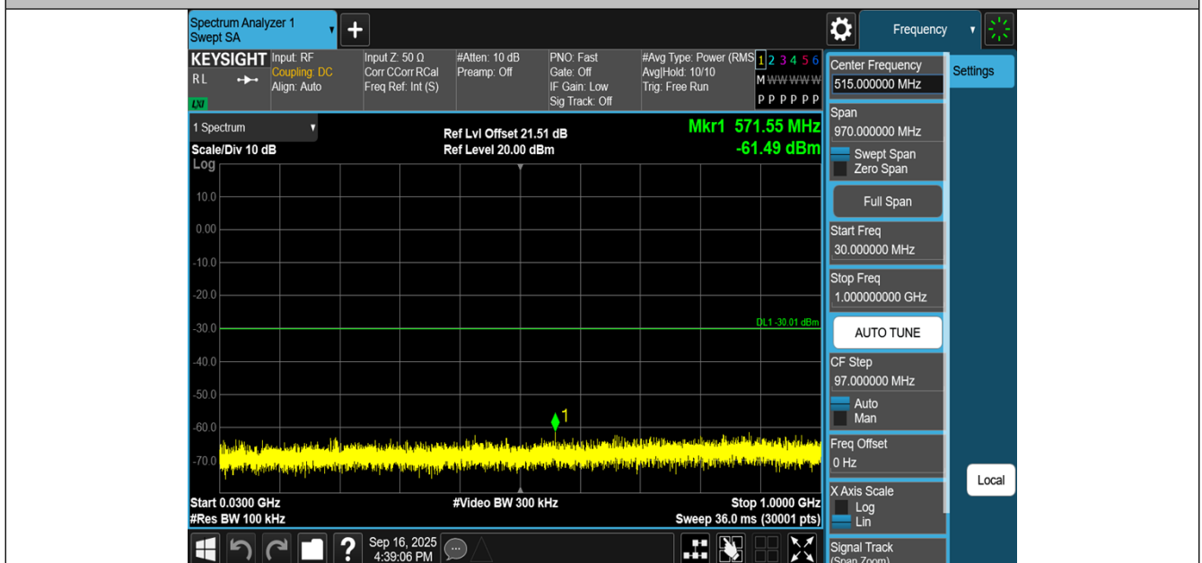
11AX20MIMO-Ant2-2437-30~1000-PASS
