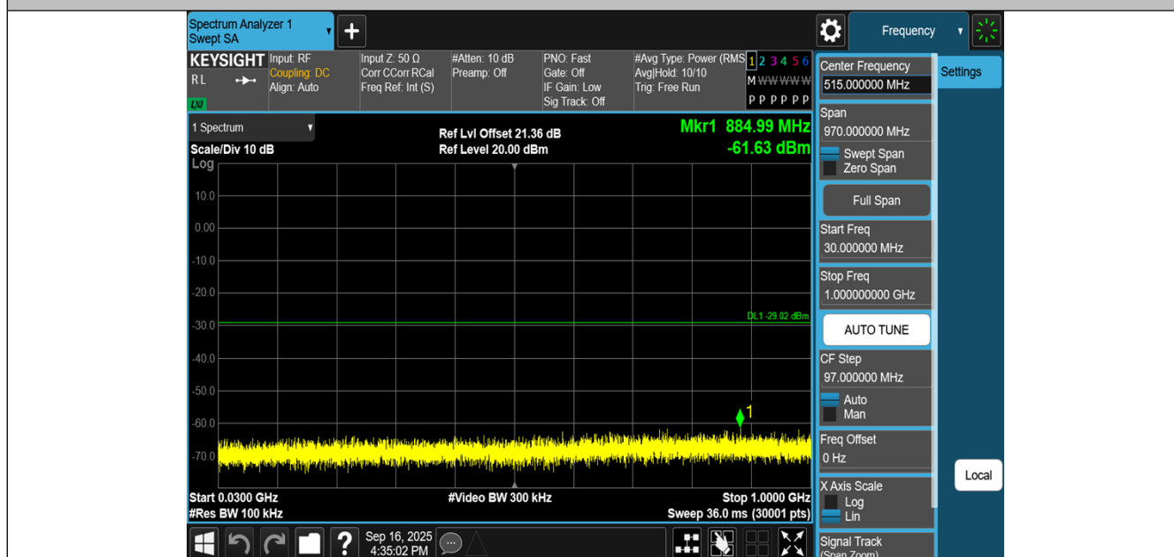
11AX20MIMO-Ant2-2412-30~1000-PASS
