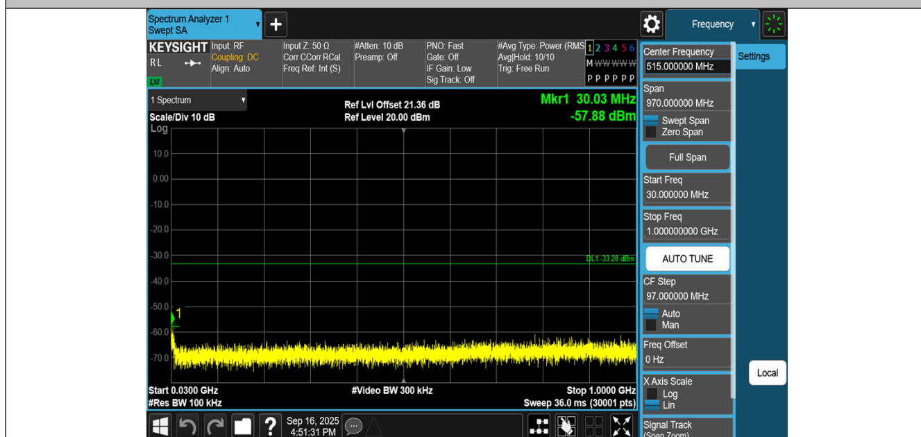
11AX40MIMO-Ant2-2422-30~1000-PASS
