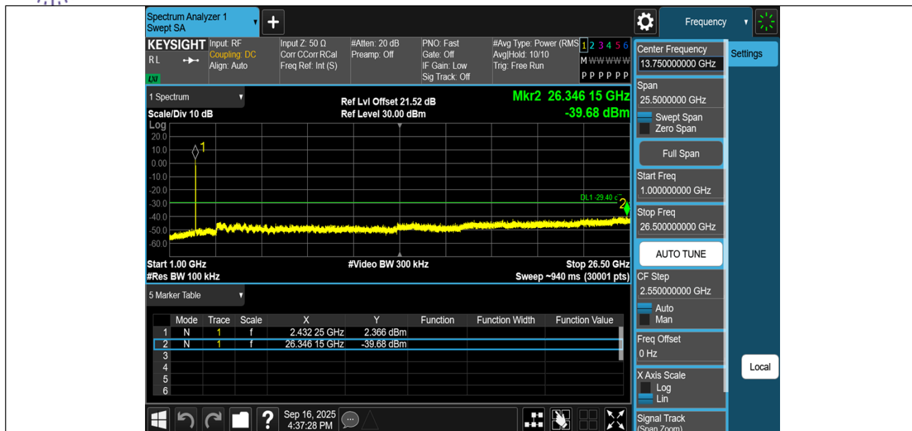
11AX20MIMO-Ant1-2437-1000~26500-PASS
