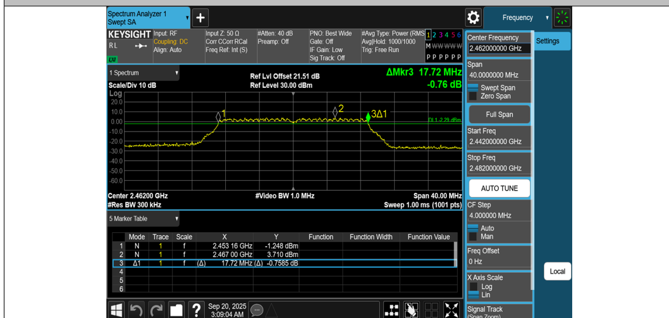
11N20MIMO-Ant2-2462-PASS
