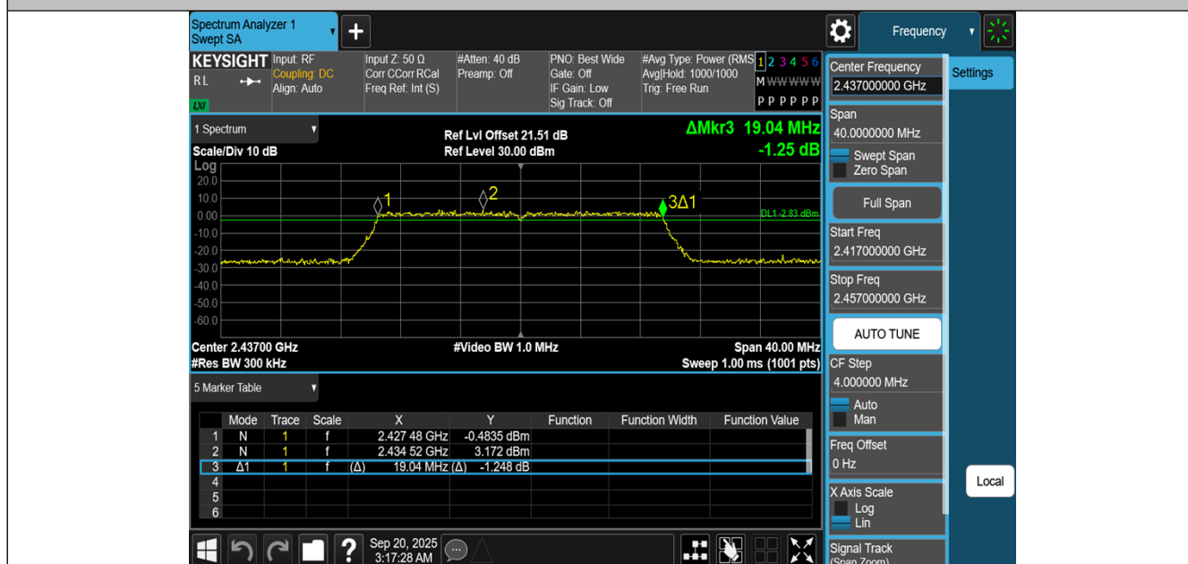
11AX20MIMO-Ant2-2437-PASS
