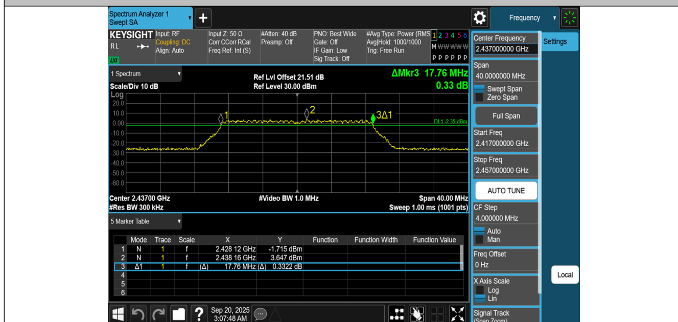
11N20MIMO-Ant2-2437-PASS
