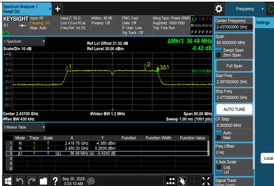
11N40MIMO-Ant1-2437-PASS
