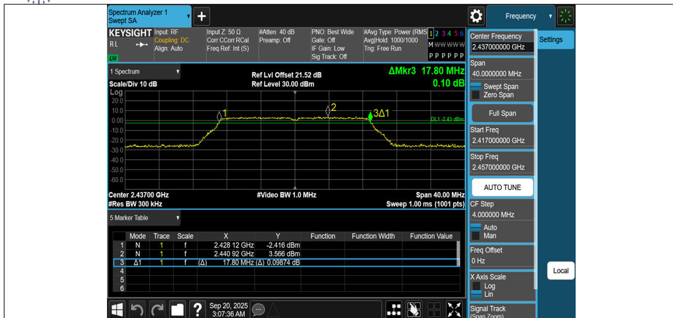
11N20MIMO-Ant1-2437-PASS
