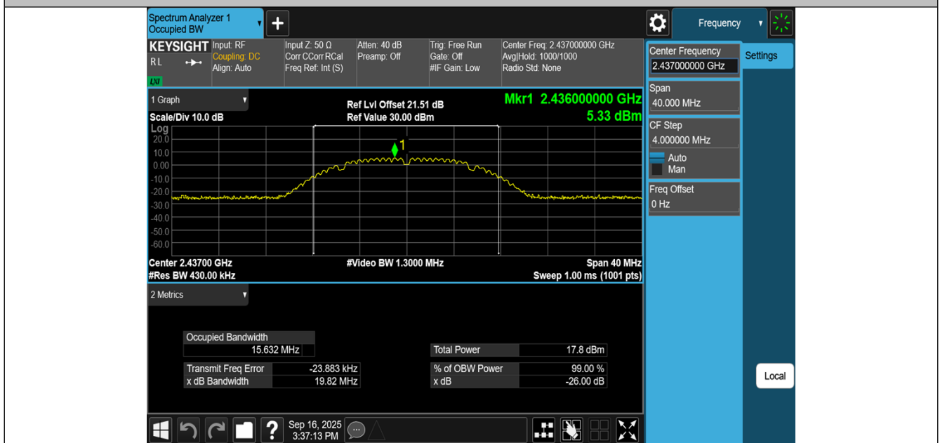
11B-Ant2-2437
