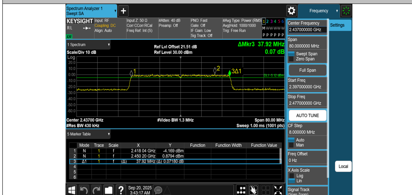
11AX40MIMO-Ant2-2437-PASS
