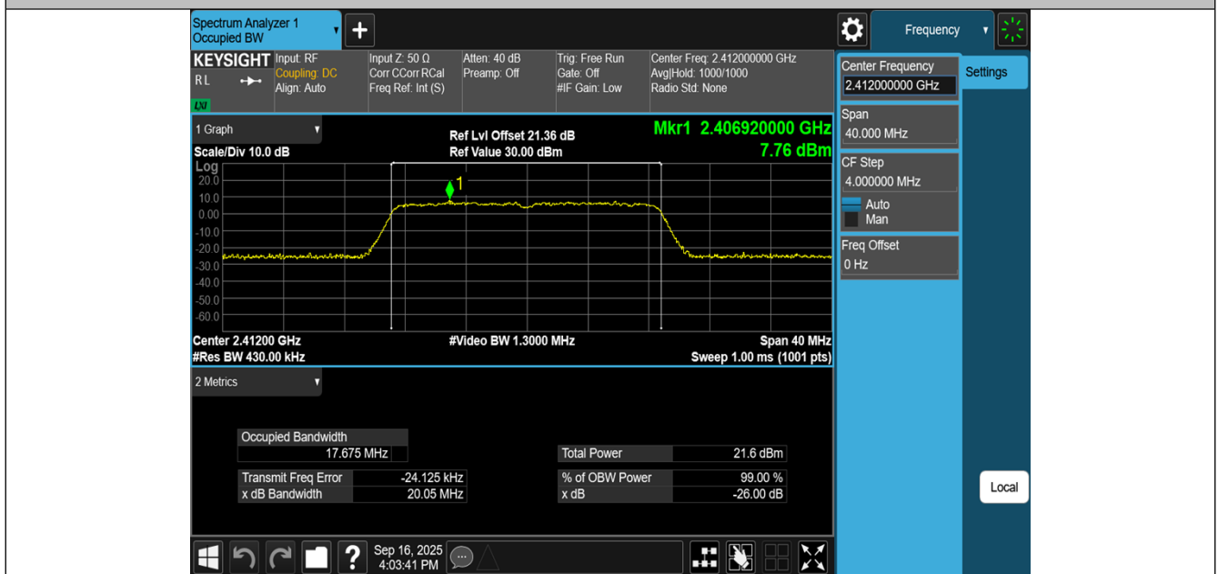
11N20MIMO-Ant2-2412
