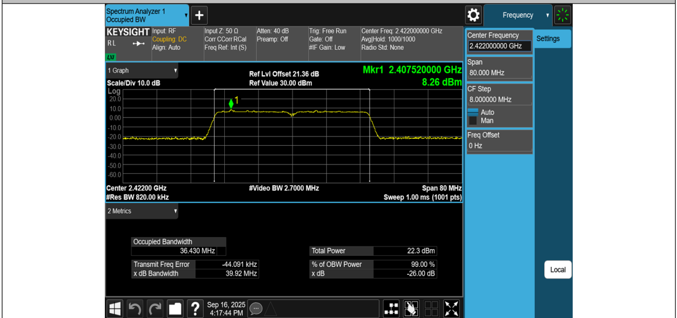
11N40MIMO-Ant2-2422
