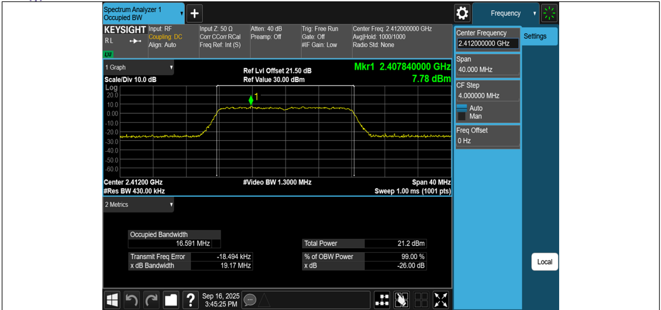
11G-Ant1-2412
