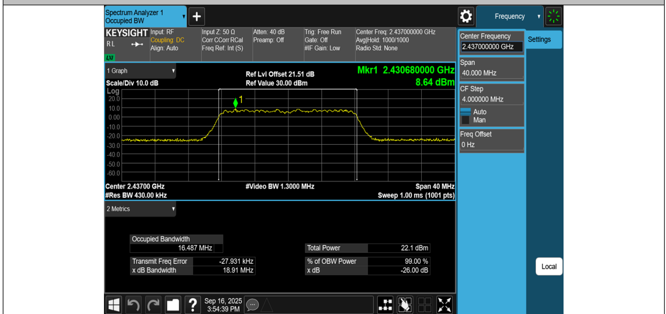
11G-Ant2-2437
