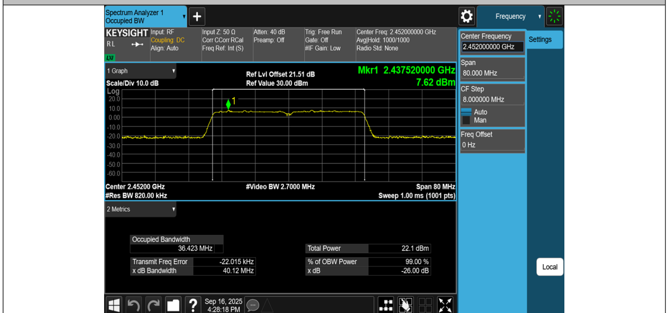
11N40MIMO-Ant2-2452
