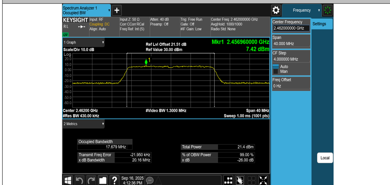
11N20MIMO-Ant2-2462
