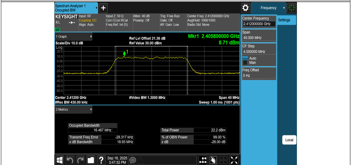
11G-Ant2-2412
