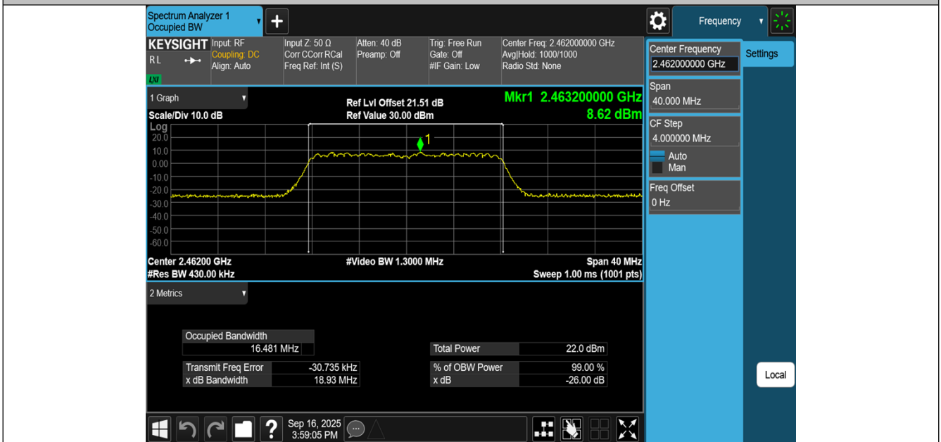
11G-Ant2-2462
