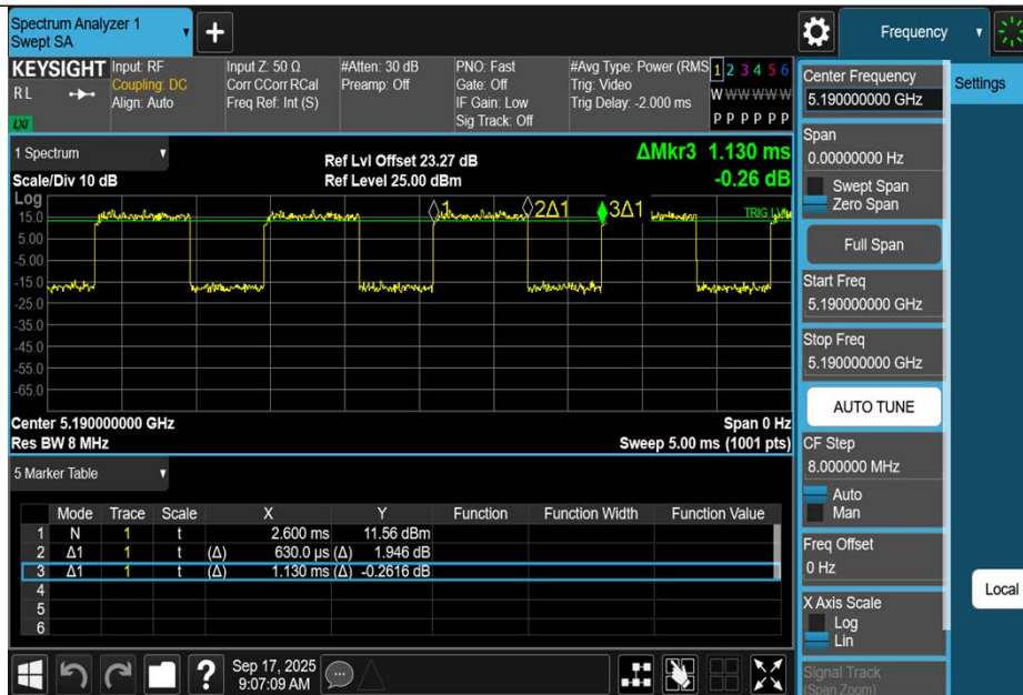
NTNV-11N40MIMO-5190
