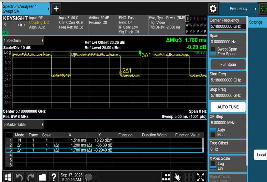
NTNV-11AC20MIMO-5180
